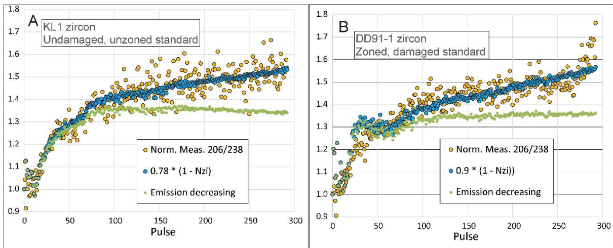
Fig 7: Signal profiles for 0.2 Hz analysis on standards KL (A) and DD91-1 (B). 206Pb/238U profiles (orange circles) normalized to estimates of instrument-biased true values compared to profiles of ablation deposits scaled by Pb depletion values chosen to maximize fit to ratio profiles (blue circles). Green dots are the same profiles assuming that ablated mass is proportional to area of the base of the pit with a final aspect ratio of 0.8
