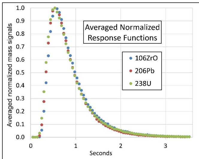
Fig 5. Averaged progressive single shot signal responses normalized to highest values for masses from KL.
