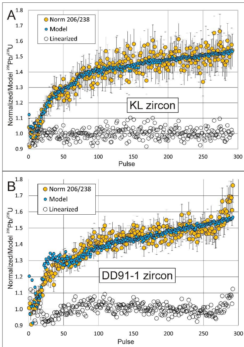
Fig 8: Normalized measured ^{206}\text{Pb}/^{238}\text{U} ratio profiles and modelling results from 0.2 Hz analyses of zircon KL-1 (A) and DD91-1 (B). Normalization factors, were taken from the mean of the first 10-12 data shown Fig 12. Pb loss is taken as constant at 0.78 for (A) and 0.9 for (B). Recycling is zero except for the first 10 pulses as explained in the text. Linearized data are explained in the text. Error bars represent 1 sigma estimates based on counts.
