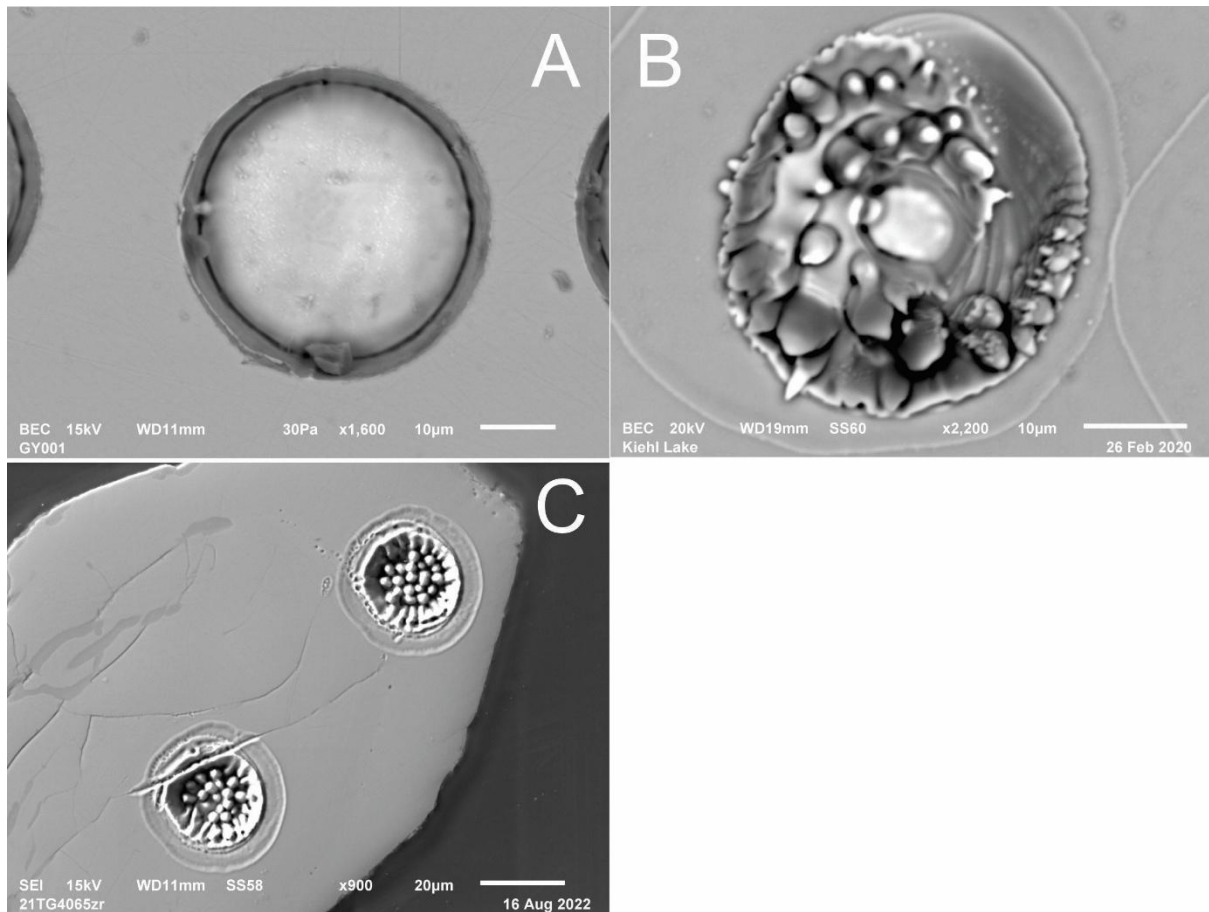
Fig. 2. SEM images intended to show that ablation pits in zircon contain a melt phase. (A) Electron backscatter image of laser ablation pit in KL zircon. (B) Same as A except that the laser beam was rotated once around a path half the radius of the pit. This shows that despite the flat surface seen at the base of the pit in A, the sample was melted. (C) Secondary electron image (SEI) of ablation pits in high-U Archean zircon that is much more damaged than KL. Irregular solidified melt is seen along the walls and base of the pits.
