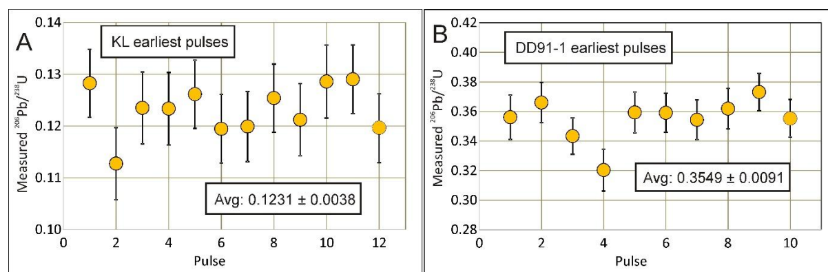
Fig 9: Averages of earliest ratios from KL (A) and DD91-1 (B). Errors represent 2 sigma.
