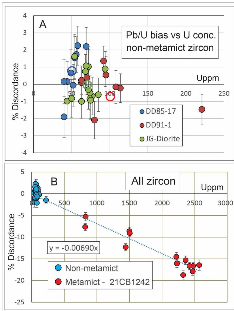
Fig 12: Results of UTILAZ data reduction on zircon with variable ages, U concentrations and radiation damage. Error bars represent 2 sigma. KL was used as the standard. (A) Data from non-metamict zircon. Open symbols represent averages. (B) Data from metamict zircon U (>500 ppm) show a roughly linear relationship between U concentration and negative discordance. The regression line is forced through the origin.
