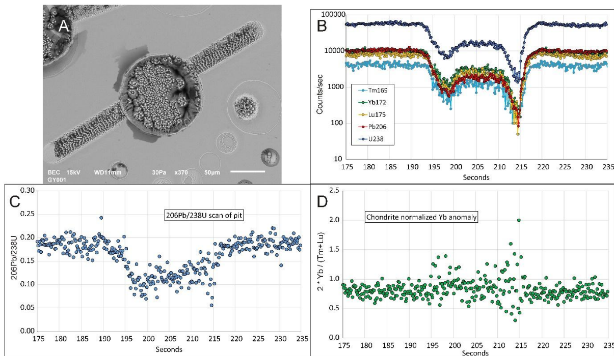
Fig. 3. (A) 130 micron pit floored by an irregular solidified melt layer crossed by a 30 µm scan line. (B) Trace element signals from the scan. (C) ^{206}\text{Pb}/^{238}\text{U} ratios show a depletion of Pb relative to U across the bottom of the pit. (D) ^{172}\text{Yb} signal shows no clear anomaly relative to the average of less volatile ^{169}\text{Tm} and ^{175}\text{Lu} above and below it, indicating that Yb is insufficiently volatile to act as a proxy for Pb during ablation.
