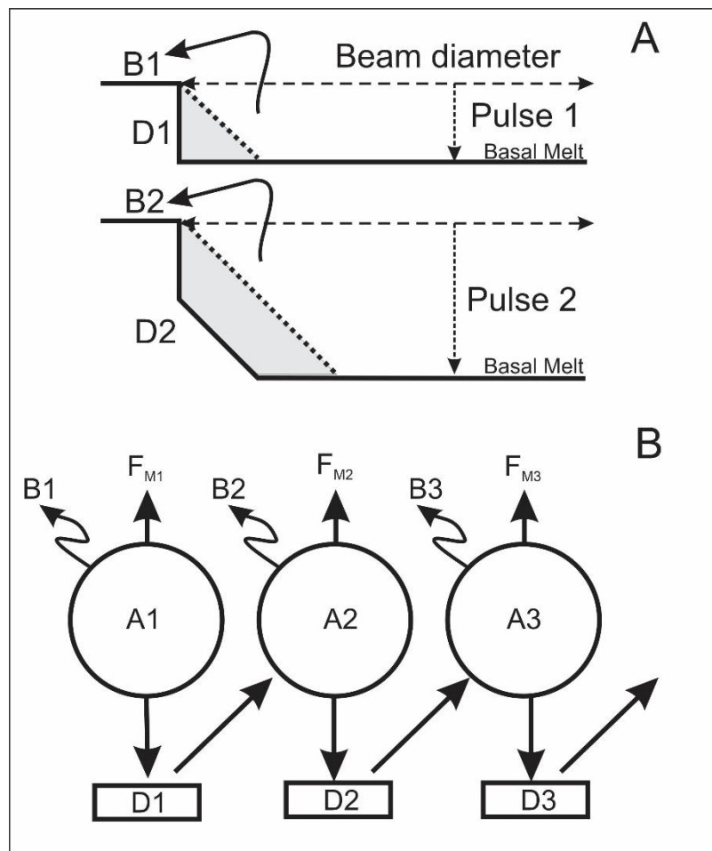
Fig. 4 (A) Schematic illustration of the model showing the effect of the first two laser pulses on a zircon sample as seen from the edge of a cross section of an ablation pit. D is the depth excavated per laser pulse. Pb-depleted ablated material (melt) deposited in the pit is shown in grey. The second pulse is assumed to re-ablate the residue left from the first but this consumes energy at the edge of the beam, causing the pit to taper with depth. (B) Effects of the first laser pulses on measured composition. The first ablation cloud ( A1 ) leaves a Pb-depleted deposit in the pit ( D1 ) and fallback ( B1 ), which increases its Pb/U ratio. The second pulse can re-evaporate D1 plus pristine material, leaving a second Pb-depleted deposit ( D2 ) as well as
