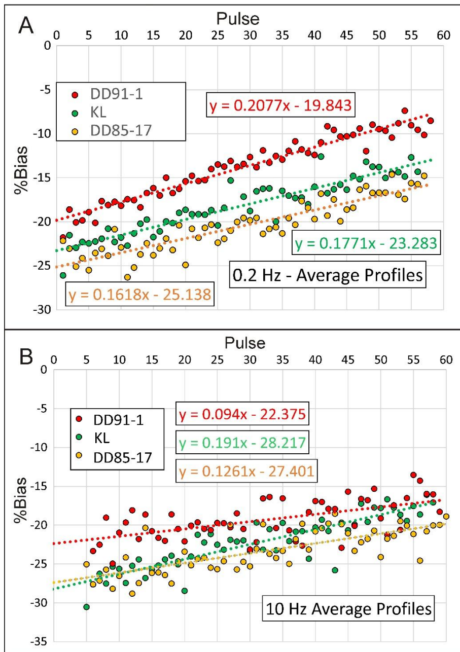
525 Fig. 10 Percent difference between the measured and true ^{206}\text{Pb}/^{238}\text{U} ratios of three zircon standards for data acquired at (A) 0.2 Hz and (B) 10 Hz. Each set of symbols represents an average of analyses on 4 spots. Analyses shown in A and B were carried out during different sessions with different instrument bias.
