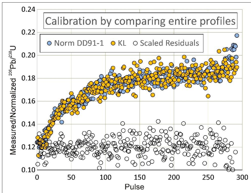
Fig 11: Comparison of measured KL ratio profile (taken as the standard) with measured DD91-1 profile (taken as the unknown) normalized to minimize the sum of squares of differences between corresponding data points (residuals). These are scaled so they are visible on the plot. The residual for two overlapping data would plot on the 0.12 line. Omitting the last 30 data, a normalization factor of 2.868 gives the minimum sum of residuals. The inferred ^{206}\text{Pb}/^{238}\text{U} value is 0.15% different from the accepted ratio.
