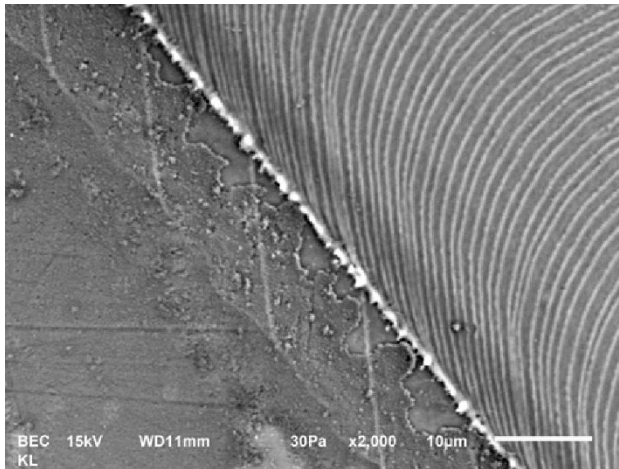
120 Figure 1: BSE high contrast image showing one side of a laser scan of KL. Bright fragments of melt are seen concentrated along the edge of the scan and ejected from it. These may be deleted in Pb relative to U contributing to a positive ^{206}\text{Pb}/^{238}\text{U} measurement bias.
