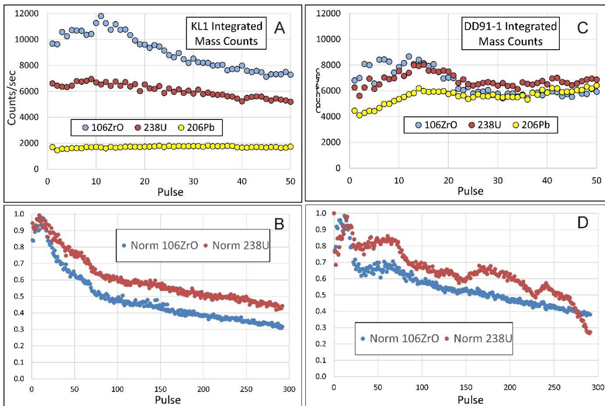
Fig 5. Averaged progressive single shot signal responses normalized to highest values for masses from KL.
