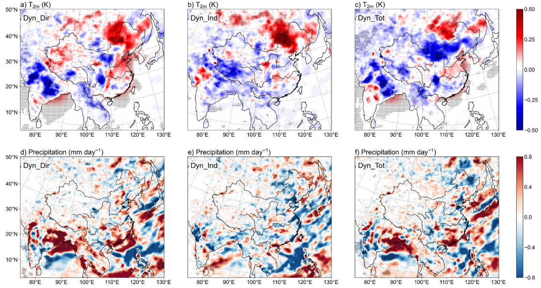
Figure 10. Changes in the surface air temperature at 2 m ( T_{2m} ) (a–c, K) and precipitation (d–f, mm day −1 ) over East Asia in summer during 2008–2021 in the Dyn_Dir (left), Dyn_Ind (center) and Dyn_Tot (right) experiments. Black-dotted regions denote statistically significant differences at the 90% confidence level based on a two-sided paired Student’s t -test.
