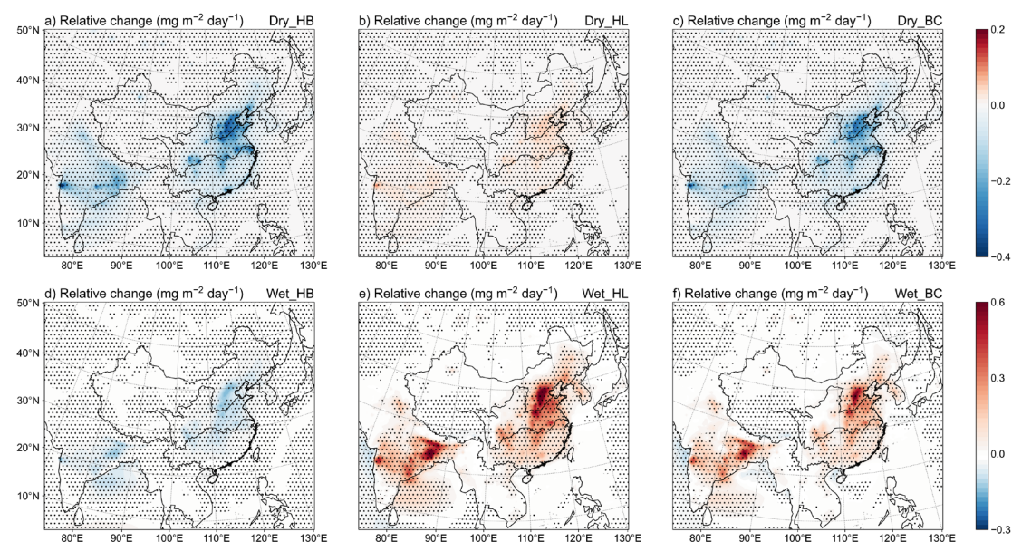
Figure 4. Relative changes in the dry deposition flux (a–c, \text{mg m}^{-2} \text{ day}^{-1} ) and wet deposition flux (d–f, \text{mg m}^{-2} \text{ day}^{-1} ) of hydrophobic BC (HB, left), hydrophilic BC (HL, center) and total BC (BC, right) over East Asia in summer during 2008–2021 between the Exp. 8 and Exp. 4. Black-dotted regions denote statistically significant differences at the 90% confidence level based on a two-side paired Student's t -test.
