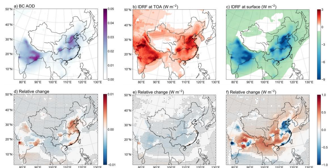
Figure 5. Spatial distributions of the BC aerosol optical depth (AOD) (a), instantaneous direct radiative forcing (IDRF) at the TOA and surface (b and c, \text{W m}^{-2} ) over East Asia in summer during 2008–2021 in the Dyn_Dir experiment. Relative changes in the BC AOD (d), IDRF at the TOA and surface (e and f, \text{W m}^{-2} ) over East Asia in summer during 2008–2021 between the Dyn_Dir and Def_Dir experiments. Black-dotted regions denote statistically significant differences at the 90% confidence level based on a two-sided paired Student's t -test.
