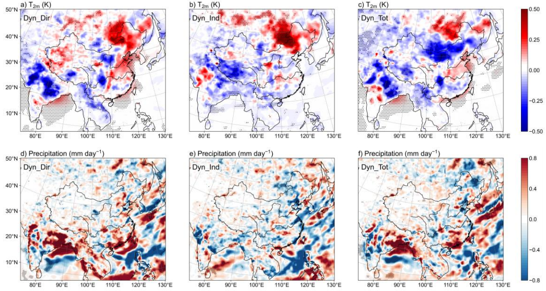
Figure 10. Changes in the surface air temperature at 2 m ( T_{2m} ) (a–c, K) and precipitation (d–f, mm day −1 ) over East AsiaChina in summer during 2008–2021 in the Dyn_Dir (left), Dyn_Ind (center) and Dyn_Tot (right) experiments. Black-dotted regions denote statistically significant differences at the 90% confidence level based on a two-sided paired Student’s t -test.
