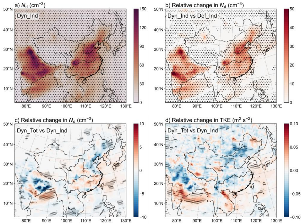
Figure 7. Changes in the cloud droplet number concentration ( N_d ) (a, \text{cm}^{-3} ) near 850 hPa from the BC–cloud interaction over East China in summer during 2008–2021 in the Dyn_Ind experiment. Relative changes in the N_d (b, \text{cm}^{-3} ) near 850 hPa from the BC–cloud interaction over East China in summer during 2008–2021 between the Dyn_Ind and Def_Ind experiments. Relative changes in the N_d (c, \text{cm}^{-3} ) and TKE (d, \text{m}^2 \text{s}^{-2} ) near 850 hPa from the BC–cloud interaction over East China in summer during 2008–2021 between the Dyn_Tot and Dyn_Ind experiments. Black-dotted regions denote statistically significant differences at the 90% confidence level based on a two-sided paired Student’s t -test.
