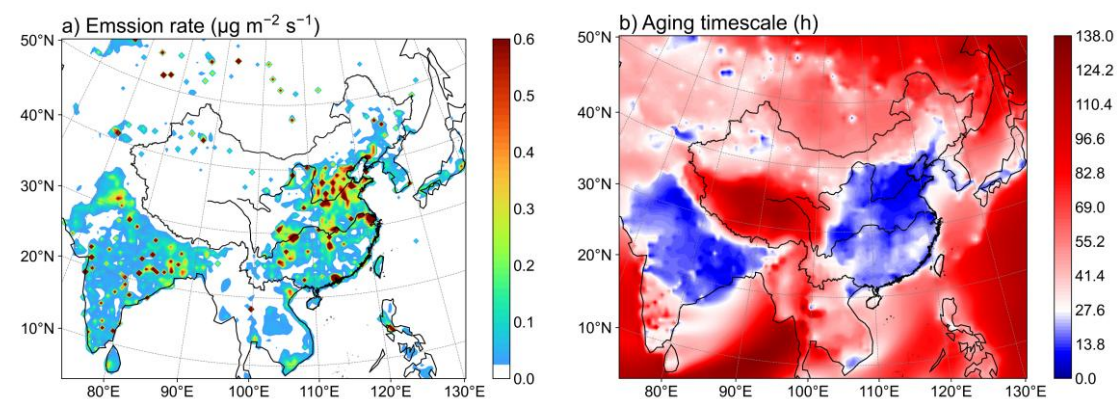
Figure 2. Spatial distributions of the aerosol precursor ( \text{SO}_2 + \text{OC} + \text{BC} ) emission rate (a, \mu\text{g m}^{-2} \text{s}^{-1} ) and BC aging timescale (b, h) over East Asia in summer during 2008–2021 in the Exp. 8.
