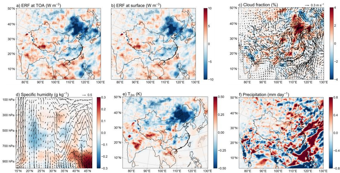
Figure 11. Spatial distributions of the nonlinear interaction term under the dynamic aging scheme (Dyn_I) for the BC effective radiative forcing (ERF) at TOA and surface (a and b, \text{W m}^{-2} ), wind field (arrow, \text{m s}^{-1} ) and cloud fraction (shaded, %) (c) near 850 hPa, meridional circulation (arrow) and specific humidity (shaded, \text{g kg}^{-1} ) (d) in the altitude–latitude section averaged from 112° to 122°E, surface temperature at 2 m ( T_{2m} ) (e, K) and precipitation (f, \text{mm day}^{-1} ) over East Asia in summer during 2008–2021. Black-dotted regions denote statistically significant differences at the 90% confidence level based on a two-sided paired Student's t -test.
