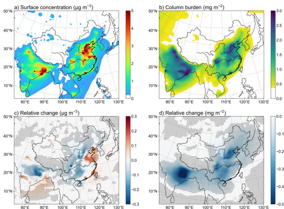
Figure 3. Spatial distributions of the BC surface concentration (a, \mu\text{g m}^{-3} ) and column burden (b, \text{mg m}^{-2} ) over East Asia in summer during 2008–2021 in the Exp. 8. Relative changes in the BC surface concentration (c, \mu\text{g m}^{-3} ) and column burden (d, \text{mg m}^{-2} ) over East Asia in summer during 2008–2021 between the Exp. 8 and Exp. 4. Black-dotted regions denote statistically significant differences at the 90% confidence level based on a two-sided paired Student's t -test.
