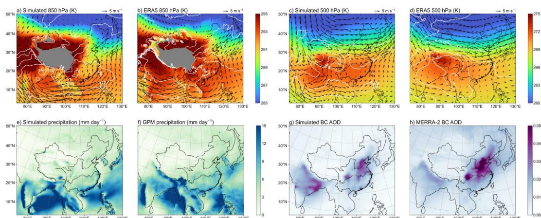
Figure 1. Comparisons between RegCM-Chem summer outputs in the Exp. 8 and multiple reference datasets, including air temperature (shaded, K), specific humidity (contours, \text{g kg}^{-1} ), wind (vectors, \text{m s}^{-1} ) at 850 hPa (a and b) and 500 hPa (c and d), precipitation (e and f, \text{mm day}^{-1} ) and BC aerosol optical depth (AOD) (g and h)
