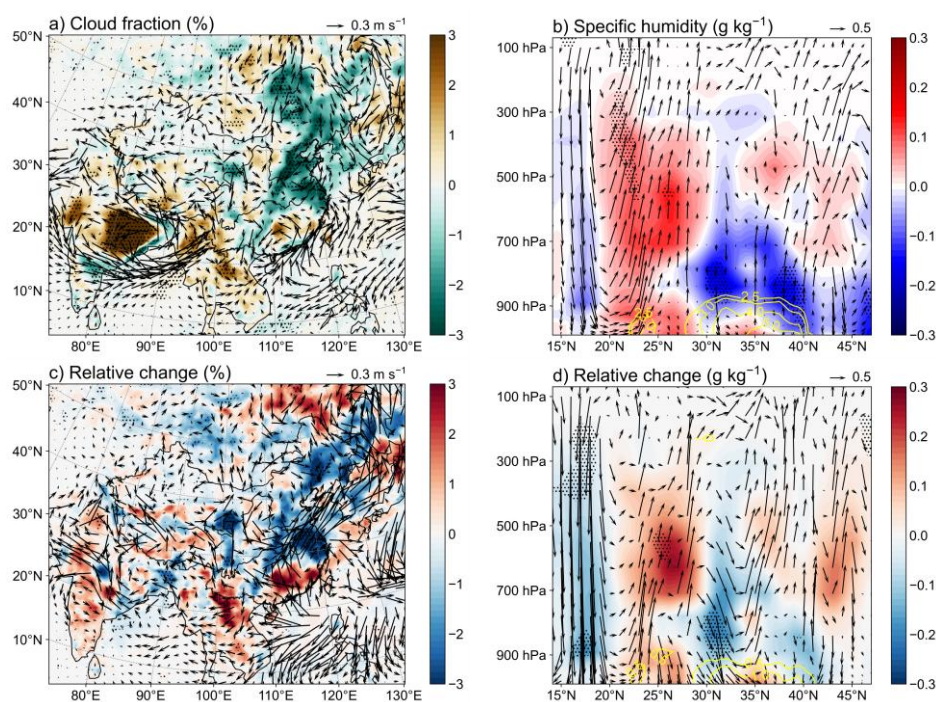
Figure 6. Changes in the wind field (arrow, \text{m s}^{-1} ) and cloud fraction (shaded, %) (a) near 850 hPa,
