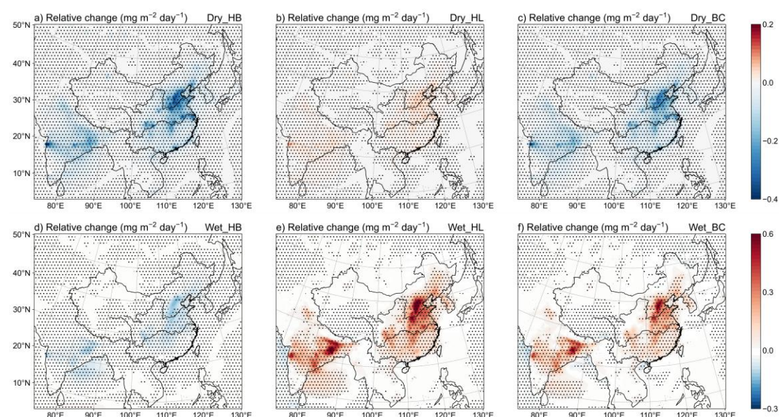
Figure 4. Relative changes in the dry deposition flux (a–c, \text{mg m}^{-2} \text{day}^{-1} ) and wet deposition flux (d–f, \text{mg m}^{-2} \text{day}^{-1} ) of hydrophobic BC (HB, left), hydrophilic BC (HL, center) and total BC (BC, right) over East Asia in summer during 2008–2021 between the Exp. 8 and Exp. 4. Black-dotted regions denote statistically significant differences at the 90% confidence level based on a two-side paired Student's t -test.
