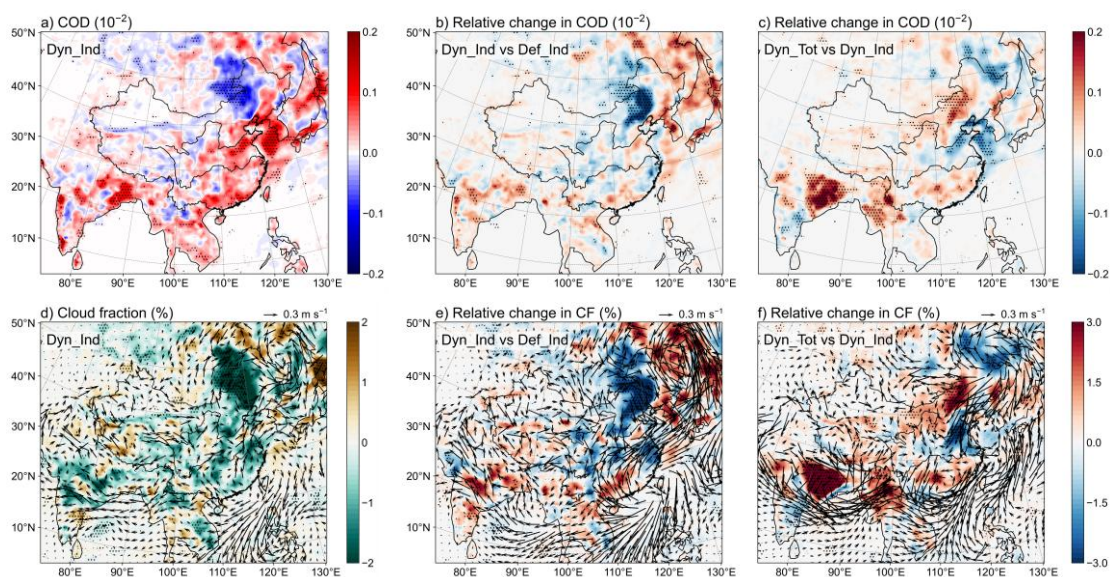
Figure 8. Changes in the cloud optical depth (COD) (a) and cloud fraction (CF) (d, %) near 850 hPa from the BC–cloud interaction over East China in summer during 2008–2021 in the Dyn_Ind experiment. Relative changes in COD (b) and CF (e, %) near 850 hPa from the BC–cloud interaction over East China in summer during 2008–2021 between the Dyn_Ind and Def_Ind experiments. Relative changes in the COD (c) and CF (f, %) near 850 hPa from the BC–cloud interaction over East China in summer during 2008–2021 between the Dyn_Tot and Dyn_Ind experiments. Black-dotted regions denote statistically significant differences at the 90% confidence level based on a two-sided paired Student’s t -test.
