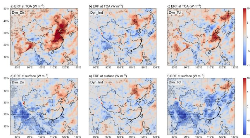
Figure 9. Spatial distributions of the BC effective radiative forcing (ERF) at the TOA and surface (a–c and d–f, \text{W m}^{-2} ) over East Asia in summer during 2008–2021 in the Dyn_Dir (left), Dyn_Ind (center) and Dyn_Tot (right) experiments. Black-dotted regions denote statistically significant differences at the 90% confidence level based on a two-sided paired Student's t -test.
