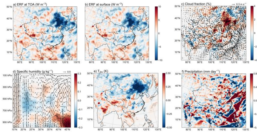
Figure 11. Spatial distributions of the nonlinear interaction term under the dynamic aging scheme (Dyn_I) for the BC effective radiative forcing (ERF) at TOA and surface (a and b, \text{W m}^{-2} ), wind field (arrow, \text{m s}^{-1} ) and cloud fraction (shaded, %) (c) near 850 hPa, meridional circulation (arrow) and specific humidity (shaded, \text{g kg}^{-1} ) (d) in the altitude–latitude section averaged from 112^\circ to 122^\circ\text{E} , surface temperature at 2 m ( T_{2m} ) (e, K) and precipitation (f, \text{mm day}^{-1} ) over East Asia in summer during 2008–2021. Black-dotted regions denote statistically significant
