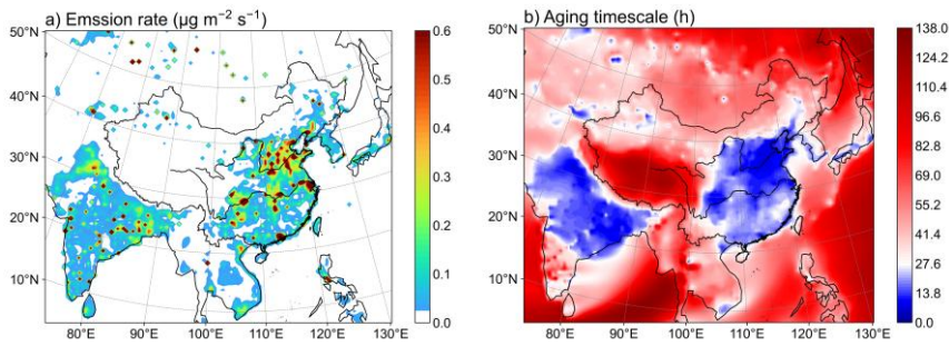
Figure 2. Spatial distributions of the aerosol precursor ( \text{SO}_2 + \text{OC} + \text{BC} ) emission rate (a, \mu\text{g m}^{-2} \text{s}^{-1} ) and BC aging timescale (b, h) over East Asia in summer during 2008–2021 in the Exp. 8.
