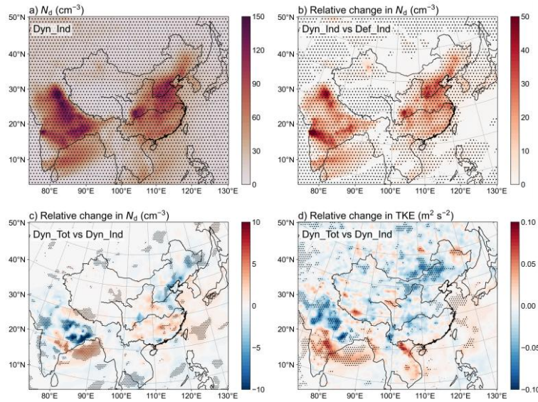
Figure 7. Changes in the cloud droplet number concentration ( N_d ) (a, \text{cm}^{-3} ) near 850 hPa from the BC–cloud interaction over East China in summer during 2008–2021 10 in the Dyn_Ind experiment. Relative changes in the N_d (b, \text{cm}^{-3} ) near 850 hPa from the BC–cloud interaction over East China in summer during 2008–2021 10 between the Dyn_Ind and Def_Ind experiments. Relative changes in the N_d (c, \text{cm}^{-3} ) and TKE (d, \text{m}^2 \text{s}^{-2} ) near 850 hPa from the BC–cloud interaction over East China in summer during 2008–2021 10 between the Dyn_Tot and Dyn_Ind experiments. Black-dotted regions denote statistically significant differences at the 90% confidence level based on a two-sided paired Student’s t -test .
