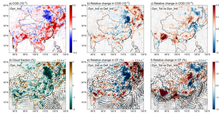
Figure 8. Changes in the cloud optical depth (COD) (a) and cloud fraction (CF) (d-f, %) near 850 hPa from the BC–cloud interaction over East China in summer during 2008–2021 in the Dyn_Ind experiment. Relative changes in COD (b) and CF (e, %) near 850 hPa from the BC–cloud interaction over East China in summer during 2008–2021 between the Dyn_Ind and Def_Ind experiments. Relative changes in the COD (c) and CF (f, %) near 850 hPa from the BC–cloud interaction over East China in summer during 2008–2021 between the Dyn_Tot and Dyn_Ind experiments. Black-dotted regions denote statistically significant differences at the 90% confidence level based on a two-sided paired Student’s t -test .
