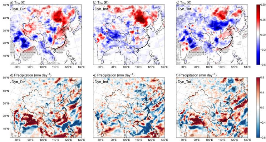
Figure 10. Changes in the surface air temperature at 2 m ( T_{2m} ) (a–c, K) and precipitation (d–f, mm day -1 ) over East China in summer during 2008–2021 in the Dyn_Dir (left), Dyn_Ind (center) and Dyn_Tot (right) experiments. Black-dotted regions denote statistically significant differences at the 90% confidence level based on a two-sided paired Student’s t -test.
