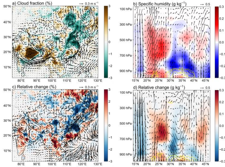
Figure 6. Changes in the wind field (arrow, \text{m s}^{-1} ) and cloud fraction (shaded, %) (a) near 850 hPa, meridional circulation (arrow), specific humidity (shaded, \text{g kg}^{-1} ) and shortwave heating rate (contour, 10^{-6} \text{ K s}^{-1} ) (b) in the altitude–latitude section averaged from 112^\circ to 122^\circ\text{E} from the BC–radiation interaction over East China in summer during 2008–2021 9 in the Dyn_Dir experiment. Relative changes in the wind field (arrow, \text{m s}^{-1} ) and cloud fraction (shaded, %) (c) near 850 hPa, meridional circulation (arrow), specific humidity (shaded, \text{g kg}^{-1} ) and shortwave heating rate (contour, 10^{-6} \text{ K s}^{-1} ) (d) in the altitude–latitude section averaged from 112^\circ to 122^\circ\text{E} from the BC–radiation interaction over East China in summer during 2008–2021 9 between the Dyn_Dir and Def_Dir experiments. Black-dotted regions denote statistically significant differences at the 90% confidence level based on a two-sided paired Student’s t -test .
