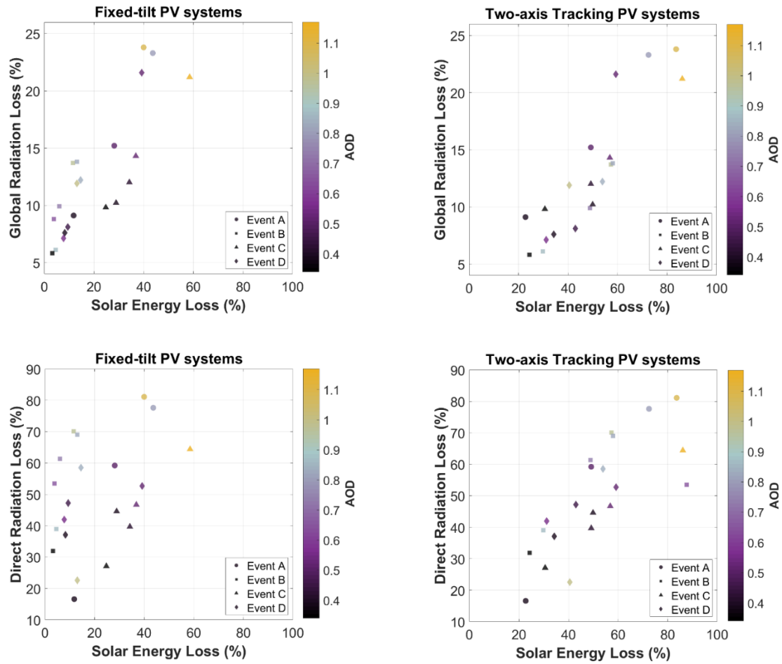
Figure 5: Global (top panel) and direct (lower panel) radiation losses (%) versus losses in produced PV solar energy (in %) during the four dust events for fixed-tilt PV systems (left) and two-axis tracking systems (right), along with AOD.
