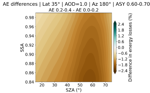
Figure 8: Differences in PV energy losses (%) as a function of solar zenith angle (SZA) and single-scattering albedo (SSA) for the Ångström exponent sensitivity analysis, under fixed latitude ( 35^\circ ), aerosol optical depth ( \text{AOD} = 1.0 ), south-facing orientation ( \text{Az} = 180^\circ ), and asymmetry parameter range \text{ASY} = 0.60\text{--}0.70 . The panel shows the difference in losses between the AE intervals 0.2–0.4 and 0.0–0.2.
