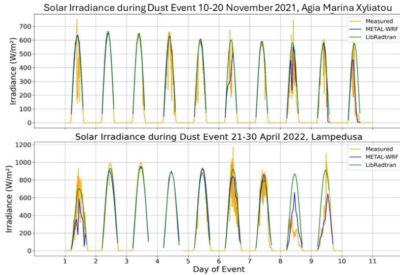
505 Figure 10: Timeseries of the GHI at Agia Marina Xyliatou, Cyprus, during event C (upper panel) and Lampedusa, Italy, during Event D (lower panel). In the case of AMX, during days 2, 3, 5 and 7 clear-sky conditions dominated, while in the case of Lampedusa, days 1, 6, 7, 8 and 9 indicated cloudy conditions.
