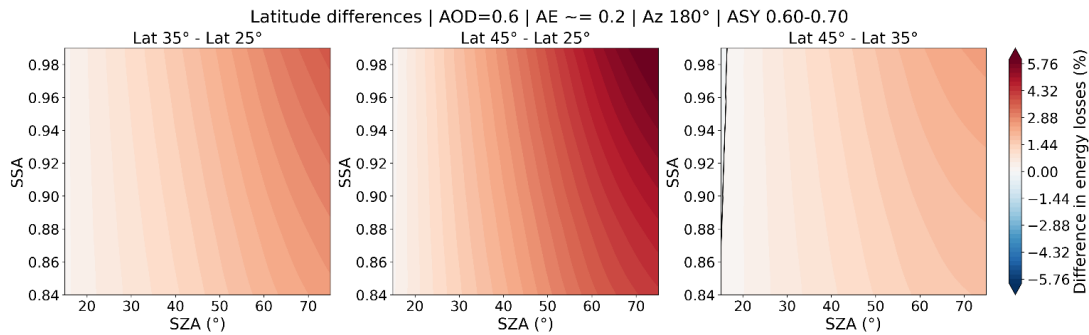
Figure 6: Differences in PV energy losses (%) as a function of solar zenith angle (SZA) and single-scattering albedo (SSA) for the latitude sensitivity analysis, under fixed aerosol optical depth (AOD = 0.6), Ångström exponent (AE ≈ 0.2), south-facing orientation (Az = 180°), and asymmetry parameter range ASY = 0.60–0.70.
