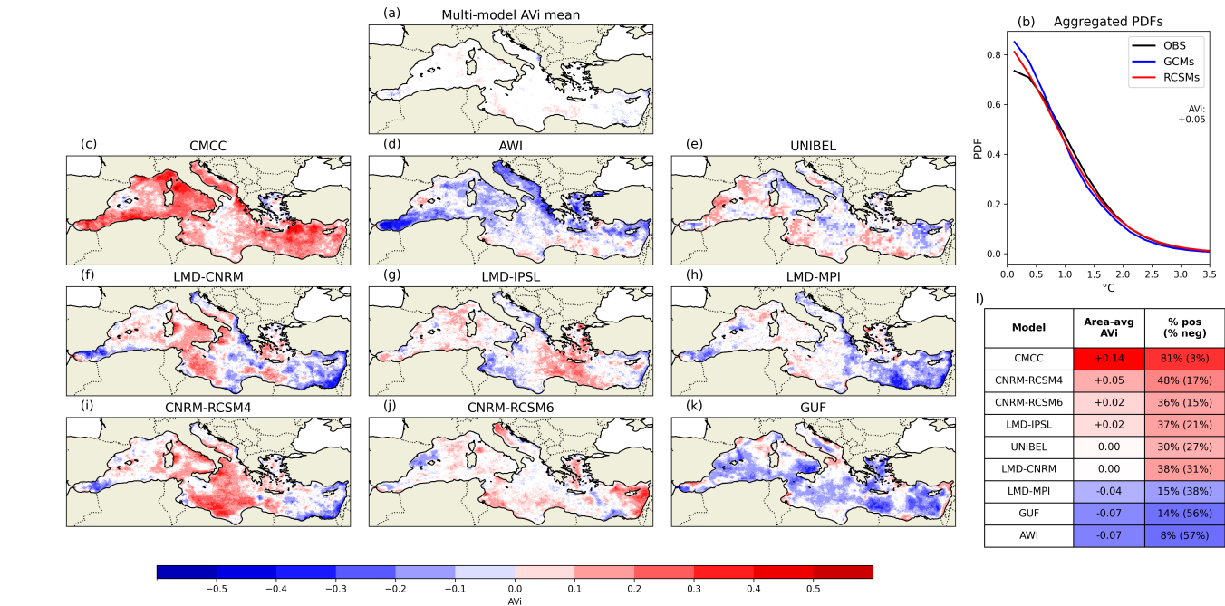
Figure 3. As in Fig. 2 but for the SST upper tail distribution (SSTs above the 90th percentile) in 1982-2020. Regarding warm SSTs (above the 90th percentile), the multi-model mean (Fig. 3a) highlights small common areas of improvements in the central Mediterranean, Tyrrhenian Sea, and Ligurian Sea, with negative values confined to the far eastern and western margins of the basin. Individual models exhibit substantially different spatial patterns of added and lost value (Fig. 225
