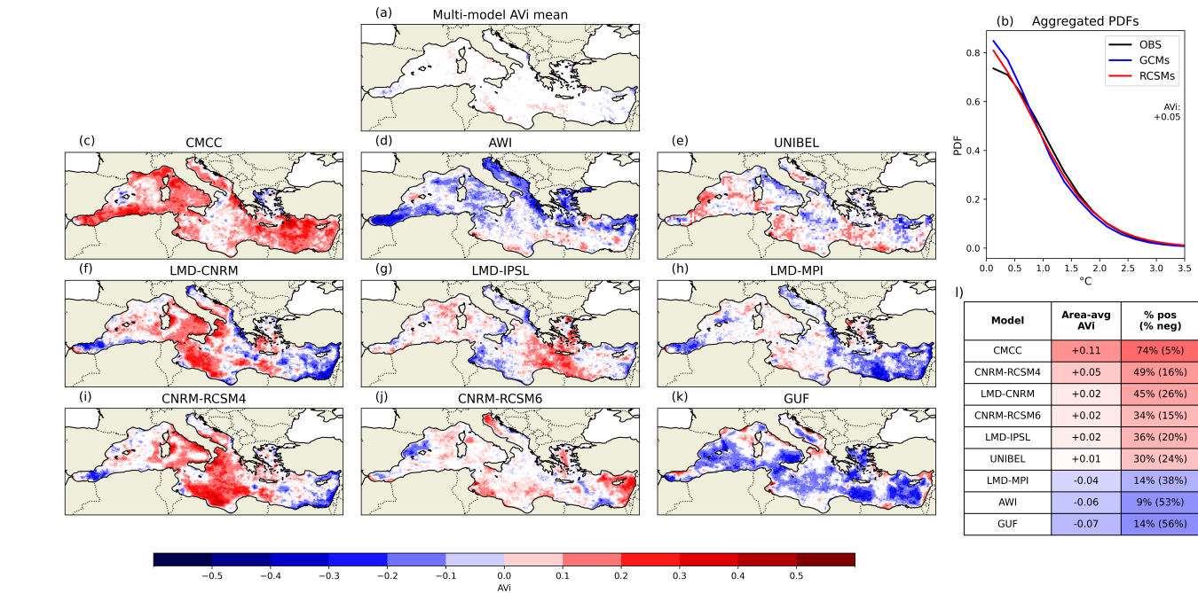
Figure 3. As in Fig. 2 but for the SST upper tail distribution (SSTs above the 90th percentile) in 1982-2020.
