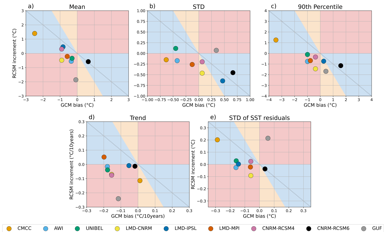
Figure 1. RCSM increment versus GCM bias for area-averaged SST (a) mean, (b) STD, (c) 90th percentile, (d) trend, (e) STD of SST residuals over 1982–2020. The green grey line indicates perfect error correction. Green Blue , red, and orange shading denote skillful error reduction, deterioration, and overcompensation (RCSM error opposite in sign but larger in magnitude than the GCM error), respectively. For the definition of the Mediterranean domain see Fig. 2.
