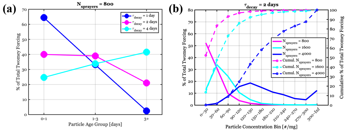
Figure 11. (a) The percent of Twomey forcing as a function of particle age for N_{\text{sprayers}} = 800 and \tau_{\text{decay}} of 1, 2, and 4 days. (b) The percent of Twomey forcing from each particle concentration bin for \tau_{\text{decay}} = 2 days. Bold lines represent the LES ensemble mean percentage of total Twomey forcing (left y-axis) and the dashed lines correspond to the cumulative percentage of Twomey forcing going from left to right in the bin space (right y-axis). Different colors are for different values of N_{\text{sprayers}} .
