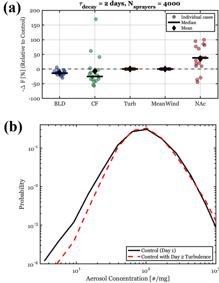
Figure 8. (a) Twomey forcing susceptibility -sensitivity analysis for \tau_{decay} = 2 days and N_{sprayers} = 4000 , where BLD is the boundary layer depth, CF is the cloud fraction/cloud reflectance, Turb is the particle model turbulence forcing that controls the spreading rate, which includes the C_0 changes related to precipitation, MeanWind is the mean wind, and NA_c is the background aerosol concentration. Positive percentages indicate that Day 2 values of a given variable act to increase Twomey forcing relative to Day 1 values. The circles represent each LPM simulation, the diamond is the ensemble mean, and the line is the ensemble median. (b) Average aerosol concentration probability distributions across all cases at local noon for the Control (Day 1 regime) and the Control run using Day 2 turbulence forcing in the particle model.
