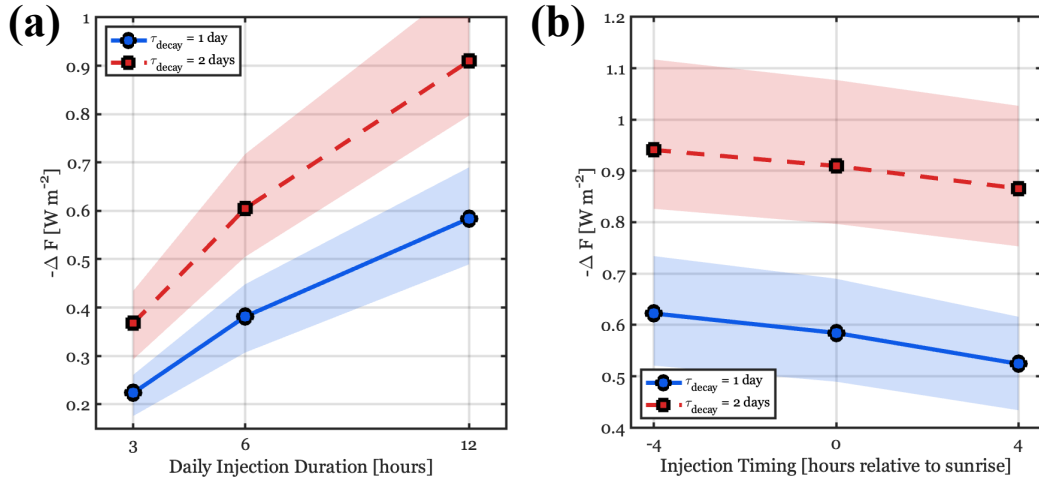
Figure 10. Global Ensemble-averaged global mean Twomey forcing as a function of (a) the daily injection duration for \tau_{\text{decay}} of 1 and 2 days and (b) the injection timing relative to sunrise, for a 12-hour daily injection. Shading corresponds to the IQR of the ensemble. Sensitivity tests use N_{\text{sprayers}} = 4000 .
