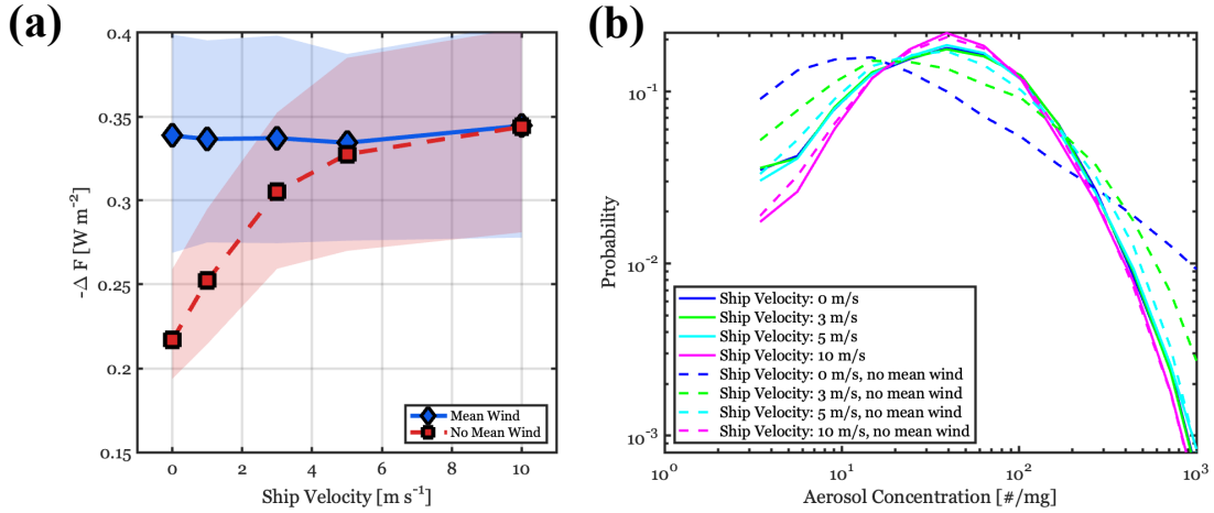
Figure 9. (a) markers indicate the ensemble-averaged global mean Twomey forcing sensitivity to ship velocity for climatological time-varying mean winds (Blue) and no mean wind (Red). Shading corresponds to the IQR of the ensemble. (b) Aerosol Ensemble mean aerosol concentration probability distributions as a function of ship velocity and mean wind/no mean wind. Sensitivity tests using \tau_{decay} = 0.5 day and N_{sprayers} = 4000 .
