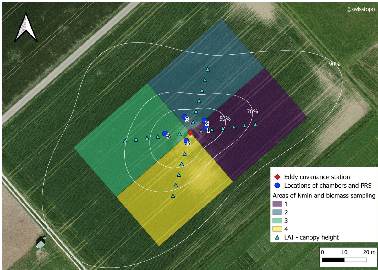
340 Figure 1. Experimental setup at the study site in Oensingen during the 2022-2023 measurement period. The red diamond marks the eddy covariance station; white lines delineate the 50%, 70%, and 90% average footprint areas (based on the Kljun et al., 2015 model); blue dots indicate locations of manual chambers and plant root simulator (PRS) probes; colored rectangles show areas for Nmin and aboveground biomass sampling; triangles denote fixed locations for LAI and canopy height measurements. Orthophoto: Federal Office of Topography swisstopo.
