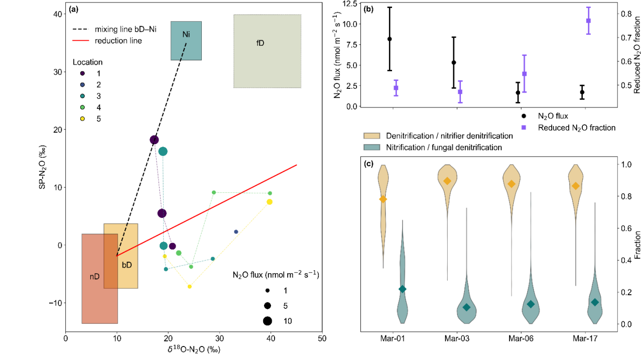
610 Figure 7. Isotopic signature of N 2 O, N 2 O flux magnitudes, and their estimated source fractions in March 2023, following fertilization applied on 27 February (ammonium-nitrate) and 28 February (slurry). (a) Dual isotope plot of \delta^{18}\text{O}-\text{N}_2\text{O} vs. site preference (SP-N 2 O). Colored boxes denote endmembers for the N 2 O mixing (nD: nitrifier denitrification, bD: heterotrophic bacterial denitrification, Ni: nitrification, fD: fungal denitrification). Endmember values of boxes are derived from Yu et al. (2020) and adjusted to the values of soil water ( \delta^{18}\text{O}-\text{H}_2\text{O} = -9.2\text{‰} ) at the study site (except for the Ni box). Lines for mixing (black) and N 2 O reduction to N 2 (red) are shown. Individual measurements are shown as circles, with size reflecting flux magnitude and color indicating location (1 to 5; see Fig. 1). (b) N 2 O fluxes measured with static chambers (black) and the fraction of N 2 O reduced to N 2 estimated by the FRAME model (purple). The latter is expressed as (1 - r) , where r denotes the residual unreduced N 2 O fraction. Values represent means \pm one standard error across measurement locations. (c) N 2 O source fractions estimated by the FRAME model, based on the mixing-reduction scenario, for heterotrophic bacterial denitrification & nitrifier denitrification vs. nitrification & fungal denitrification, displayed as violin plots, with mean values indicated by diamonds (see text for details).
