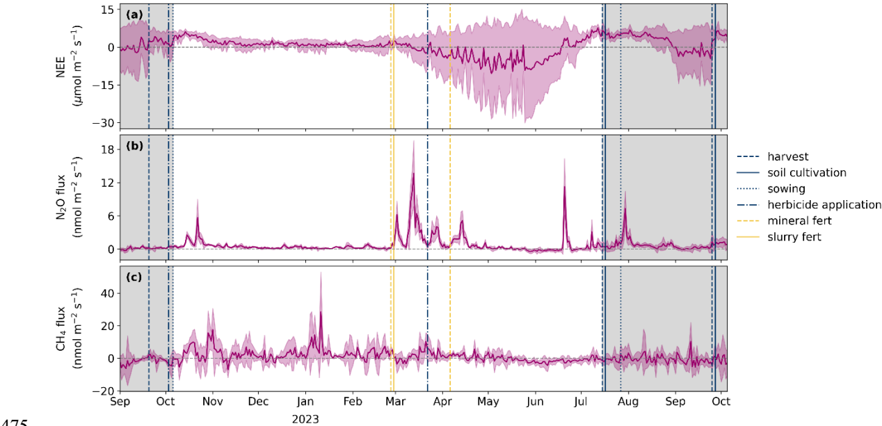
Figure 3. Gap-filled greenhouse gas fluxes at the Oensingen cropland measured from September 2022 to October 2023. The unshaded area corresponds to the winter wheat cropping season, while the shaded areas indicate the final phase of the preceding temporary grassland and the cover crop following winter harvest. (a) Net ecosystem CO 2 exchange (NEE), (b) N 2 O fluxes, and (c) CH 4 fluxes. Fluxes were gap-filled using the Marginal Distribution Sampling (MDS) for NEE and random forest (RF) for N 2 O and CH 4 fluxes. Lines represent daily averages of the gap-filled half-hourly fluxes, while the shading indicates \pm 1 standard deviation. Vertical lines mark management activities: yellow dashed = mineral fertilization (fert), yellow solid = slurry fertilization (fert), blue solid = soil cultivation, blue dotted = sowing, blue dashed = harvest, and blue dash-dot = herbicide application. See Table 1 for details on management activities.
