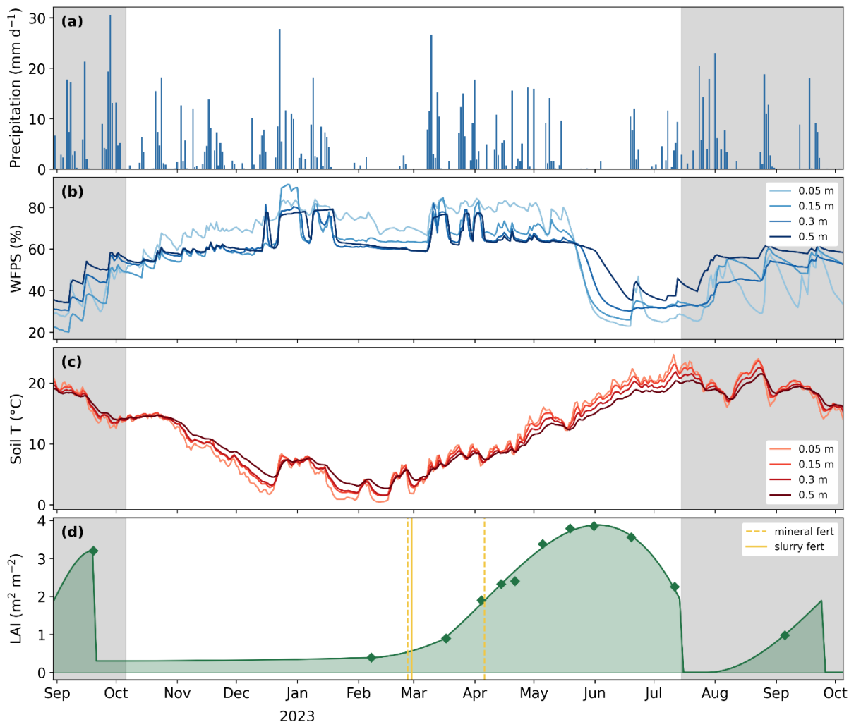
420 Figure 2. Environmental conditions and vegetation dynamics at the Oensingen cropland from September 2022 to October 2023. The unshaded area corresponds to the winter wheat cropping season, while the shaded areas indicate the final phase of the preceding temporary grassland and the cover crop following the winter wheat harvest. (a) Daily precipitation sums; (b) daily average water-filled pore space (WFPS) at 0.05, 0.15, 0.3, and 0.5 m soil depths; (c) daily average soil temperature (soil T) at the same depths as WFPS; (d) leaf area index (LAI), with diamonds indicating measured values and the line representing modelled 425 values obtained using cubic splines. Yellow lines indicate fertilization (fert) events.
