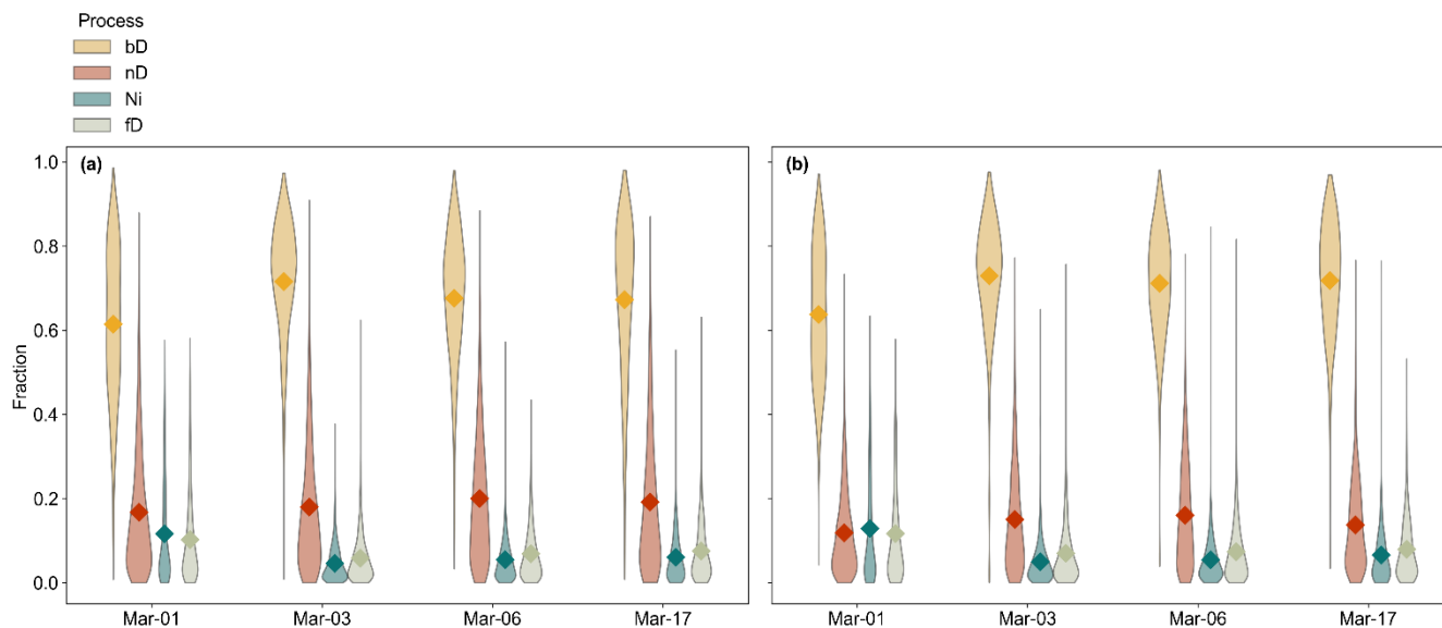
Figure A6. N 2 O source fractions estimated by the FRAME model in March 2023 following fertilization (27-28 February). Two alternative model scenarios are shown: (a) mixing-reduction, and (b) reduction-mixing. Violin plots show posterior distributions for heterotrophic bacterial denitrification (bD), nitrifier denitrification (nD), nitrification (Ni), and fungal denitrification (fD). Diamonds indicate mean values.
