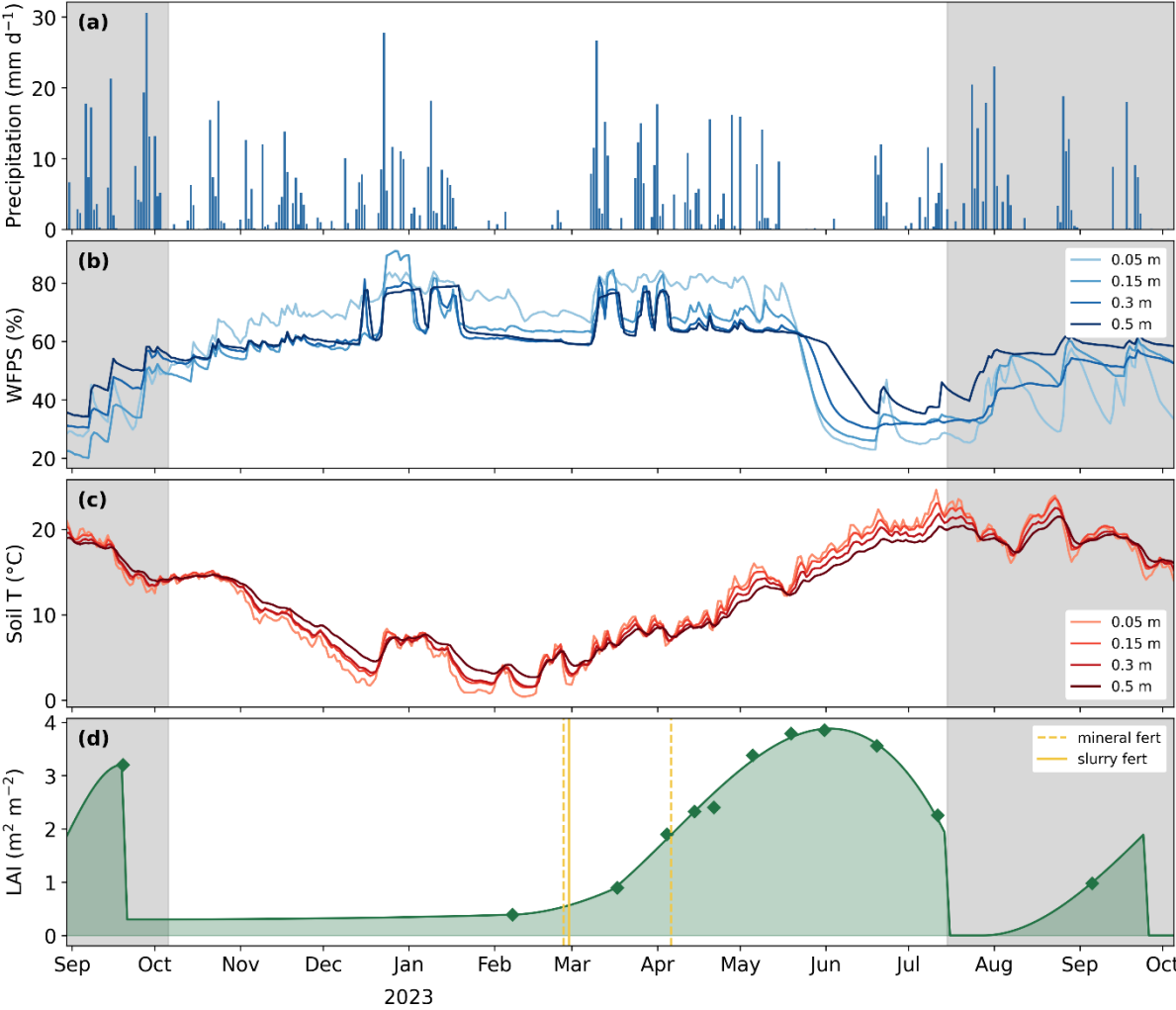
430 Figure 2. Environmental conditions and vegetation dynamics at the Oensing cropland from September 2022 to October 2023. The unshaded area corresponds to the winter wheat cropping season, while the shaded areas indicate the final phase of the preceding temporary grassland and the cover crop following the winter wheat harvest. (a) Daily precipitation sums; (b) daily average water-filled pore space (WFPS) at 0.05, 0.15, 0.3, and 0.5 m soil depths; (c) daily average soil temperature (soil T) at the same depths as WFPS; (d) leaf area index (LAI), with diamonds indicating measured values and the line representing modelled values obtained using cubic splines. Yellow lines indicate fertilization (fert) events. 435
