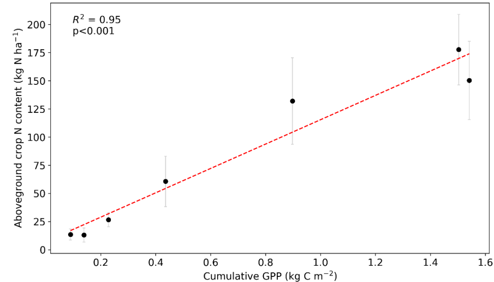
Figure A1. Relationship between cumulative gross primary productivity (GPP) and aboveground crop N content during the wheat growing season. Means \pm 1 standard deviation SD are given (n=12). The dashed red line indicates a linear least-squares regression, with the coefficient of determination (R 2 ) and respective p-value shown.
