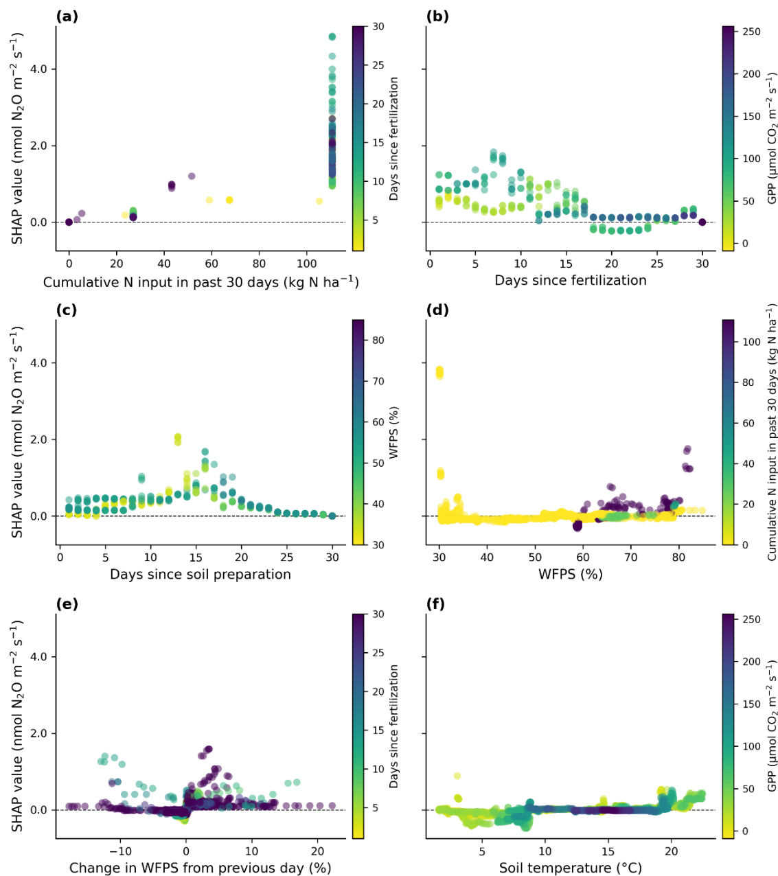
Figure A4. SHAP dependence plots for the drivers used in the XGBoost model for N 2 O fluxes (except for GPP, which is shown separately in Fig. 5). Each panel shows the SHAP values of a given driver against its observed values across all data, reflecting the driver's marginal contribution to the modelled N 2 O flux. Points are colored by a second driver.
