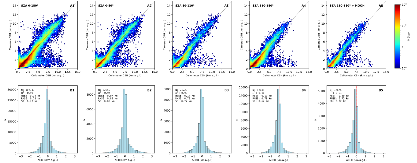
Figure 12. Bidimensional frequency histogram of median cloud heights values from the camera network within a 150 m radius of the Valladolid ceilometer location, against ceilometer values for cloud base height (CBH) and cloud top height (CTH) in panels A and C, respectively. Panels B and D represent the frequency histogram of the differences ( \Delta CBH and \Delta CTH) between both instruments. Filtering criteria have been applied to discard heights provided by two or fewer cameras, with fewer than 20 height values and a standard deviation higher than 1 km. Rows represent different lighting conditions: SZ 0 – 180° (all conditions), SZ 0 – 80° (daylight), SZ 80 – 110° (twilight), SZ 110 – 180° (night), and SZ 110 – 180° (night with moon presence). Results include total number of cases (N), coefficient of determination ( R^2 ), mean bias error (MBE), root mean square error (RMSE) and standard deviation (SD).
