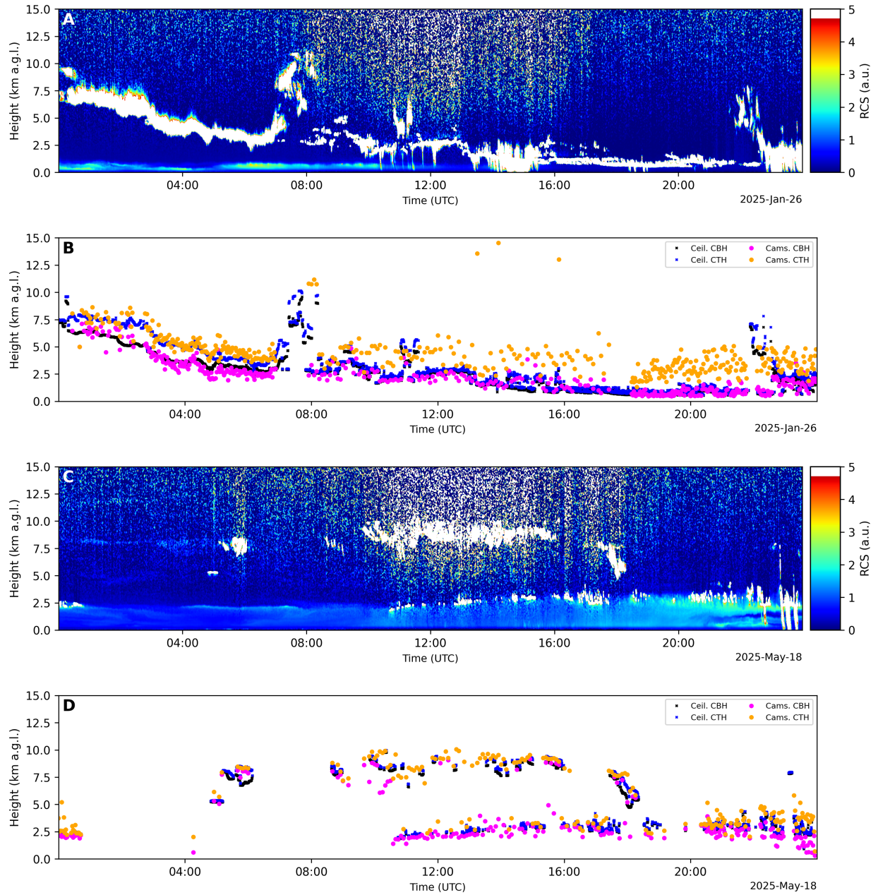
Figure 15. Temporal evolution for three two different days of the ceilometer range corrected signal (RCS) overlaid with the cloud base and top heights (CBH and CTH) and those estimated by the all-sky camera network. Camera values are based on the median height value within a 150 m radius of the ceilometer location.
