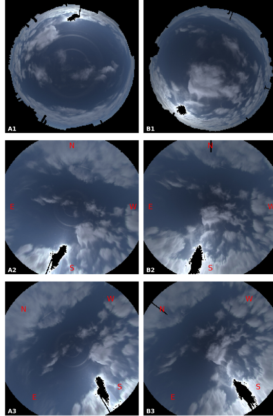
Figure 2. Sky images captured by cameras C013 and C014 on 28 December 2025 at 11:20 UTC. It is shown: fisheye original HDR all-sky images, with the obstacle objects and the sun saturated pixels colored black (A1, B1), their planar projection oriented upside to North (A2, B2) and their planar projection oriented so the rows of both images align (A3, B3).
