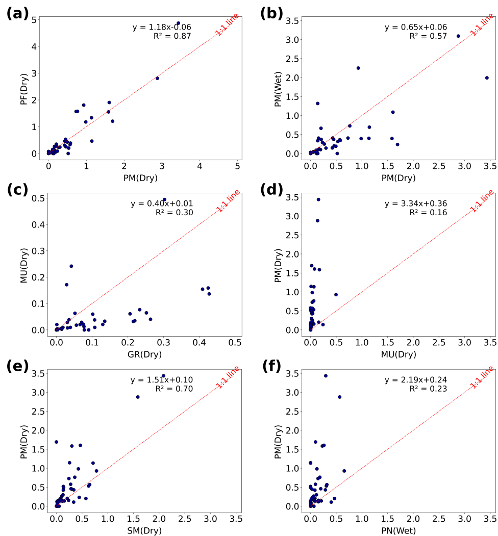
Figure S7. Correlation plots of mean, overall VOC EF ( \text{g kg}^{-1} ) for select biomass fuel pairs. The red line indicates the 1:1 line.
