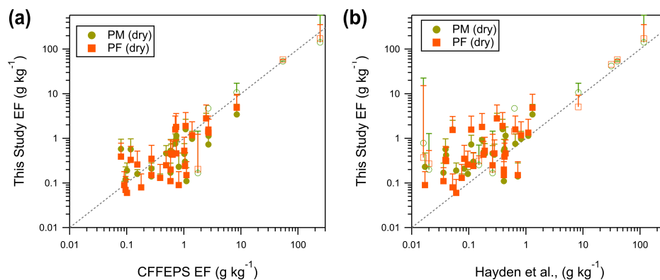
Figure S10. EF ( \text{g kg}^{-1} ) for 32 VOC (solid symbols) and other trace gas species (open symbols) (Moraes et al., 2026) for dry peat fuels [PM (dry) - green circle, PF (dry) - orange squares] compared to (a) CFFEPS EFs for residual/smoldering combustion of boreal forest duff/organic soil from Urbanski (2014) and (b) EFs measured by aircraft for a boreal wildfire from Hayden et al. (2022). The dotted line is the 1:1 line.
