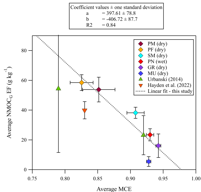
Figure S9. Average \text{NMOC}_G EF ( \text{g kg}^{-1} ) as a function of average MCE for low-moisture content fuels from this study (diamonds). The dashed grey line is a linear fit to the study data. The average \text{NMOC}_G EF from Hayden et al. (2022) (orange inverted triangle) and Urbanski (2014), “Boreal forest duff” and “Wildfire boreal forest” (green triangles), are also plotted.
