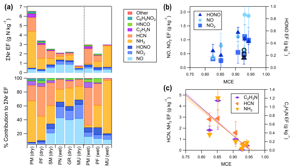
Figure 6. (a) EF of Nr species ( \text{g N kg}^{-1} ) on the top panel and their % contribution to \Sigma \text{Nr} on the bottom panel; (b) NO, \text{NO}_2 , and HONO EFs ( \text{g kg}^{-1} ); and (c) HCN, \text{NH}_3 , and \text{C}_2\text{H}_3\text{N} EFs ( \text{g kg}^{-1} ) as a function of fire-integrated MCE for the low-moisture content fuels [MU (dry), GR (dry), SM (dry), PN (wet), PF (dry), PM (dry)]. MU (dry) EFs are outlined in black in Fig. 6b. Error bars represent the standard deviation of the mean. The dashed lines in Fig. 6(c) are linear fits to the data.
