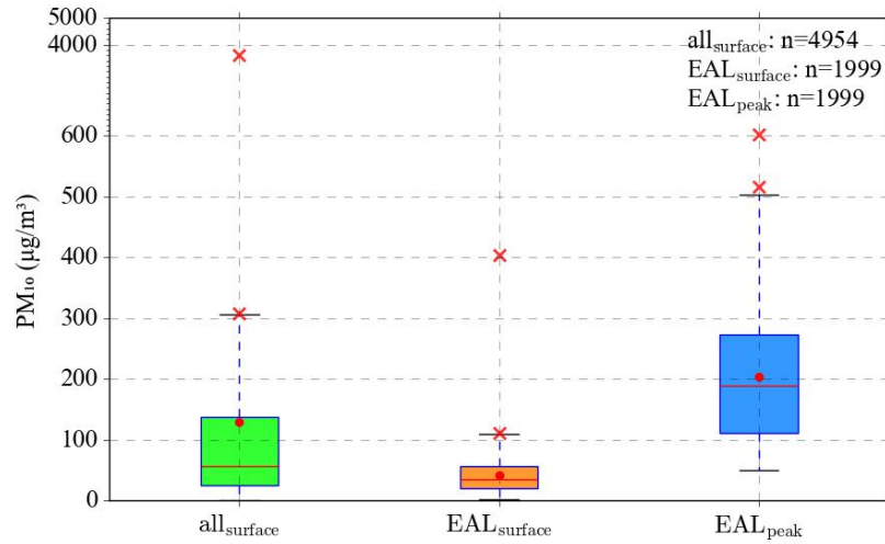
Fig. 12. Boxplots of PM 10 concentrations during the experiment at the Dunhuang site, including surface values for all days, surface values during elevated aerosol layer (EAL) days, and peak values within elevated aerosol layers. The red lines represent the median, red dots indicate the mean values, the box edges denote the 25th and 75th percentiles (Q1 and Q3), and the whiskers represent non-outlier data points. Outliers (values beyond Q3 + 1.5 × IQR or below Q1 – 1.5 × IQR) are marked with red crosses, with only the minimum and maximum outliers labelled for clarity. Under a normal distribution, the whiskers encompass approximately 99% of the data.
