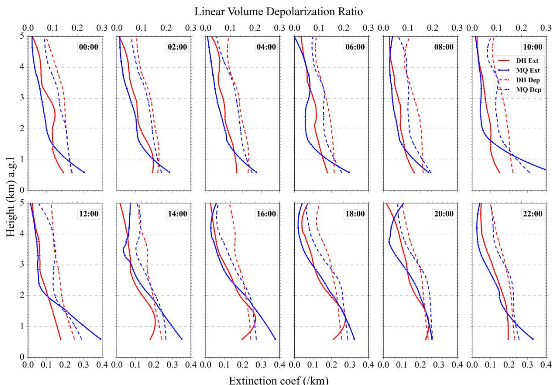
Fig. 6 Hourly averaged vertical profiles of aerosol extinction coefficient (solid lines) and linear volume depolarization ratio (dashed lines) during the experimental periods at Dunhuang (red lines) and Minqin (blue lines).
