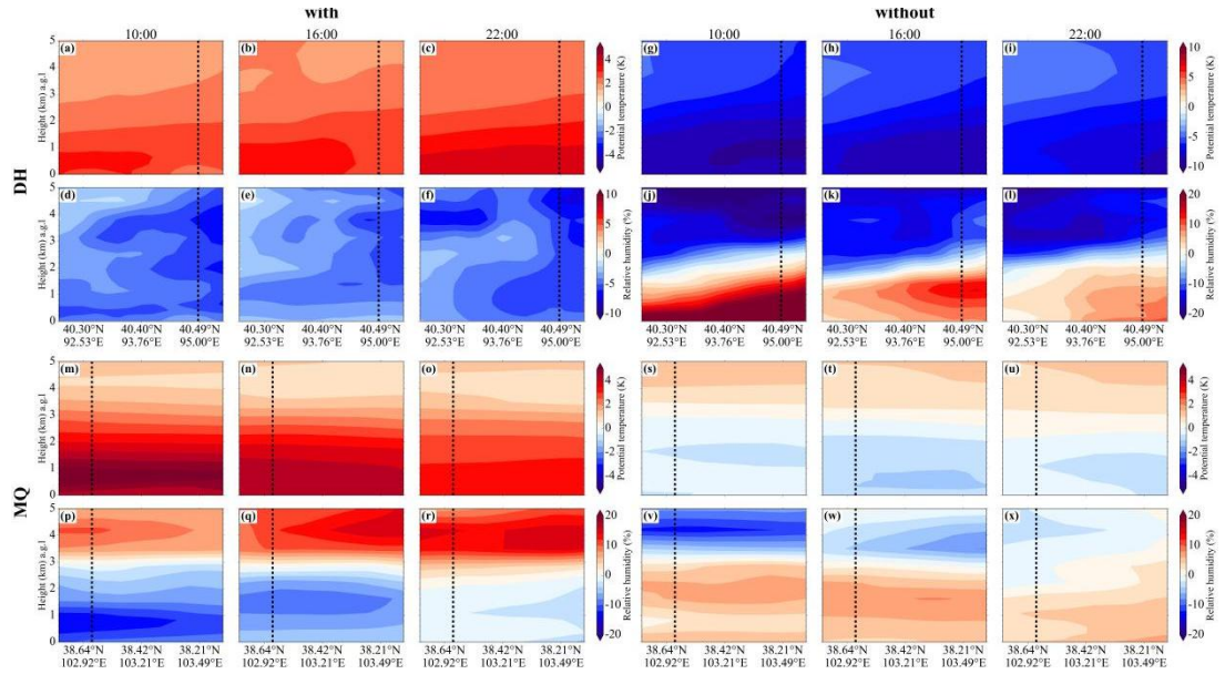
Fig. 11. Anomalies of potential temperature and relative humidity between the mean states during periods with and without elevated aerosol layers and the summer climatological state at Dunhuang and Minqin.
