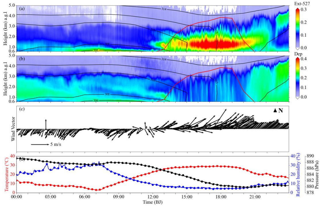
Fig. 7. Time series of aerosol vertical distribution and meteorological parameters at Dunhuang on 21 April 2012. (a) Time–height cross-sections of aerosol extinction coefficient and (b) depolarization ratio derived from MPL lidar, with potential temperature contours (black lines) and boundary layer height (red lines) from ERA5. (c) wind vectors measured by an automatic meteorological station (model WXT520), and (d) temperature, relative humidity, and pressure.
