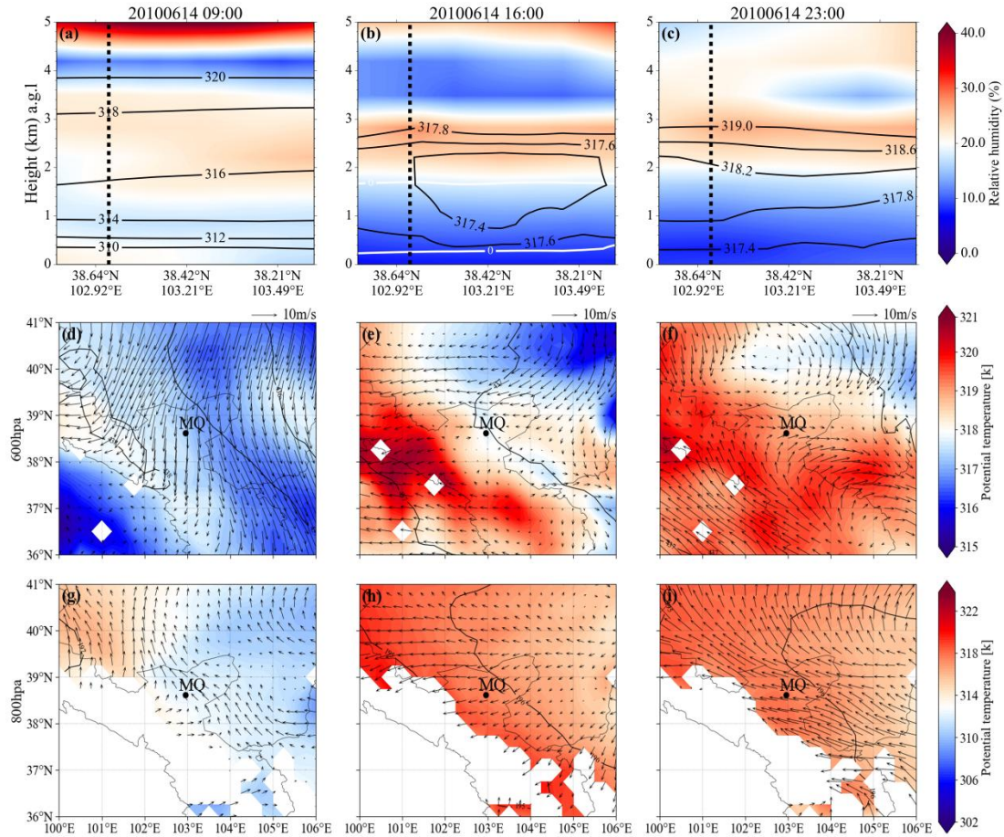
Fig. 10. Thermal and dynamical fields at Minqin on 14 June 2010. (a–c) Vertical cross-sections of relative humidity with unstable stratification (demarcated by the white enclosed area) along the transect indicated by the red line in Fig. 1. Black solid lines represent isotherms, while black dashed lines denote the location of the observation site. (d–i) Meteorological fields at the 600 hPa and 800 hPa levels, with geopotential height contours, during the experimental period over the Minqin region. White regions indicate elevated mountain terrain.
