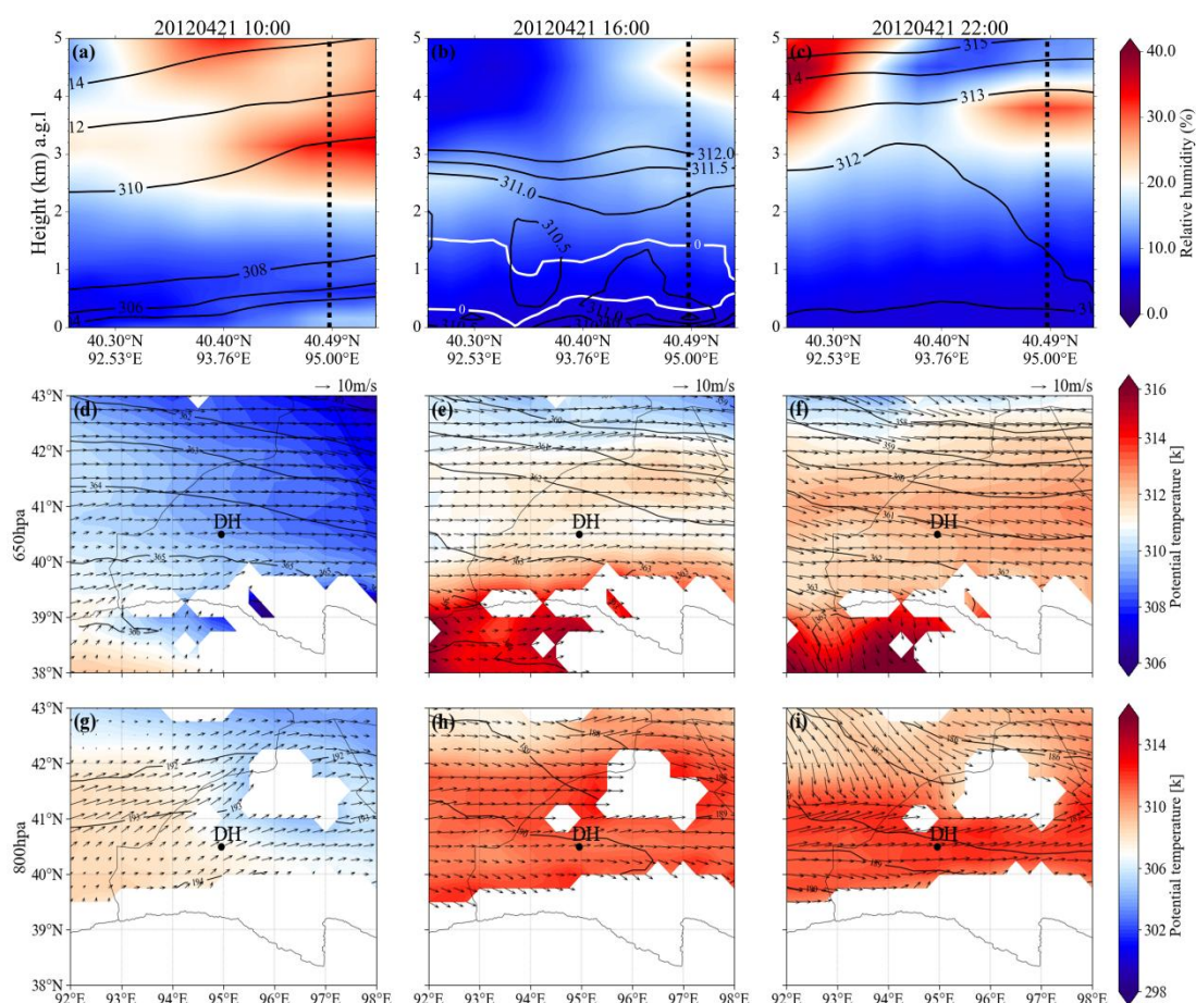
Fig. 8. Thermal and dynamical fields at Dunhuang on 21 April 2012. (a–c) Vertical cross-sections of relative humidity with unstable stratification (demarcated by the white enclosed area) along the transect indicated by the red line in Fig. 1. Black solid lines represent isotherms, while black dashed lines denote the location of the observation site. (d–i) Meteorological fields at the 650 hPa and 800 hPa levels, with geopotential height contours, during the experimental period over the Dunhuang region. White regions indicate elevated mountain terrain.
