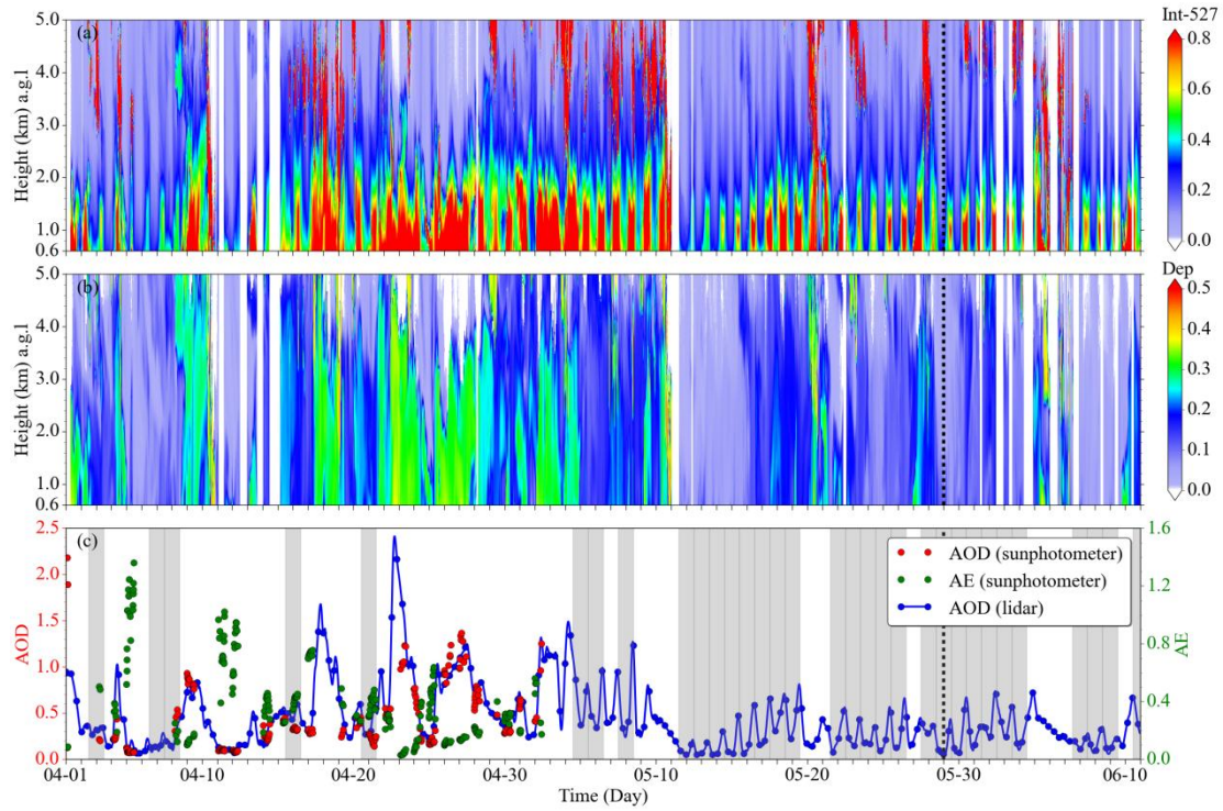
Fig. 4. Time series of observations obtained from a micro-pulse lidar (MPL) and a sun photometer during the intensive observation period at Dunhuang in 2012. Time–height cross-sections of (a) normalised relative backscatter (NRB) and (b) linear volume depolarization ratio (Dep) derived from MPL observations. (c) Time series of aerosol optical depth (AOD) retrieved from AERONET at 500 nm (red dots) and from MPL at 527 nm, along with the Ångström exponent (AE) at 440–870 nm (green dots). All identified elevated aerosol layers are indicated by shaded regions, and the representative case selected for detailed discussion is highlighted with black dashed lines.
