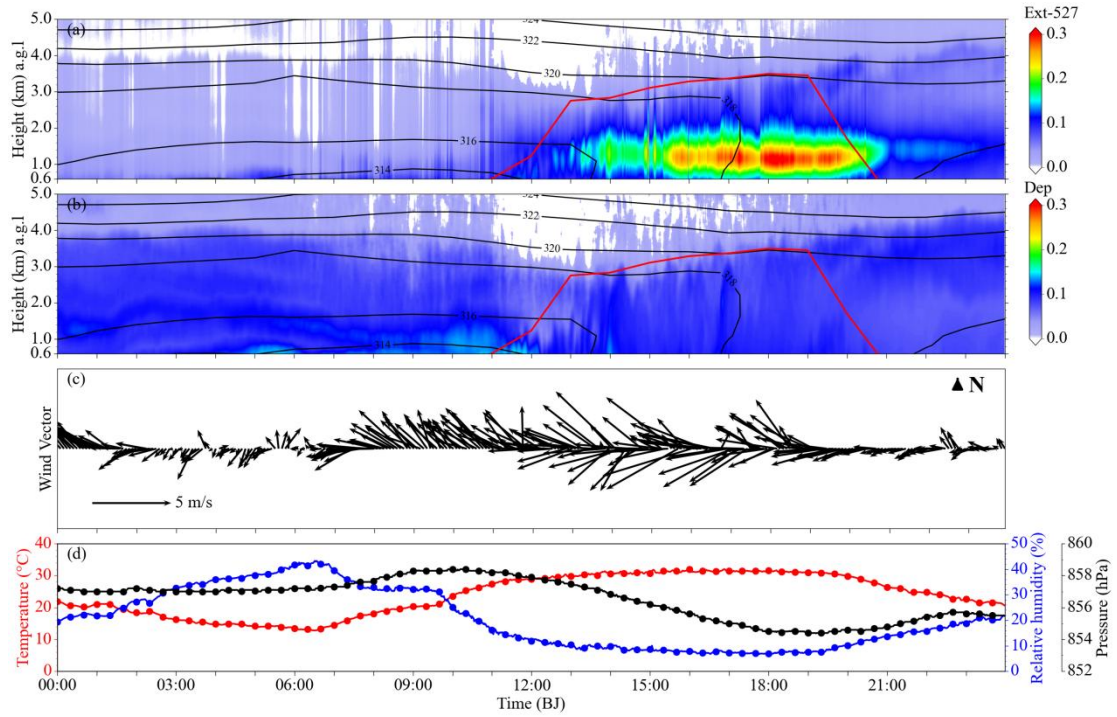
Fig. 9. Time series of aerosol vertical distribution and meteorological parameters at Minqin on 14 June 2010. (a) Time–height cross-sections of aerosol extinction coefficient and (b) depolarization ratio derived from MPL lidar, with potential temperature contours (black lines) and boundary layer height (red lines) from ERA5. (c) wind vectors measured by an automatic meteorological station (model WXT520), and (d) temperature, relative humidity, and pressure.
