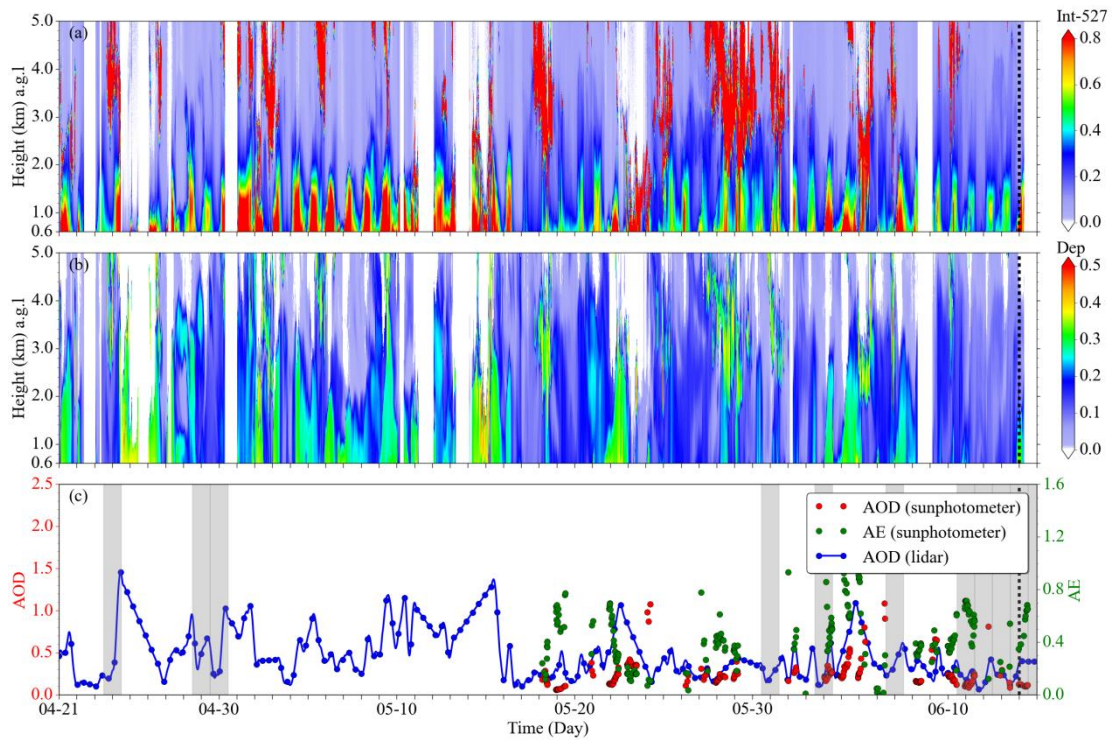
Fig. 5. Time series of observations obtained from a micro-pulse lidar (MPL) and a sun photometer during the intensive observation period at Minqin in 2010. Time–height cross-sections of (a) normalised relative backscatter (NRB) and (b) linear volume depolarization ratio (Dep) derived from MPL observations. (c) Time series of aerosol optical depth (AOD) retrieved from AERONET at 500 nm (red dots) and from MPL at 527 nm, along with the Ångström exponent (AE) at 440–870 nm (green dots). All identified elevated aerosol layers are indicated by shaded regions, and the representative case selected for detailed discussion is highlighted with black dashed lines.
