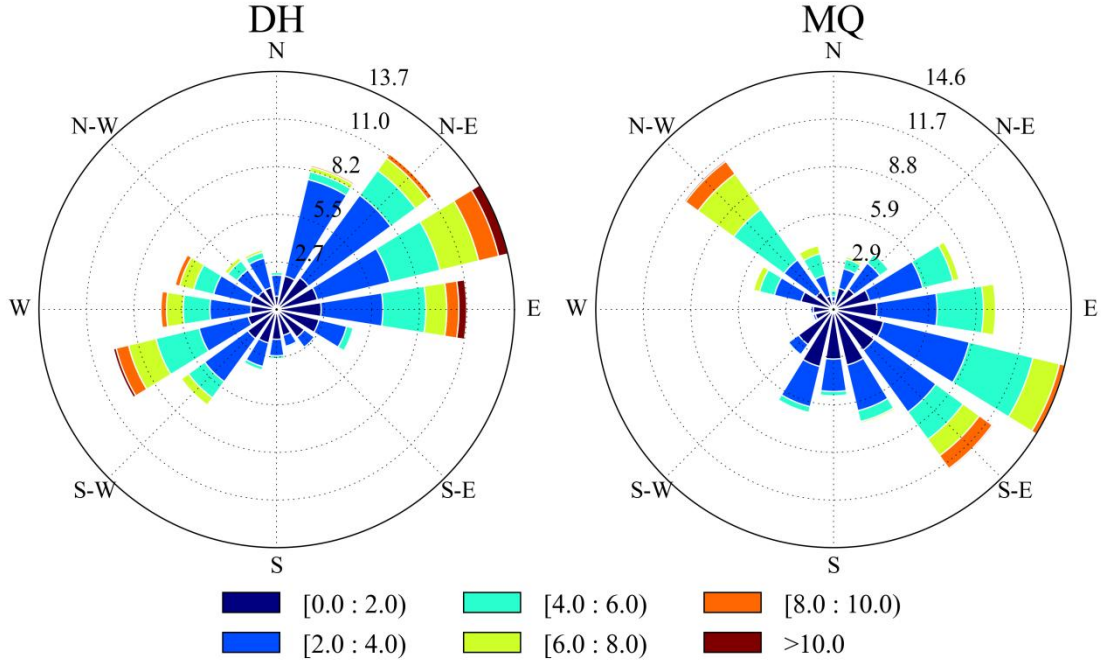
Fig. 3. Surface wind speed and wind direction during the intensive observation periods at Dunhuang from 1 April to 10 June 2012 (left) and Minqin from 21 April to 15 June 2010 (right).
