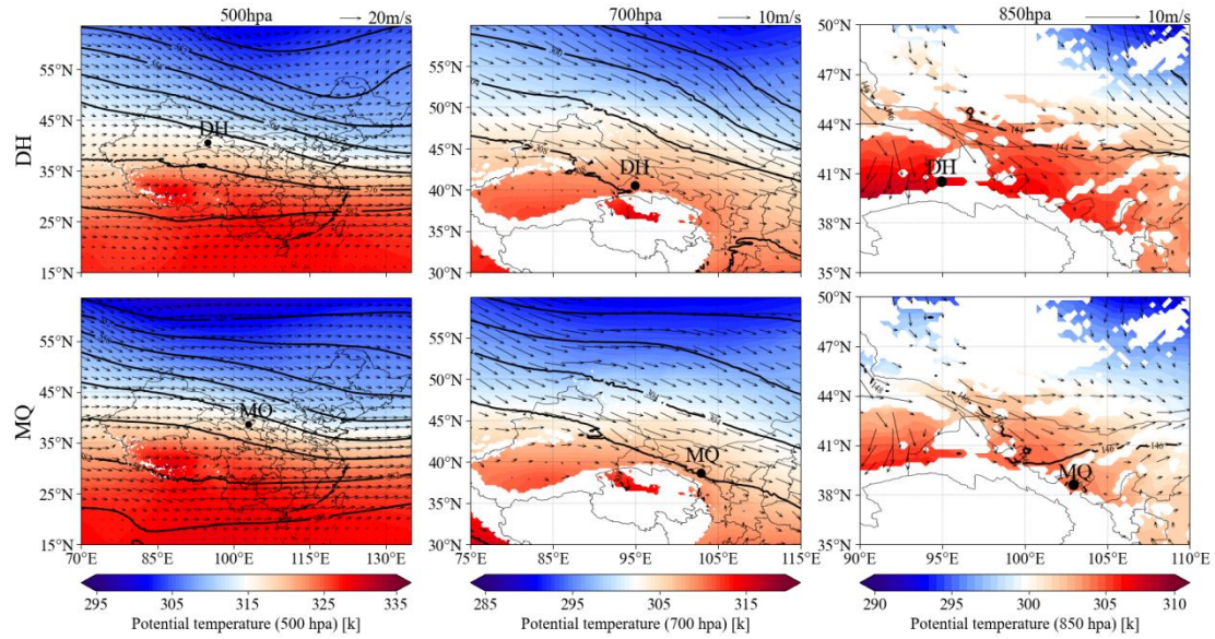
Fig. 2. Mean meteorological fields during the two intensive observation periods (Dunhuang: 1 April–10 June 2012; Minqin: 21 April–15 June 2010), with geopotential height contours. The white regions indicate elevated mountainous terrain.
