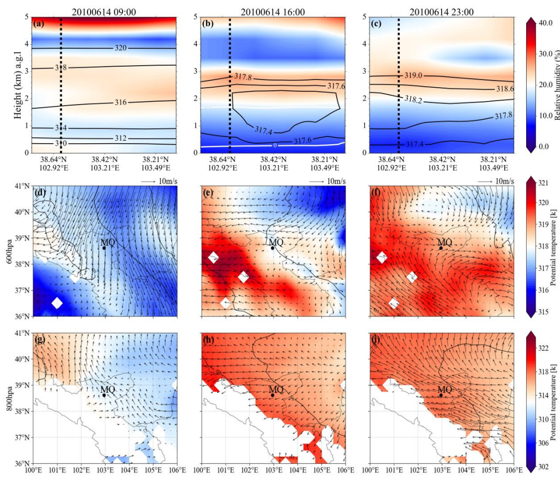
Fig. 10. Thermal and dynamical fields at Minqin on 14 June 2010. (a–c) Vertical cross-sections of relative humidity with unstable stratification (demarcated by the white enclosed area) along the transect indicated by the red line in Fig. 1. Black solid lines represent isotherms, while black dashed lines denote the location of the observation site. (d–i) Meteorological fields at the 600 hPa and 800 hPa levels, with geopotential height contours, during the experimental period over the Minqin region. White regions indicate elevated mountain terrain.
