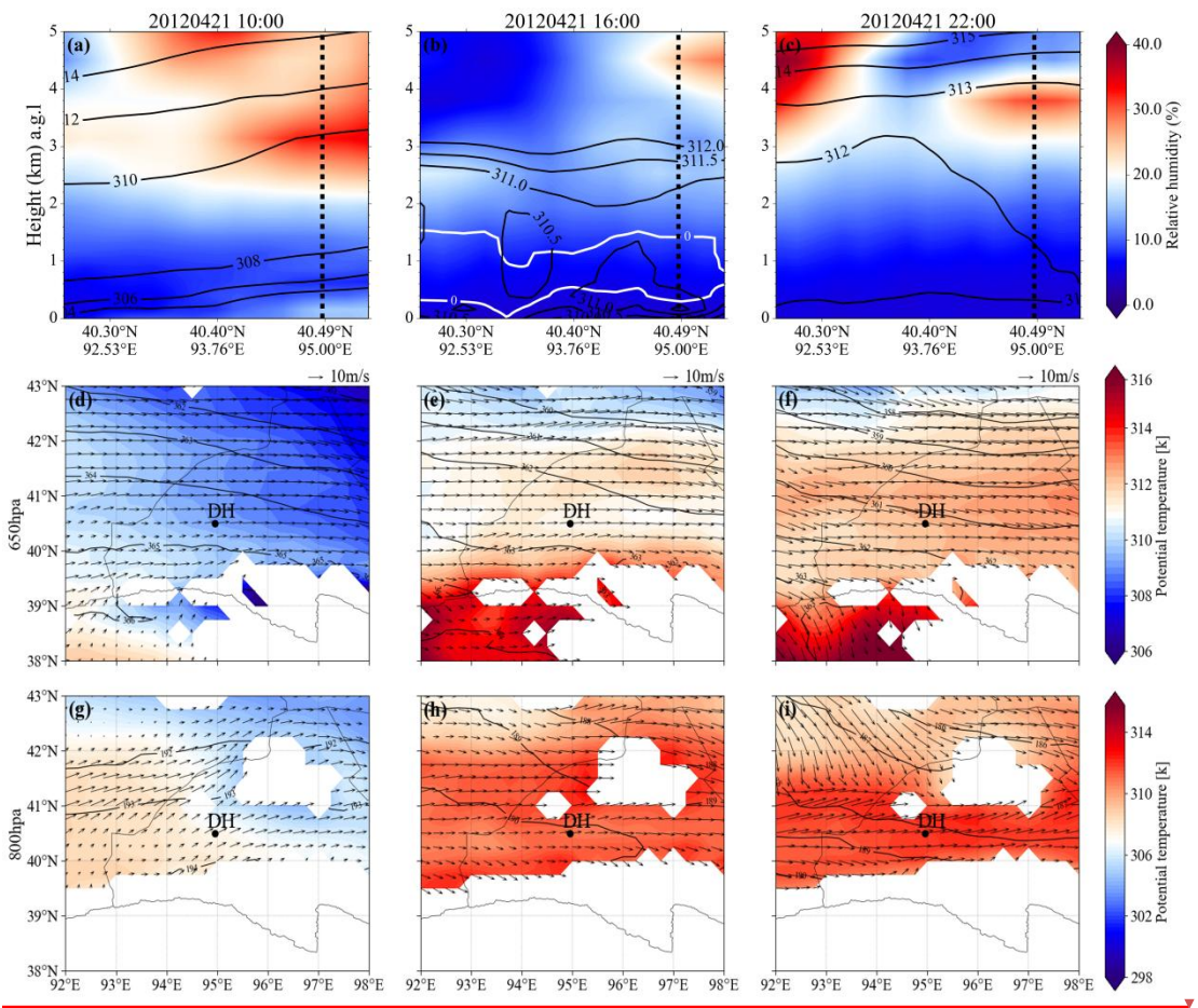
Fig. 8. Thermal and dynamical fields at Dunhuang on 21 April 2012. (a–c) Vertical cross-sections of relative humidity with unstable stratification (demarcated by the white enclosed area) along the transect indicated by the red line in Fig. 1. Black solid lines represent isotherms, while black dashed lines denote the location of the observation site. (d–i) Meteorological fields at the 650 hPa and 800 hPa levels, with geopotential height contours, during the experimental period over the Dunhuang region. White regions indicate elevated mountain terrain.
