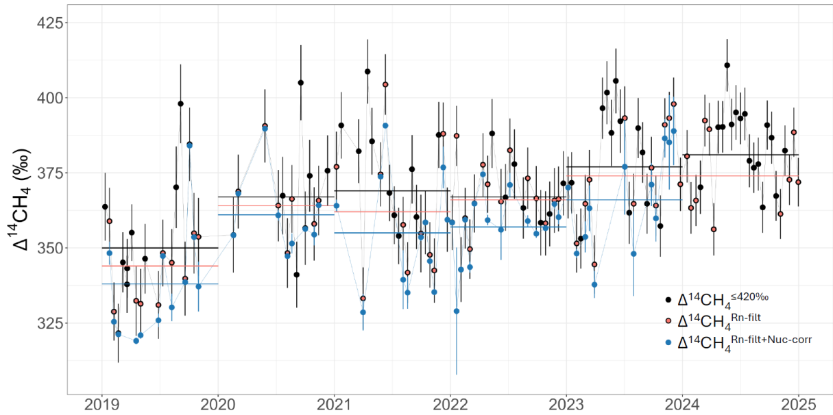
Figure 3: Nuclear influence on background \Delta^{14}\text{CH}_4 measurements at JFJ with values \leq 420 ‰ ( \Delta^{14}\text{CH}_4 \leq 420 ‰) (black points). Red symbols denote points where Rn is lower than 1.5 \text{ Bq m}^{-3} \text{ STP} ( \Delta^{14}\text{CH}_4^{\text{Rn-filt}} ) (same as in Fig. 2a,b). Black error bars show the statistical uncertainty of the individual \Delta^{14}\text{CH}_4 measurements. Blue points correspond to the red points after subtraction of the simulated nuclear influence ( \Delta^{14}\text{CH}_4^{\text{Rn-filt} + \text{Nuc-corr}} ). Blue error bars represent the standard deviation of the nuclear influence. Horizontal black, red and blue lines show the annual mean values derived from the black (Table 1, \Delta^{14}\text{CH}_4 \leq 420 ‰), red (Table 1, \Delta^{14}\text{CH}_4^{\text{Rn-filt}} ) and blue points (Table 1, \Delta^{14}\text{CH}_4^{\text{Rn-filt} + \text{Nuc-corr}} ), respectively. \Delta^{14}\text{CH}_4^{\text{Rn-filt} + \text{Nuc-corr}} values were not available for 2024 due to missing input parameters for the nuclear simulation for this year.
