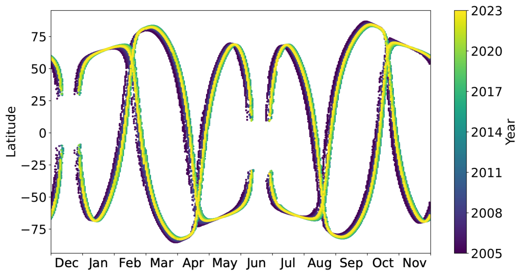
Figure 1: Latitudinal coverage of the ACE-FTS measurements for 2005-2023.
