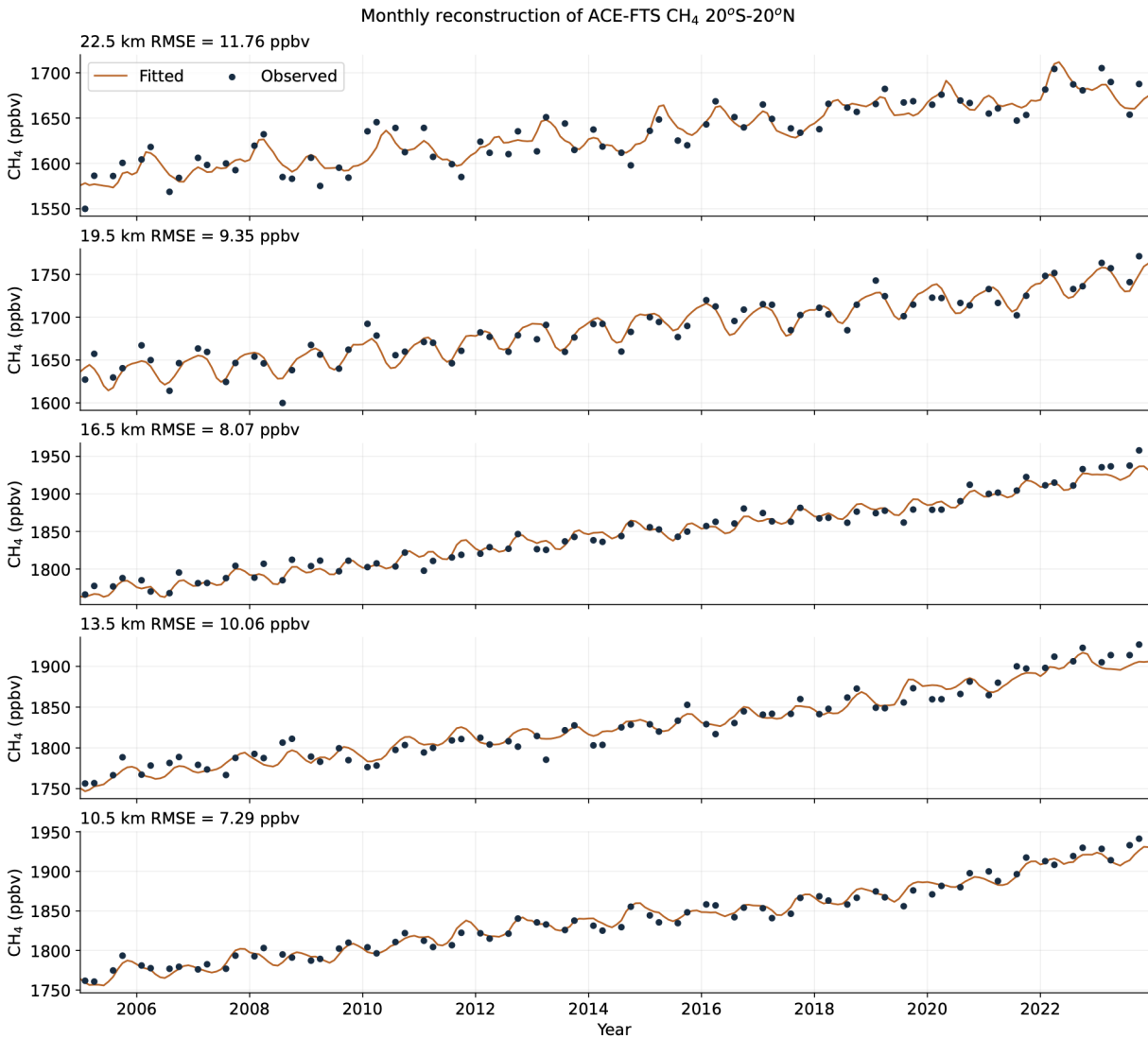
Figure A1: Monthly reconstruction of ACE-FTS CH 4 mixing ratios averaged over 20°S–20°N at selected altitudes during 2005–2023. Black dots represent observations available in February, April, August, and October. Red lines show monthly reconstructions from regression fits. Regressions were fitted separately at each altitude using only available observations. The root-mean-square error (RMSE) between fitted and observed values is indicated above each panel.
