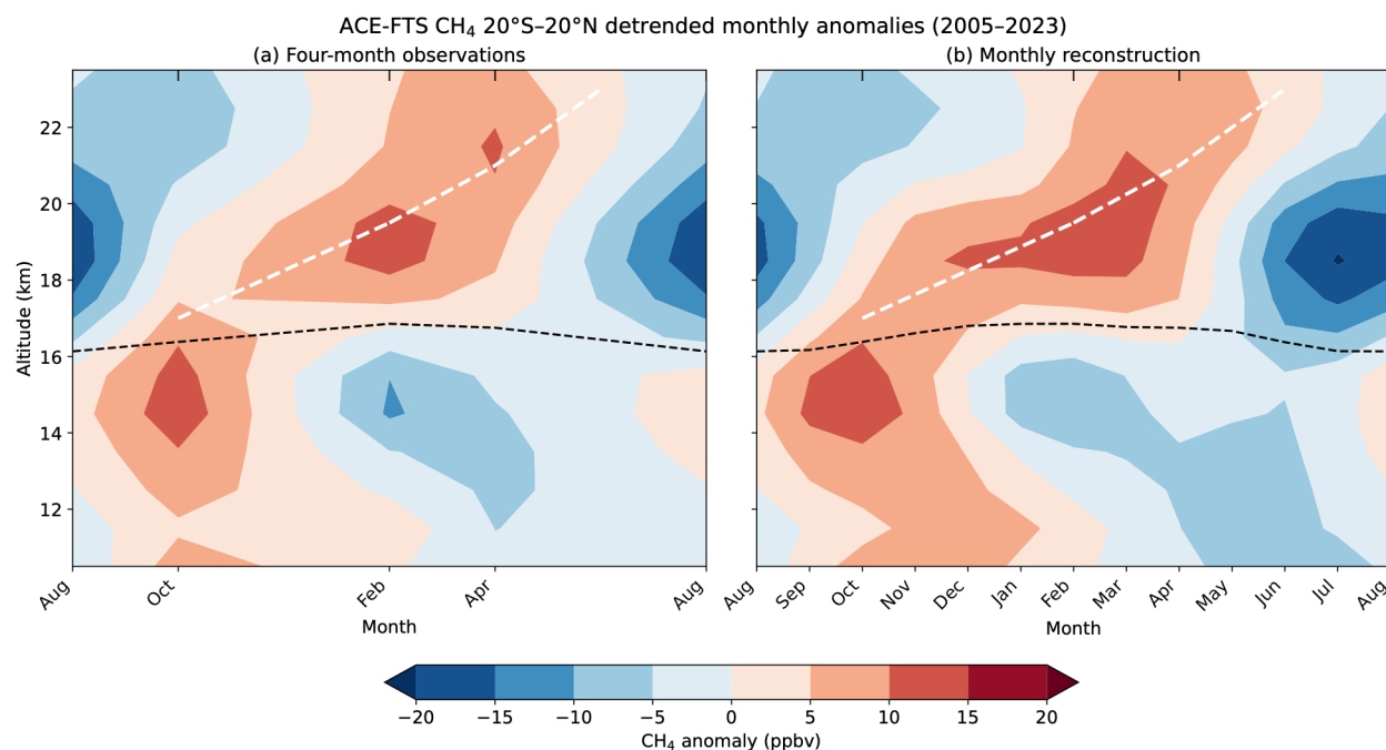
Figure 10: Climatological detrended monthly anomalies of ACE-FTS CH 4 averaged over 20°S–20°N during 2005–2023, derived from (a) observations in August, October, February and April (b) monthly reconstructions using regression fit including annual and semi-annual cycle. At each altitude, the linear trend is first removed from both observations and reconstructed values. Anomalies are then calculated relative to each year’s mean of the four detrended observation months in (a) and the 12 detrended reconstructed months in (b), before averaging each month across the 19 years. Black dashed lines indicate the climatological tropopause height. White dashed lines in (a) trace the maximum anomalies at each altitude to indicate the possible upward progression of positive anomalies. The same white dashed lines are overlaid in (b) for comparison. August is repeated at the right edge to show continuity across the annual cycle.
