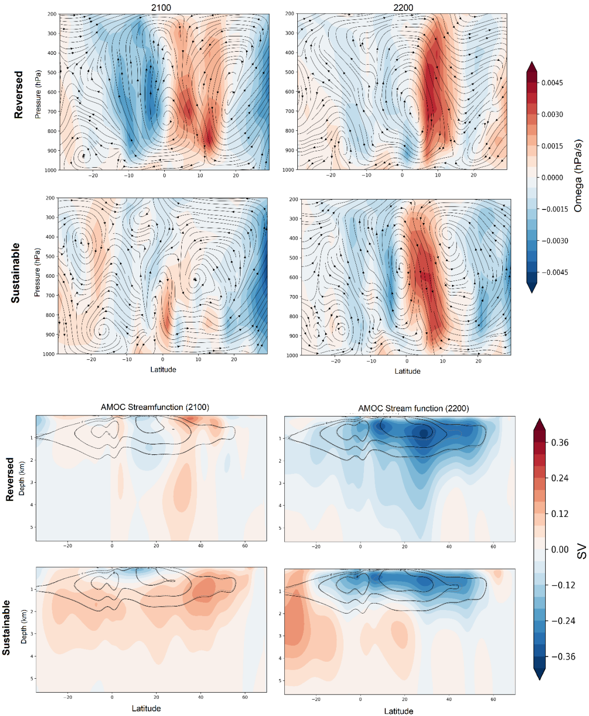
Figure S7. Top) Differences in the Hadley circulation between both scenarios and the baseline at the end of the 21st and 22nd centuries. Contour data are vertical velocity ( \omega ); streamlines are the resultant vectors of \omega \times 1000 and meridional wind. Data are averaged over tropical latitudes. Bottom) The Atlantic meridional overturning circulation (AMOC), (contours, in Sv, only values above 4 Sv shown with a 4 Sv interval) for a forest (black) and baseline (gray), as well as differences of experiments relative to baseline (shading, in Sv).
