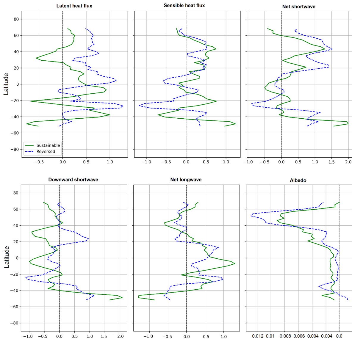
Figure S3. The zonal changes (10-degree mean) in the energy balance parameters ( W/m^2 ) and unitless albedo in the reforested area for two land cover scenarios, including latent and sensible heat fluxes, incoming short-wave and net short-wave and long-wave radiation. The changes are calculated by the difference between the 2100:2090-2110 mean for each scenario and the baseline simulation. Colors are blue for the Reversed and green for the Sustainable scenarios. Note that each plot has a different scale
