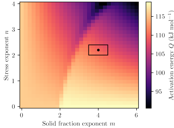
Figure 10. Apparent activation energy estimated from the experimental measurements as a function of the model parameters m and n . The rectangle indicates the range of physically meaningful parameters ( m = 4 \pm 1 and n = 2.2 \pm 0.2 ).
