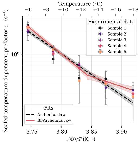
Figure 8. Scaled strain rate prefactor \dot{\epsilon}_0 as a function of inverse temperature for all studied samples, corrected for second-order microstructural effects.
