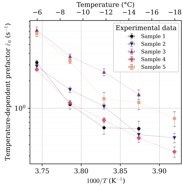
Figure A2. Strain rate prefactor \dot{\epsilon}_0 as a function of inverse temperature for all studied samples.
