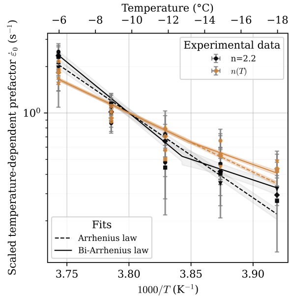
Figure A3. Scaled strain rate prefactor \dot{\epsilon}_0 as a function of inverse temperature for all studied samples considering a constant stress exponent and the stress exponent temperature sensitivity proposed by Jones and Brunet (1978).
