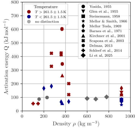
Figure 1. Reported activation energies of the viscoplastic behaviour of the snow-firm-ice continuum as a function of density and temperature regime.
