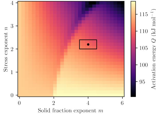
Figure 10. Activation - Apparent activation energy estimated from the experimental measurements as a function of the model parameters m and n . The rectangle indicates the range of physically meaningful parameters ( m = 4 \pm 1 and n = 2.2 \pm 0.2 ).
