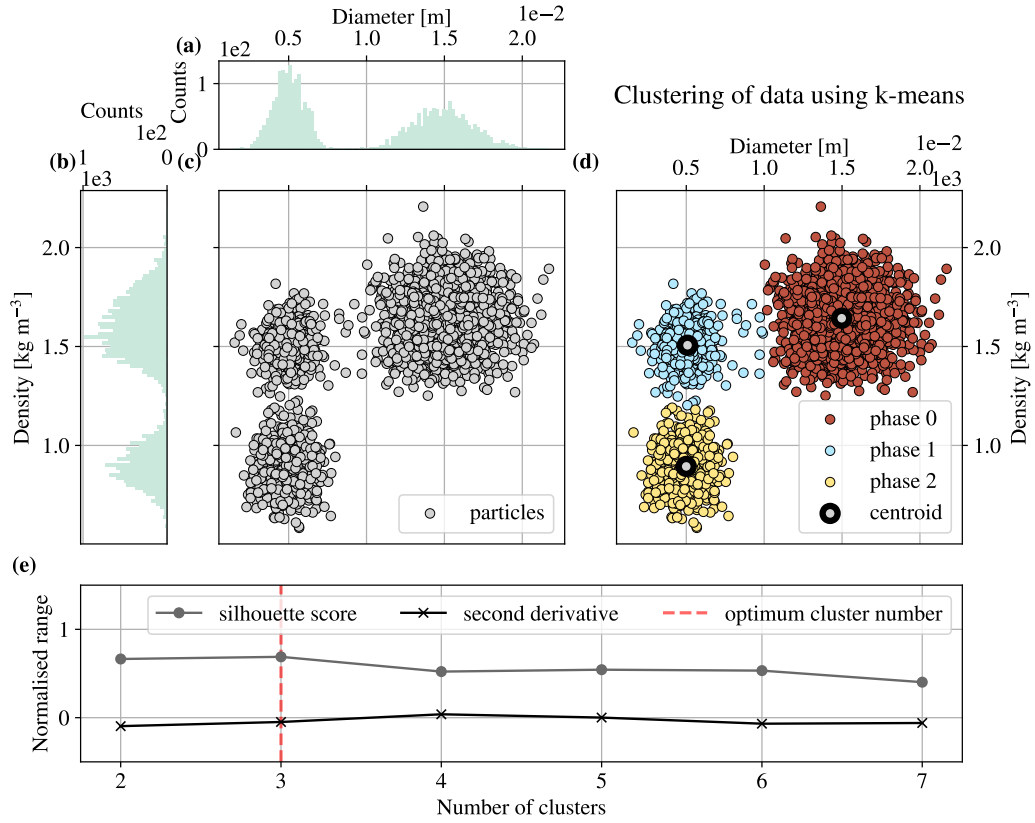
Figure 4. Illustration of the approach to detect particle phases. Synthetic data set of a bimodal particle diameter distribution (a). Synthetic data set of a bimodal particle density distribution (b). Cross-plot corresponding to the diameter and density distributions in (a) and (b), respectively (c). Cross-plot containing the same particle samples as (c) coloured by the phase they are classified to according to the k-means algorithm using the optimum number of clusters (d). Silhouette score for a given number of clusters employed in the k-means algorithm (grey), and the corresponding second derivative (black) (e). The absolute maximum in (e) is chosen to be the optimum number of clusters (dashed red).
