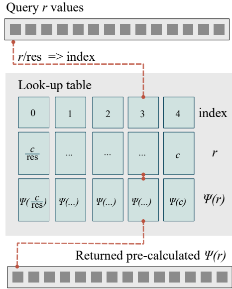
Figure B2. Schematic diagram of the lookup table algorithm implemented in Pysammos. r corresponds to the distance between a particle and a grid point. The resolution of the lookup table is res . \Psi(r) is the coarse-graining function, and c corresponds to its cut-off distance (i.e., \Psi(c) = 0 ).
