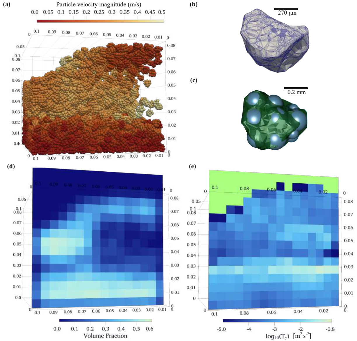
Figure 15. DEM simulation of a granular bed, fluidised with a gas velocity of 2 \text{ m s}^{-1} , using glued-sphere particles (a). Reconstructed ash particle shape from (Gabellini et al., 2025) (b), to which the glued-sphere particles in (a) are approximated, as shown in (c). Coarse-grained fields of the volume fraction (d) and vertical granular temperature (e) corresponding to the simulation time step shown in (a). Note that the pale green colour in (e) indicates NaN. This occurs at locations where T_y is set to 0 \text{ m}^2 \text{s}^{-2} by convention (see Appendix C2). Consequently, \log_{10}(0) is undefined and is represented as NaN in ParaView.
