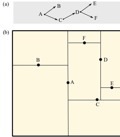
Figure B1. Simplified example of a kd-tree in 2D (a) corresponding to the divisions in space shown in (b). Each level of the tree corresponds to a labelled line in the spatial visualisation. The levels of the tree alternate in axes (e.g., A is vertical, B and C are horizontal). Note that only a single branch is built completely, while others stop in earlier levels.
