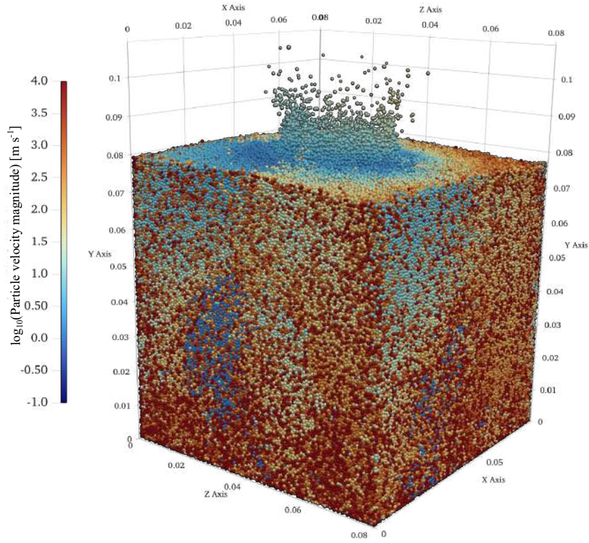
Figure 10. DEM numerical simulation of a polydisperse cuboid bed, of spherical particles initially at rest, hit at high velocity by an impactor larger in size.
