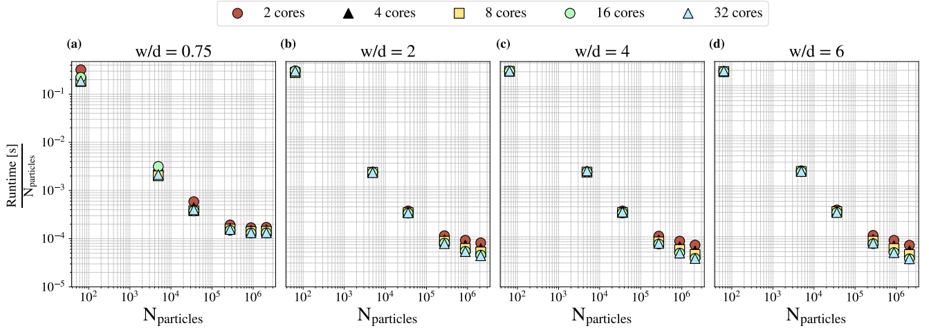
Figure 8. Computational cost per particle, and per time step, as the dataset size increases using a different number of CPUs for parallelisation. The cost per particle is measured as the runtime duration (in seconds) normalised by the number of particles within the region of the model being processed. The performance was compared across different search radii, w/d : the default 0.75 (a), 2 (b), 4 (c) and 6 (d).
