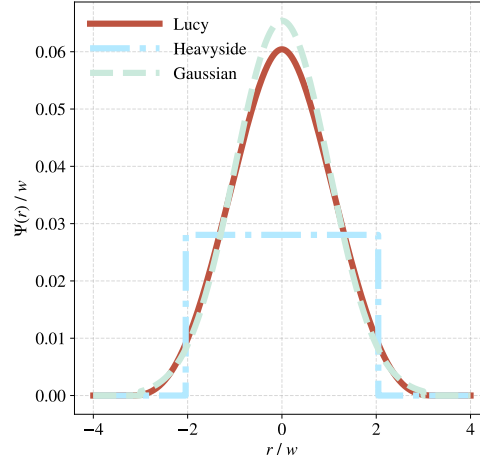
Figure 6. Visualisation of the three implemented coarse-graining weighting functions, \Psi(r) , in one dimension ( r ) normalised by the half-width-effective smoothing width ( w ). Note that the functions have been plotted with equal variance in order to ensure that any differences are due to kernel shape, not scale.
