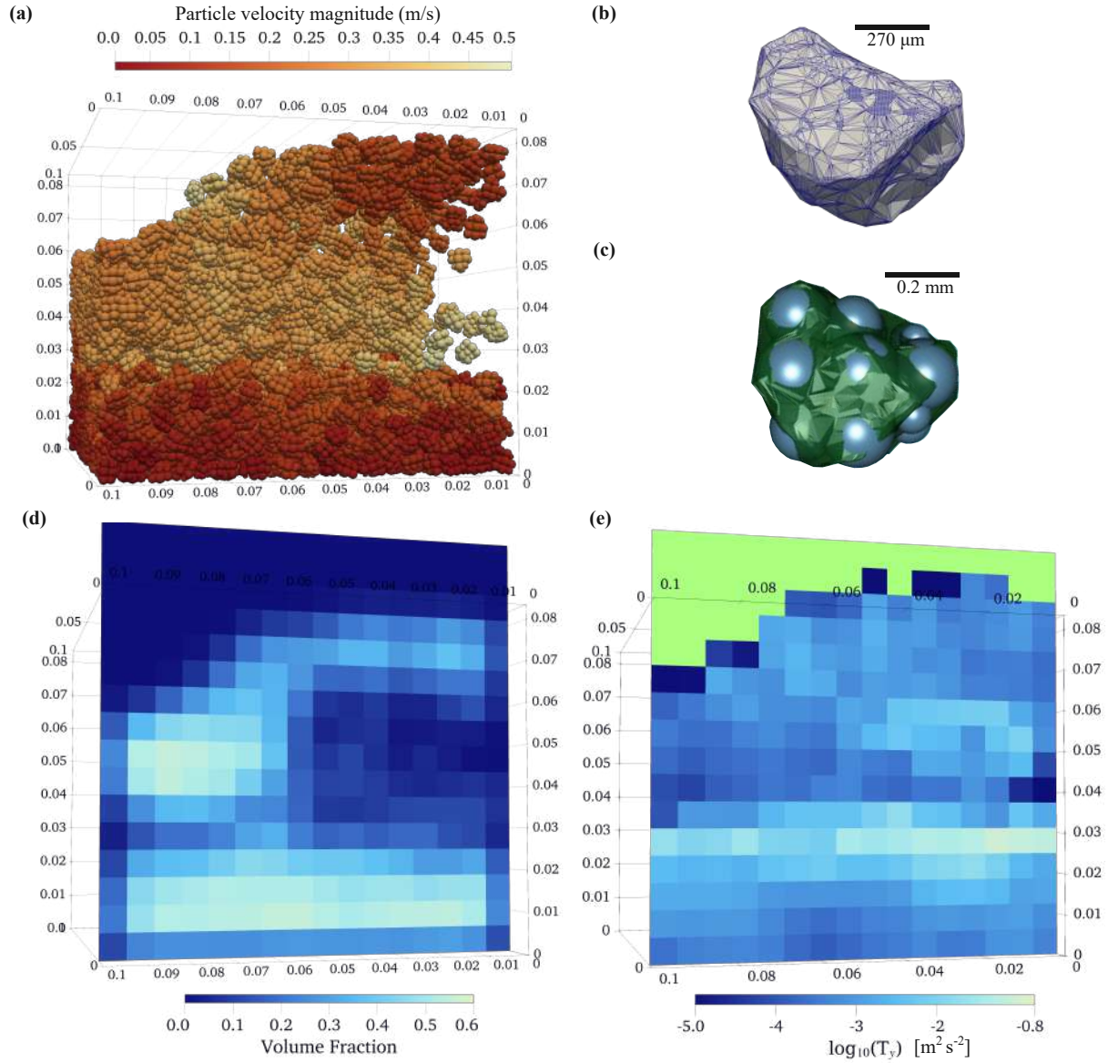
Figure 15. DEM simulation of a granular bed, fluidised bed with a gas velocity of 2 \text{ m s}^{-1} , using glued-sphere glued-sphere particles (a). Reconstructed ash particle shape from (Gabellini et al., 2025) (b), to which the glued-sphere glued-sphere particles in (a) are approximated to as shown in (c). Coarse-grained fields of the volume fraction (d) and vertical granular temperature (e) corresponding to the simulation time step shown in (a). Note that the greyish-pale green colour in (e) corresponds indicates NaN . This occurs at locations where T_y is set to T_y = 00 \text{ m}^2 \text{s}^{-2} by convention (see Appendix C2). Consequently, but cannot be \log_{10}(0) is undefined and is represented as NaN in log 10 scale ParaView.
