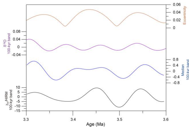
Figure 8. Comparison of the \chi_{fd} /HIRM and median grain-size records with the eccentricity and benthic oxygen isotope \delta^{18}\text{O} stack data. The \chi_{fd} /HIRM, median grain-size and benthic oxygen isotope \delta^{18}\text{O} stack data were filtered at the 100-kyr band.
