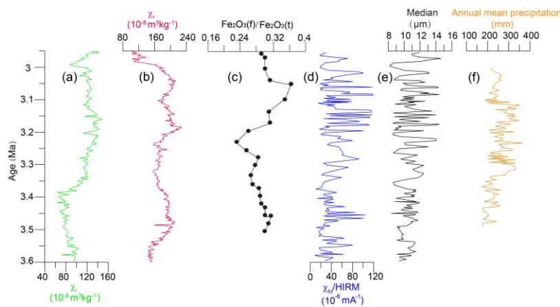
Figure 7. Comparison of the GS \chi_{lf} /HIRM and median grain-size records with the paleoclimatic records affected by the EASM precipitation during ~3.6–2.95 Ma. (a) Magnetic susceptibility at low frequency ( \chi_{lf} ) from the Chaona section (Song et al.,
