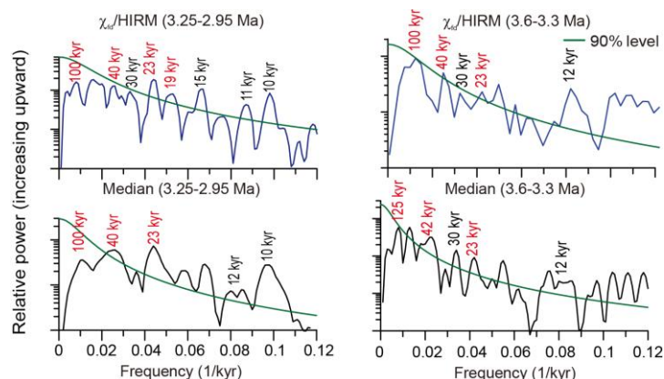
Figure 4. Results of spectral analyses of the reconstructed \chi_{fd}/\text{HIRM} and median grain-size records during \sim 3.6\text{--}3.3\text{ Ma} and the published \chi_{fd}/\text{HIRM} and median grain-size records during 3.25\text{--}2.95\text{ Ma} . The orbital cycles revealed by these two paleoclimatic records during 3.6\text{--}3.3\text{ Ma} passed the 90% confidence level.
