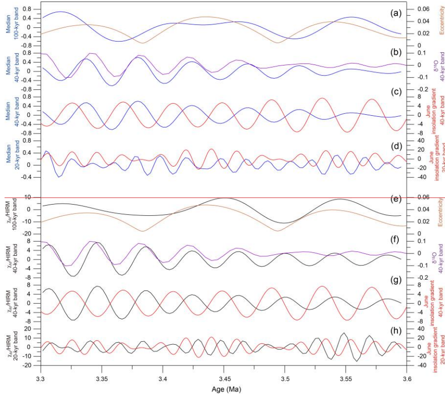
Figure 6. Comparison of the filtered \chi_{fd}/\text{HIRM} and median grain-size records from the GS section with the eccentricity, the filtered June insolation gradient and the filtered benthic \delta^{18}\text{O} stack during ~3.6-3.3 Ma. (a) and (e) \chi_{fd}/\text{HIRM} and median grain-size records at the 100-kyr band with eccentricity. (b) and (f) \chi_{fd}/\text{HIRM} , median grain-size and benthic \delta^{18}\text{O} stack at the filtered 40-kyr band. (c) and (g) \chi_{fd}/\text{HIRM} , median grain-size and June insolation gradient at the filtered 40-kyr band. (d) and (h) \chi_{fd}/\text{HIRM} , median grain-size and June insolation gradient at the filtered 20-kyr band. The 20-kyr central frequency = 0.05 \text{ kyr}^{-1} , and the bandwidth = 0.012 \text{ kyr}^{-1} . The 40-kyr central frequency = 0.024 \text{ kyr}^{-1} , and the bandwidth = 0.004 \text{ kyr}^{-1} . The 100-kyr central frequency = 0.01 \text{ kyr}^{-1} , and the bandwidth = 0.002 \text{ kyr}^{-1} .
