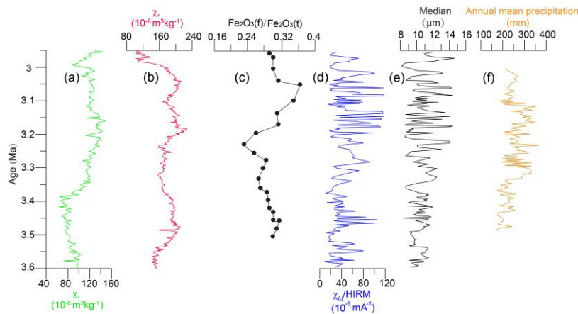
Figure 7. Comparison of the GS \chi_{ld} /HIRM and median grain size records with the paleoclimatic records affected by the EASM precipitation during 3.6–2.95 Ma. (a) Magnetic susceptibility at low frequency ( \chi_{lf} ) from the Chaona section (Song et al., 2001). (b) Magnetic susceptibility at low frequency ( \chi_{lf} ) from the Shilou section (Ao et al., 2016). (c) The ratio of free iron ( \text{Fe}_2\text{O}_3(\text{f}) ) to total iron ( \text{Fe}_2\text{O}_3(\text{t}) ) content of the Dianguan section (Yang et al., 2018). (d) GS \chi_{ld} /HIRM. (e) GS median grain size. (f) Annual mean precipitation variations based on the pollen records from the SG-1b core (Schwarz et al., 2022).
