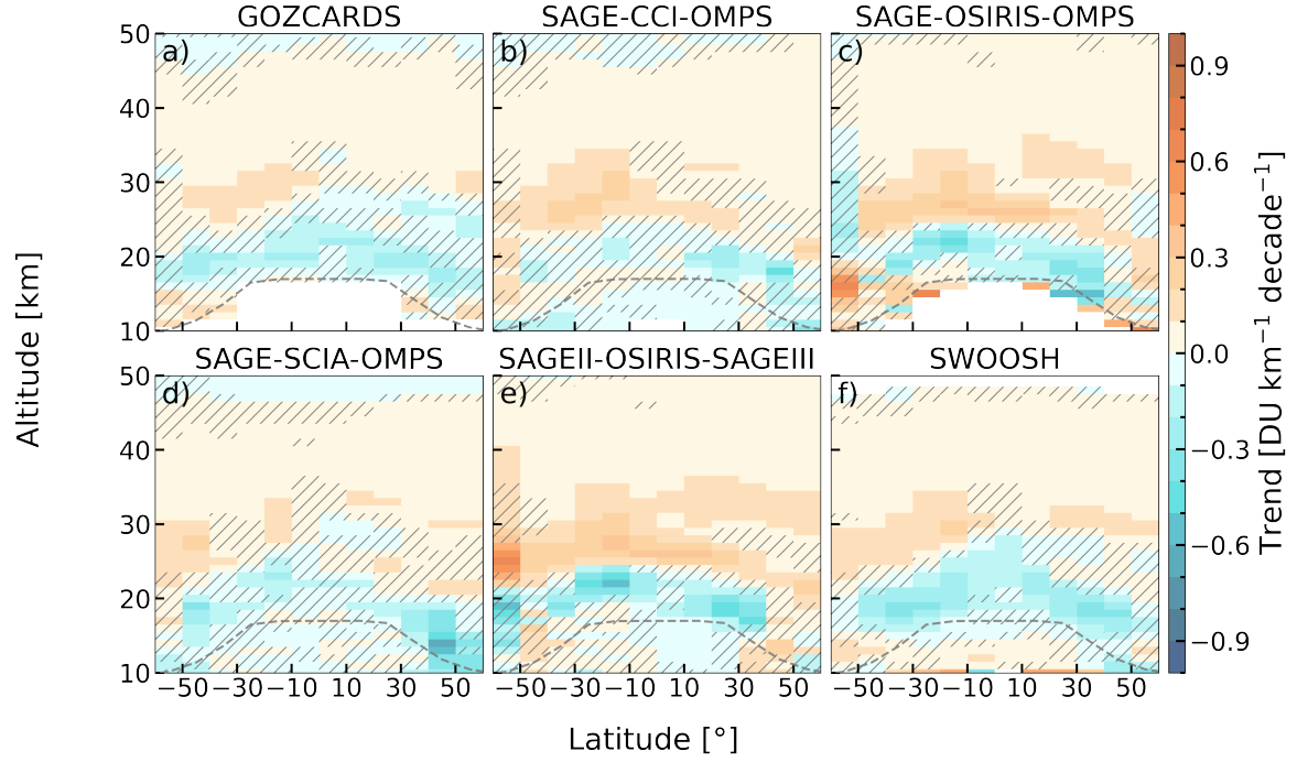
Figure A4. Profile ozone trends (LOTUS model) in \text{DU km}^{-1} per decade from 2000 to 2024 for the six profile ozone datasets (a) GOZCARDS, (b) SAGE-CCI-OMPS, (c) SAGE-OSIRIS-OMPS, (d) SAGE-SCIA-OMPS, (e) SAGEII-OSIRIS-SAGEIII, and (f) SWOOSH. Hatches indicate regions of no significance ( 2\sigma ). Same as Fig. 9, but using the LOTUS setup in the MLR.
