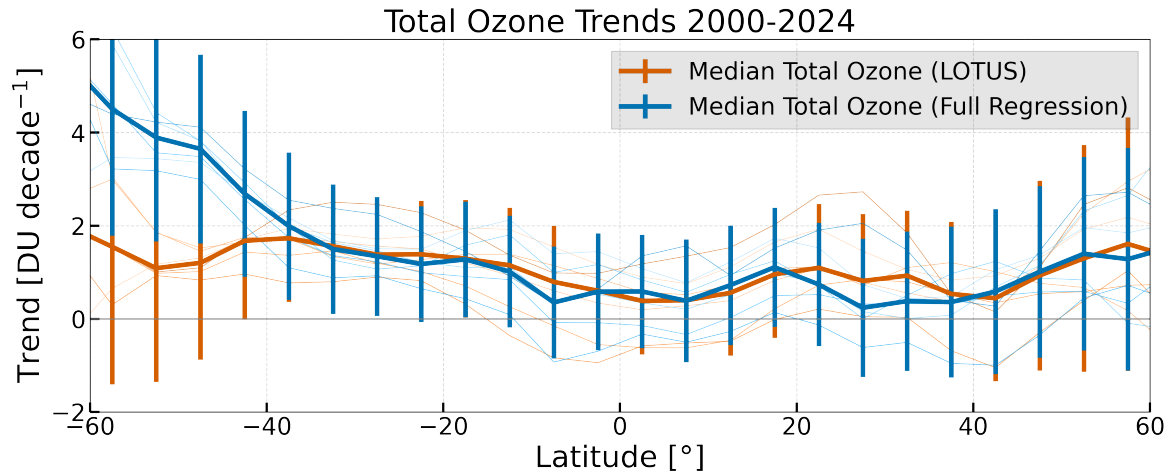
Figure 7. Total ozone trends in DU/decade from 2000 to 2024 for the six total ozone datasets WUODC, SBUV NASA (MOD), SBUV NOAA (COH), GSG, GTO-ECV, and MSR2 (thin lines) and the median and its 2\sigma uncertainty (thick line and error bars). Shown in blue are the MLR results with additional dynamical and SAOD proxies and in orange the LOTUS model setup.
