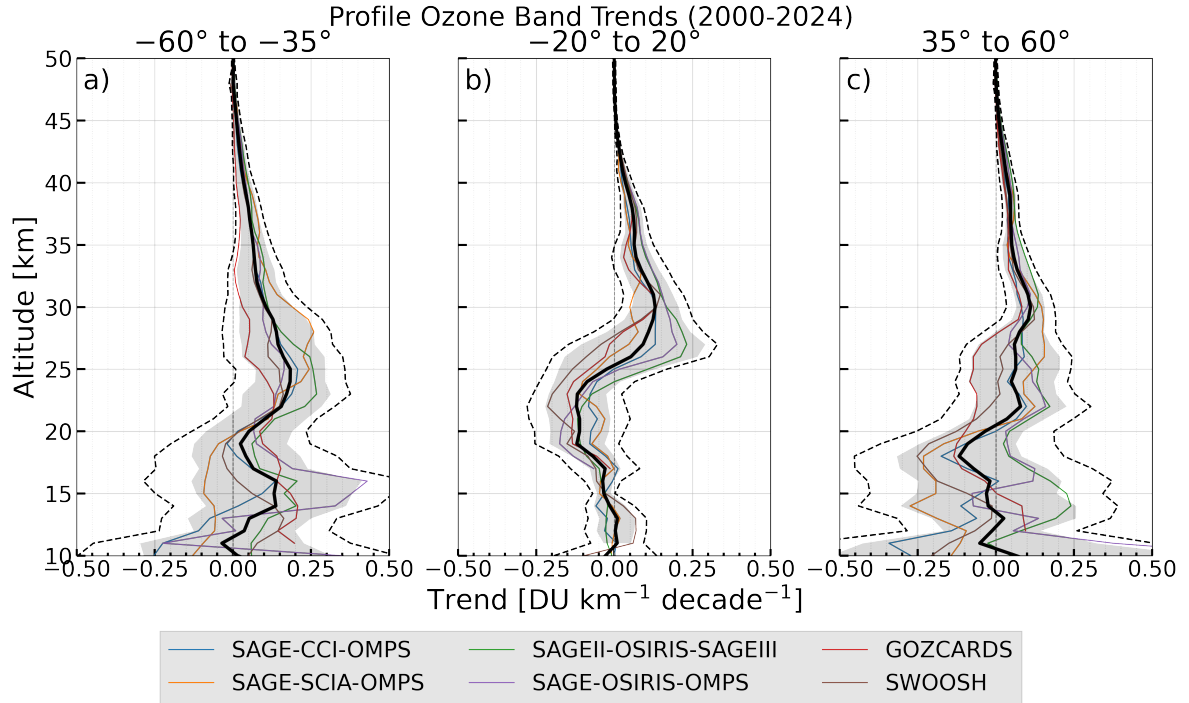
Figure 10. Ozone trends from 2000 to 2024 in three latitude bands ((a)35°S-60°S, (b) 20°S-20°N, (c) 35°N-60°N) in \text{DU km}^{-1} per decade for the six merged ozone profile datasets: GOZCARDS, SAGE-CCI-OMPS, SAGE-OSIRIS-OMPS, SAGEII-OSIRIS-SAGEIII, SAGE-SCIA-OMPS, and SWOOSH. Shaded area indicates the 2\sigma uncertainties of the mean trends (black line), calculated using the LOTUS uncertainty estimate described in Eq. 7 and the dashed line indicates the J-Distribution uncertainty described by Eq. 9.
