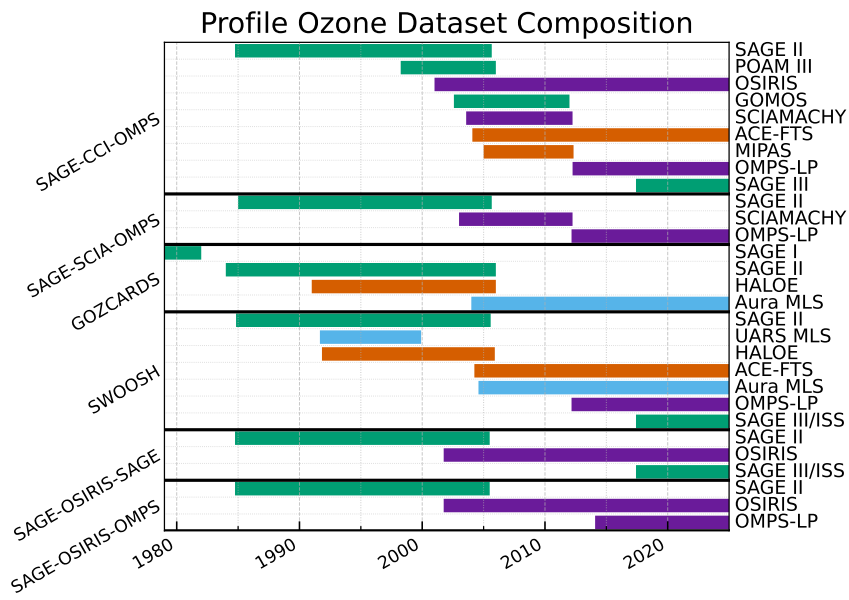
Figure 1. Satellite missions contributing to each of the six merged ozone profile datasets. The colors show the type of observation. Light blue instruments shown in light blue measure in the microwave region, those shown in green measure in the UV/Vis visible region, those shown in orange measure in thermal-infrared the thermal infrared region, and those shown in violet measure UV/visible limb-scatter instruments in violet limb scatter.
