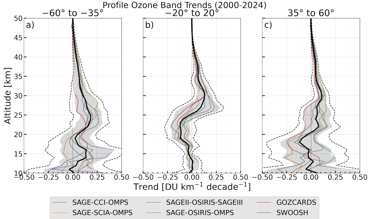
Figure 10. Ozone trends from 2000 to 2024 in three distinct broad latitude bands ((a) 35° S–60° S, (b) 20° S–20° N, (c) 35° N–60° N) in DU/km/km -1 per decade for the six merged ozone profile datasets: GOZCARDS, SAGE-CCI-OMPS, SAGE-OSIRIS-OMPS, SAGEII-OSIRIS-SAGEIII, SAGE-SCIA-OMPS, and SWOOSH. Shaded area indicates the 2 \sigma uncertainties of the mean trends (black line) , calculated using the LOTUS uncertainty estimate described in Eq. 7 and the dashed line indicates the J-Distribution uncertainty described in by Eq. 9 of the mean trends (black line) .
