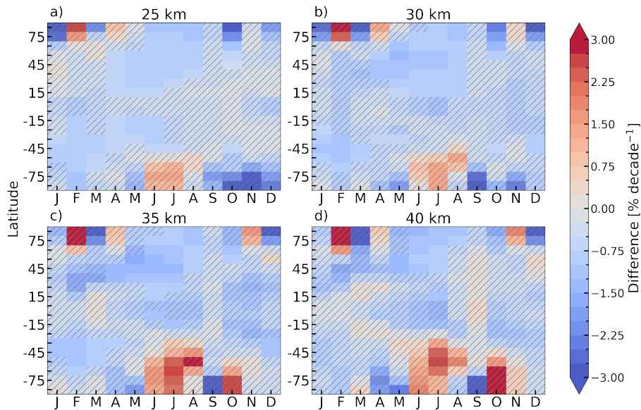
Figure 3. Zonal mean decadal trends of differences in %/decade from 2005 to 2022 between MLS L3 data converted after and before gridding ( post-gridded - pre-gridded ) in % per decade from 2005 to 2022 at altitudes of 25, 30, 35 and 40 km (panels a to d). Hatches indicate insignificant trends within 2\sigma .
