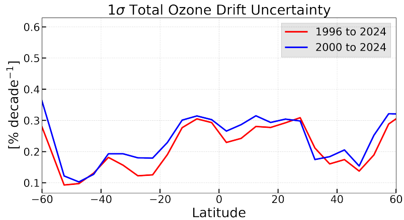
Figure 5. Standard deviation ( 1\sigma ) of the mean of the drifts ( 1\sigma ) derived from NASA SBUV, NOAA SBUV, GSG, GTO-ECV, and MSR2 total column data until 1995 and since 1996 (red line) and 2000 (blue line) as a function of latitude.
