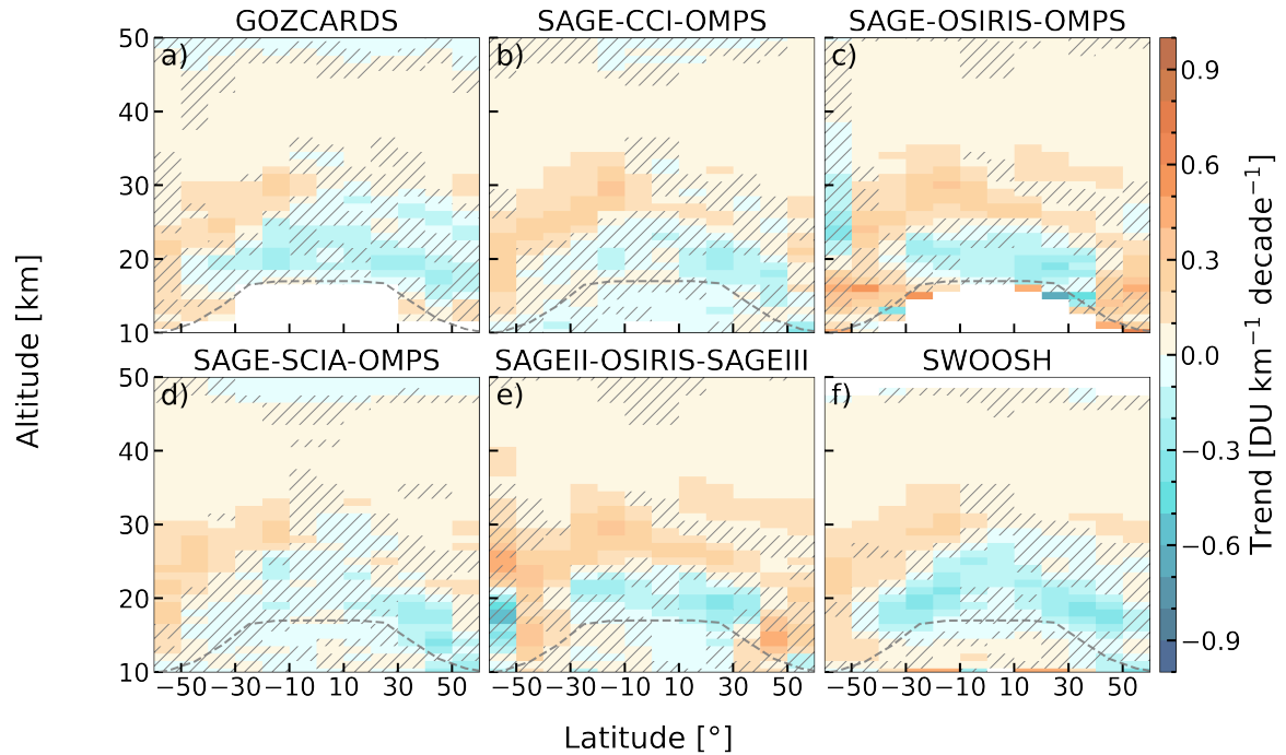
Figure 9. Profile ozone trends in \text{DU}/\text{km}/\text{km}^{-1} per decade from 2000 to 2024 from the six merged ozone datasets as a function of latitude and altitude: (a) GOZCARDS, (b) SAGE-CCI-OMPS, (c) SAGE-OSIRIS-OMPS, (d) SAGE-SCIA-OMPS, (e) SAGEII-OSIRIS-SAGEIII, and (f) SWOOSH. Hatched areas indicate regions of no significance ( 2\sigma ). Dashed lines are the climatological thermal tropopause derived from ERA5.
