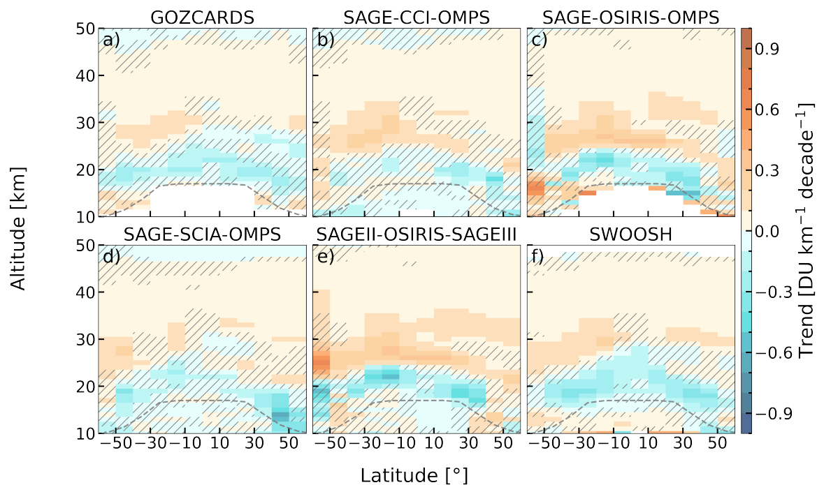
Figure A4. Profile ozone trends (LOTUS model) in DU/km/km -1 per decade from 2000 to 2024 for the six profile ozone datasets (a) GOZCARDS, (b) SAGE-CCI-OMPS, (c) SAGE-OSIRIS-OMPS, (d) SAGE-SCIA-OMPS, (e) SAGEII-OSIRIS-SAGEIII, and (f) SWOOSH. Hatches indicate regions of no significance (2σ). Same as Fig. 9, but using the LOTUS setup in the MLR.
