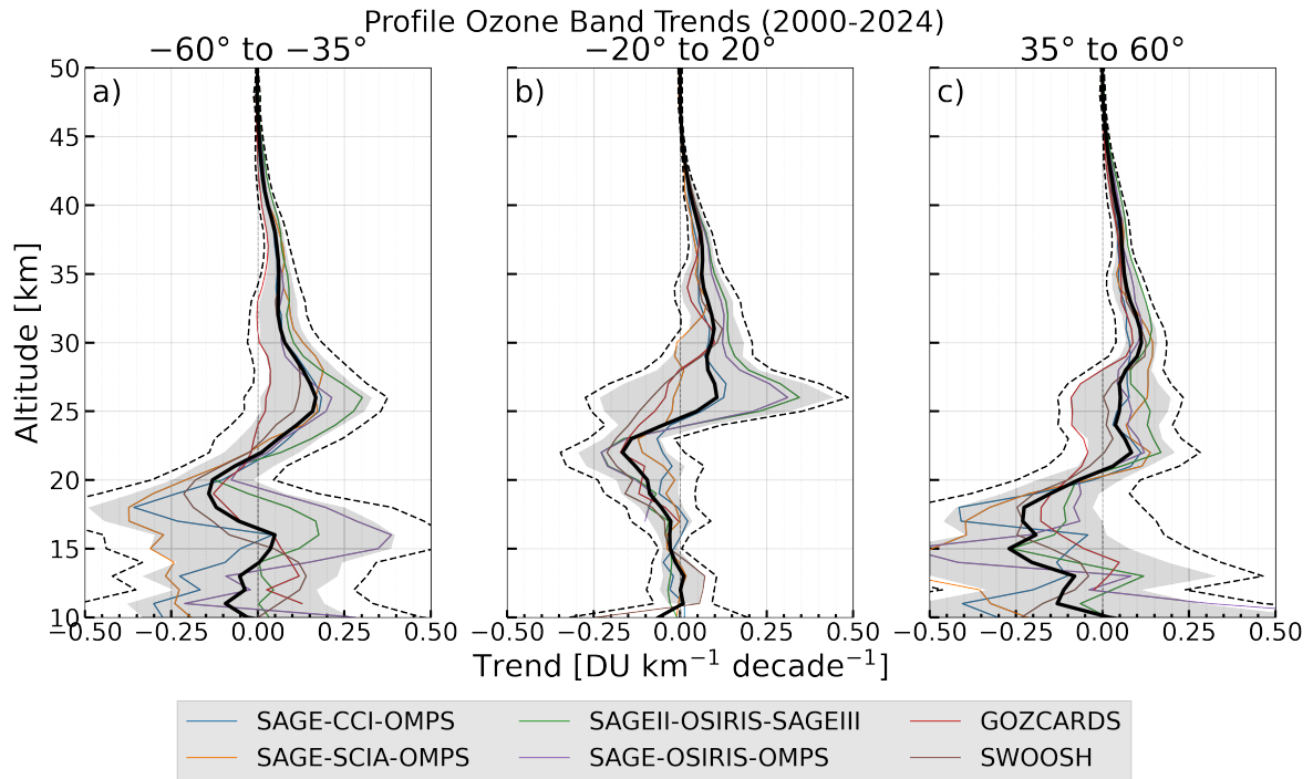
Figure A9. Ozone trends with the LOTUS Model from 2000 to 2024 in three distinct latitude bands ((a) 35°S-60°S, (b) 20°S-20°N, (c) 35°N-60°N) in DU/km/km -1 per decade for the six merged ozone profile datasets: GOZCARDS, SAGE-CCI-OMPS, SAGE-OSIRIS-OMPS, SAGEII-OSIRIS-SAGEIII, SAGE-SCIA-OMPS, and SWOOSH. Shaded area indicates the 2 \sigma uncertainties, calculated using the LOTUS (Eq. 7) and the dashed line indicates the J-Distribution uncertainty (Eq. 9) of the mean trends (black line). Same as Fig. 10, but using the LOTUS setup in the MLR.
