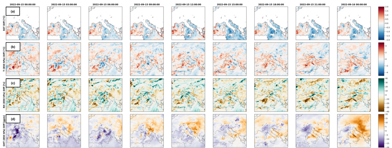
Figure S3. Spatiotemporal evolution of lower-tropospheric and surface differences between the driving forcing dataset (REF minus ECMWF) throughout the event. Rows from top to bottom shows differences in: (a) Sea Surface Temperature (°C), (b) 850 hPa temperature (°C), (c) 850 hPa relative humidity (%), and (d) 850 hPa geopotential height (gpm). Columns show the evolution at 3 h steps throughout the simulation.
