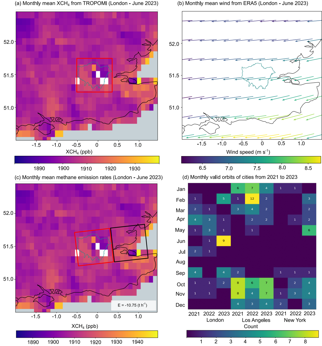
Figure 3. Illustration of the upwind background determination based on the improved source pixel method used in this study. (a) Mean \text{XCH}_4 retrievals derived from the TROPOMI instrument for London in June 2023. (b) Monthly mean wind vectors derived from hourly resolved ERA5 reanalysis data set for London in June 2023. (c) Location of the immediately adjacent upwind background region defined according to the wind direction shown in panel (b). (d) Monthly number of valid satellite overpasses for the three cities during 2021–2023 that passed strict quality control and were used in the final emission estimates.
