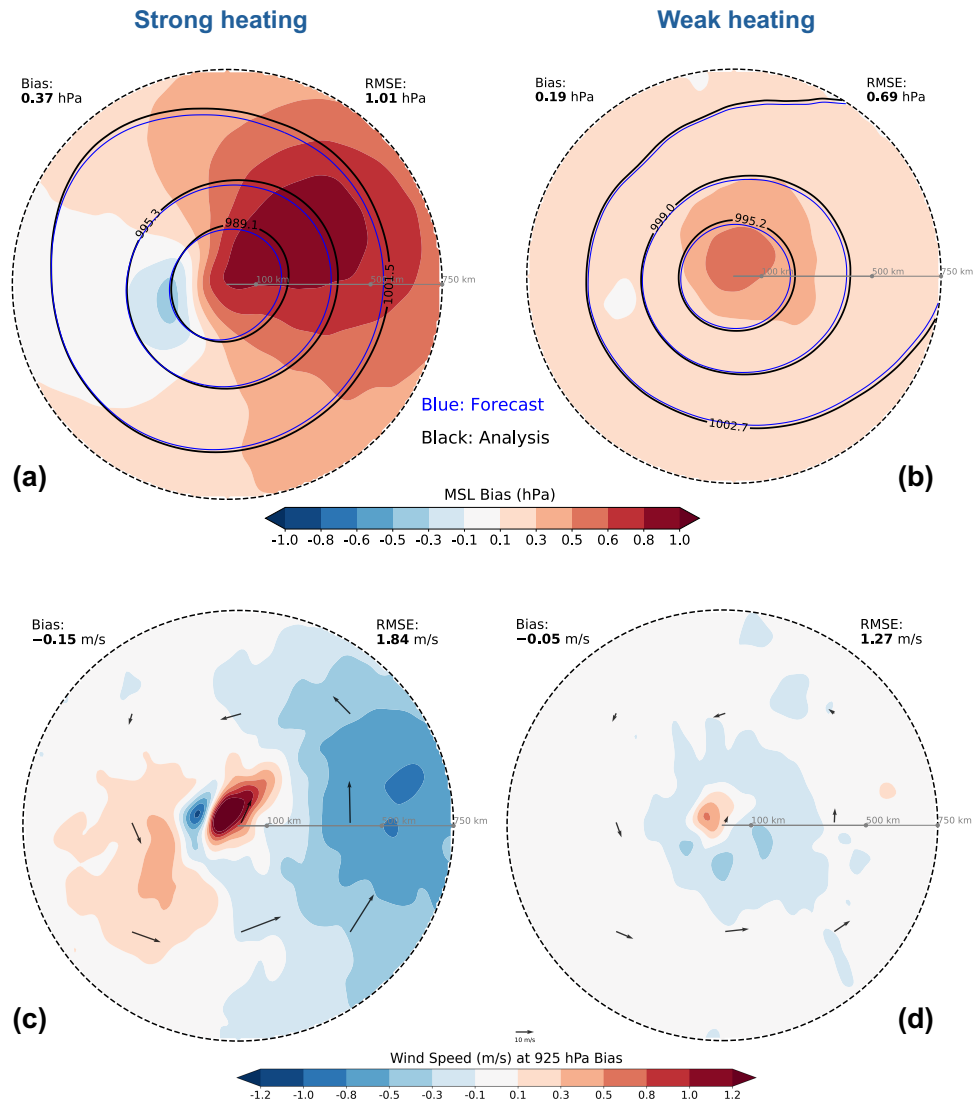
Figure 2. Biases for (a,c) strong heating group and (b,d) weak heating group: (a,b) mean sea level pressure (MSLP) (hPa) bias composite (shading), analysis composite (black contours), forecast composite (blue contours) and (c,d) wind speed bias (m/s) at 925 hPa (shading), black (blue) quivers show analysis (forecast) wind composite.
