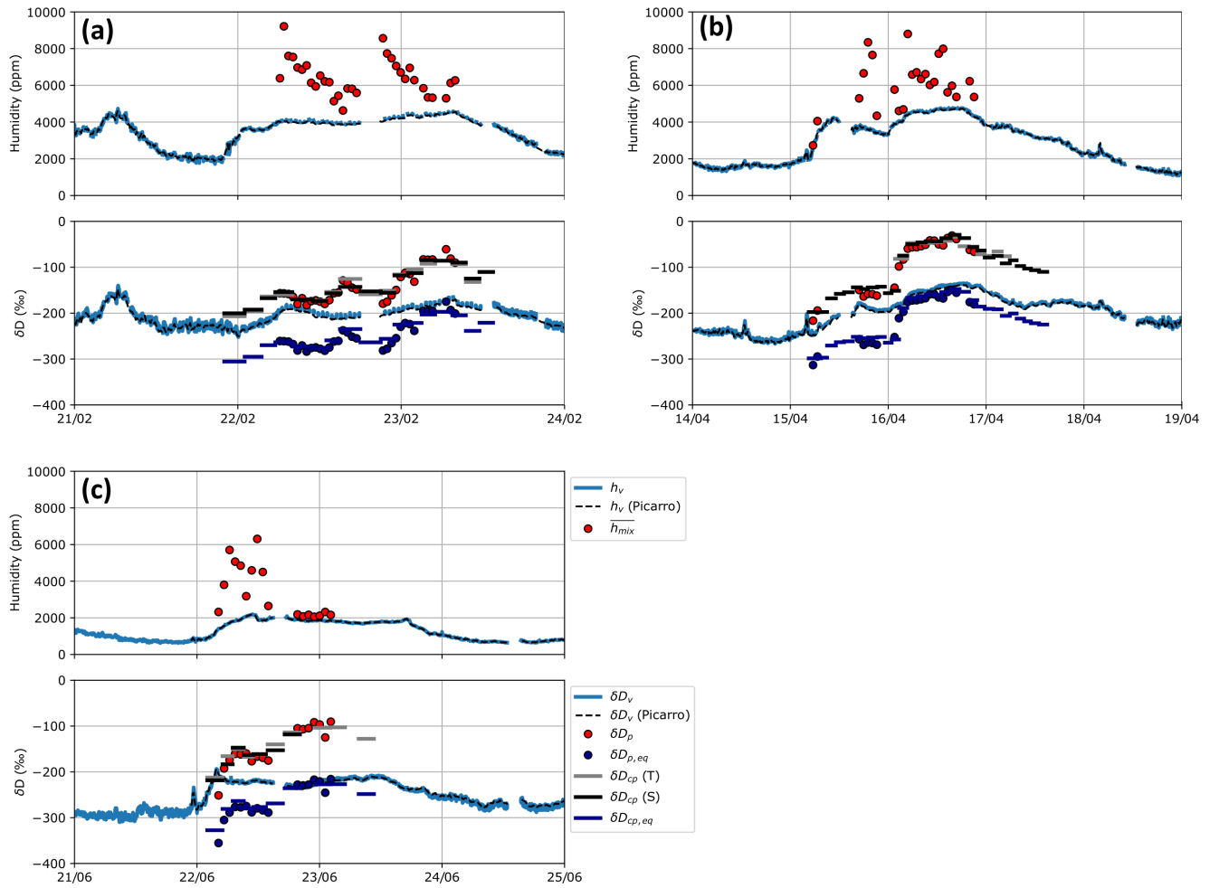
270 Figure 4: Isotopic measurements during the three selected precipitation events (a–c). Upper panels: water vapor mixing ratio from AP2E vapor inlet ( h_v , blue line), snowflake inlet ( \bar{h}_{mix} , red circles), and Picarro reference (black dashed line). Lower panels: \delta D of vapor ( \delta D_v , blue line), computed online \delta D of precipitation ( \delta D_p , red circles), \delta D of manually collected samples ( \delta D_{cp} , horizontal lines; black : sock, grey : tray; the length of the lines corresponds to the time between two sample collections) and Picarro reference 275 of \delta D_v (black dashed line). Darkblue circles and darkblue horizontal lines indicate the isotopic composition \delta D_{p,eq} and \delta D_{cp,eq} of a theoretical vapor that would be in equilibrium with the precipitation (section 4.2.2). The gaps in the curves correspond to periods of automatic instrument calibration.
