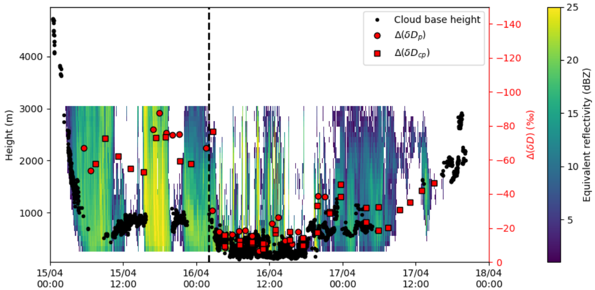
Figure 8: Combined view of in-situ isotope observations and remote sensing. Red circles (resp. squares) correspond to the \Delta(\delta D) calculated from online \Delta(\delta D_p) (resp. collected \Delta(\delta D_{cp}) ) precipitation; the black dots correspond to the ceilometer-derived cloud base height and the MRR equivalent reflectivity is plotted in background (color scale). Note that the \Delta(\delta D) axis is plotted on a reversed scale. The vertical dashed line separates the first and second parts of the event, situated on April 16 th at 03:00 UTC.
