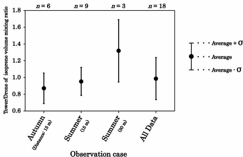
Figure 65: Ratios of isoprene volume mixing ratios measured simultaneously by the tower and drone at a 30 m height. Ratios are shown for the autumn observation at a 15 m horizontal distance, summer observations at 15 and 30 m horizontal distances, and all data combined. Points indicate average values, and error bars indicate \pm standard deviation.
