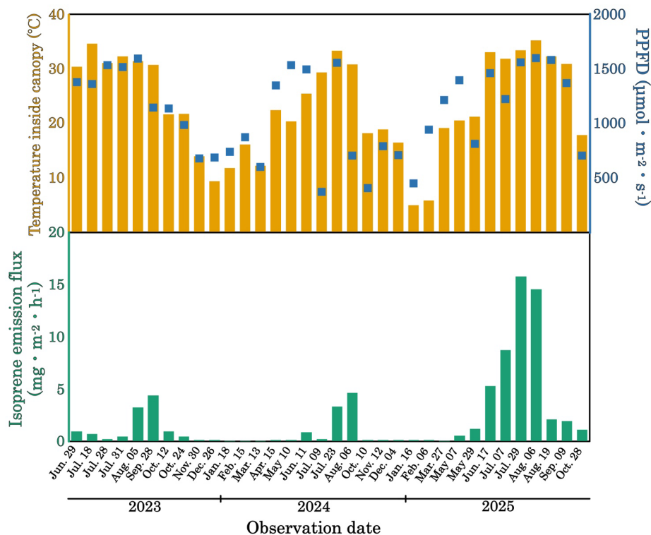
Figure 45: Daily average isoprene emission fluxes estimated from tower-based measurements (green bar graph), together with canopy temperature (orange bar graph) and PPFD (blue filled square) during the observation days from June 2023 to October 2025. Fluxes were calculated from the concentration gradient between 23 and 30 m using the aerodynamic gradient method.
