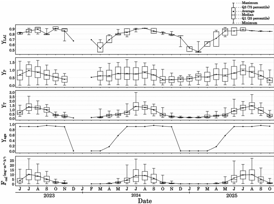
Figure 109: Monthly variation in the overlay of average values on the boxplots of MEGAN-calculated isoprene fluxes F_{cal} and the activity factors \gamma_{LAI} , \gamma_P , \gamma_T , and \gamma_{age} .
