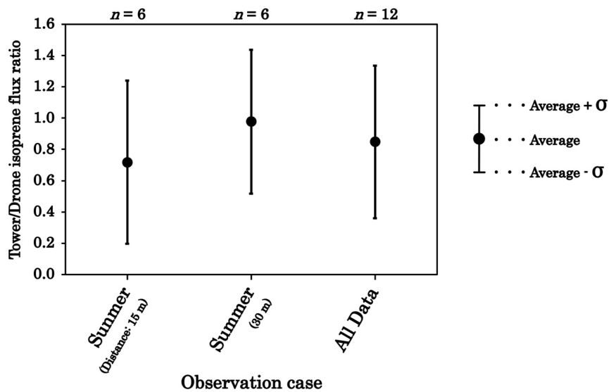
490 Figure 87: Ratios of tower-based and drone-based isoprene flux estimates during the supplemental drone experiment. Tower-based fluxes were calculated from the 23–30 m height interval, whereas drone-based fluxes were calculated from the 30–40 m height interval using tower-derived micrometeorological parameters. Points indicate average values, and error bars indicate \pm standard deviation.
