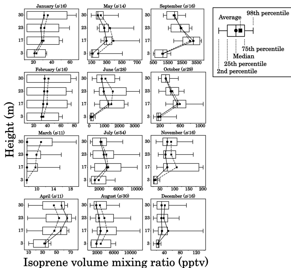
Figure 34: Boxplots overlaid with average values showing the monthly distribution of isoprene volume mixing ratios by height during the intermittent sampling campaign. The solid and dashed lines connect the median and average values for each height, respectively.
