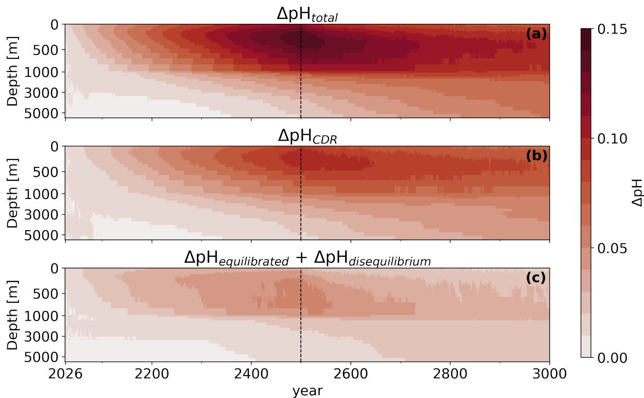
Figure 10. Hovmoeller plots of pH differences due to OAE over depth and time for the 2 °C scenario. The total pH change in (a), the pH response to CDR in (b) and the sum of the pH hysteresis – pH-equilibrated and p\text{CO}_2 disequilibrium effects in (c). All plots show the global horizontal averages, ensemble means until 2500 and the first ensemble member with OAE termination after 2500 (vertical dashed line). Note the irregular y-axis, with a break at 1000 m depth.
