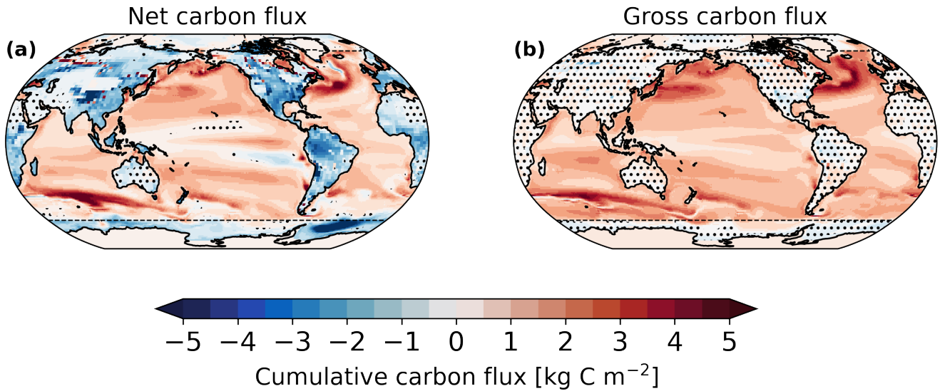
Figure 6. Spatial maps of cumulative net carbon fluxes (difference between OAE and Ref simulation) from 2026 to 2500 for the 2 °C warming scenario in (a) and the gross carbon fluxes (difference between OAE and Ref*) in (b). Colors-Positive indicates additional ocean carbon uptake. Colours show ensemble means and hatchings show differences that are not significant at the 95% confidence level based on a two-sided Students t-test. Dashed black lines mark the regions north of 70°N and south of 60°S, where alkalinity addition is not applied.
