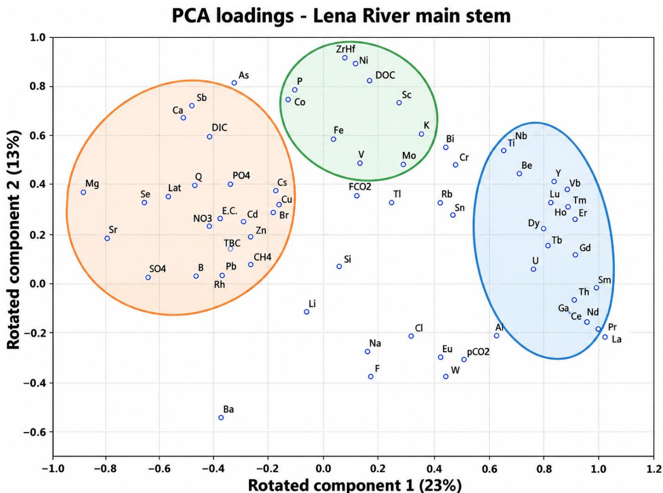
Fig. 7. Varimax-rotated PCA loading plot for standardized hydrochemical variables measured in the Lena River main stem ( n = 26 ). Rotated components 1 and 2 explain 23% and 13% of total variance, respectively (36% cumulative). Colored envelopes are visual guides to broad geochemical associations inferred from the loadings and independent geochemical evidence: orange, mobile weathering- and groundwater-related solutes; green, DOC, nutrients, and mixed surface-derived variables; blue, low-solubility lithogenic and colloid-associated elements. Overlap among envelopes and variables outside them emphasize that the ordination is exploratory and does not represent statistically discrete clusters.
