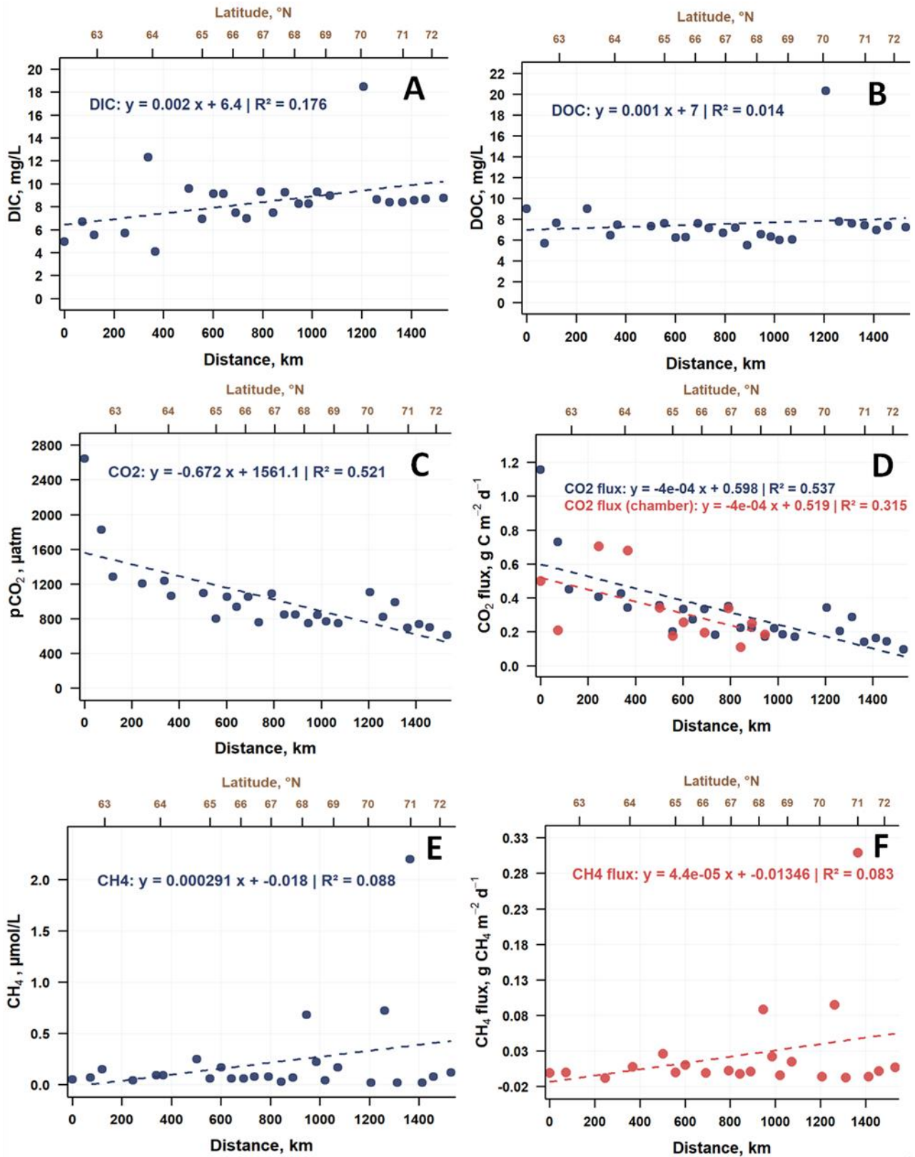
Fig. 2. Spatial variations of DIC (A), DOC (B), p\text{CO}_2 (C), \text{FCO}_2 (D), \text{CH}_4 concentration (E) and \text{FCH}_4 (F) in the main stem of the Lower Lena River, from Yakutsk to Kyusur. The dots represent discrete sampling points and dashed lines are linear regressions with equation parameters given on each panel.
