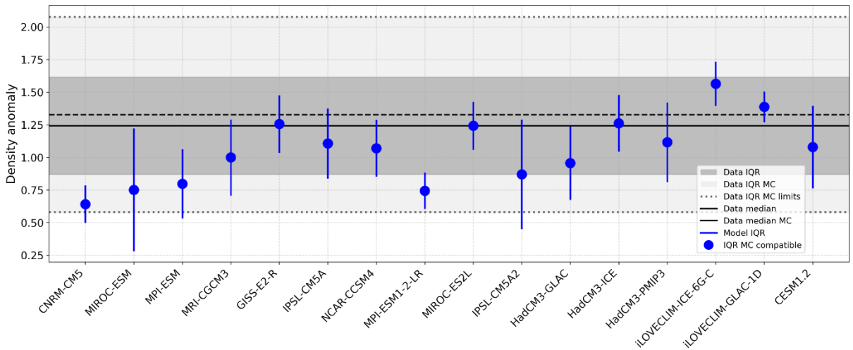
Figure 7: The dark grey band indicates the reconstructed IQR without considering uncertainties, while the light grey band and grey dotted lines indicate the Monte Carlo propagated reconstruction IQR after accounting for reconstruction uncertainty.
