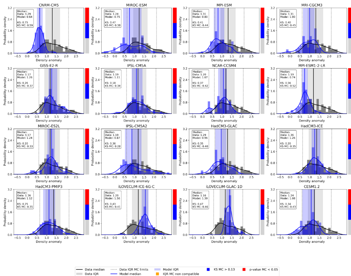
975 976 Figure C1: Distribution histograms of surface density anomalies (LGM-PI, kg/m 3 ) at the global scale. Density reconstructions 977 are shown in black, model simulations in blue. Kernel Density Estimates (KDEs) illustrate the central tendency and overall 978 shape of the distributions. Vertical lines indicate the median of each distribution, and shaded envelopes represent the 979 interquartile ranges (IQRs), providing a measure of data spread that is independent of extreme values. Grey dotted lines 980 indicate the limits of the Monte Carlo propagated reconstruction IQR obtained after accounting for the 95% confidence 981 intervals associated with the density reconstructions. The histograms display the frequency of values, complementing the 982 KDEs and IQRs to give an integrated view of distribution characteristics. Reconstructions uncertainties are explicitly 983 propagated through the Monte Carlo procedure. Colored indicators on the right side of each panel summarize the outcomes 984 of the three comparison metrics. A red flag indicates a Monte Carlo-derived two-sample KS test with p < 0.05 , a blue flag 985 indicates a Monte Carlo-derived KS statistic exceeding the global critical threshold ( KS > 0.13 ), and an orange flag indicates 986 non-overlapping Monte Carlo propagated IQRs between reconstructed and simulated distributions.
