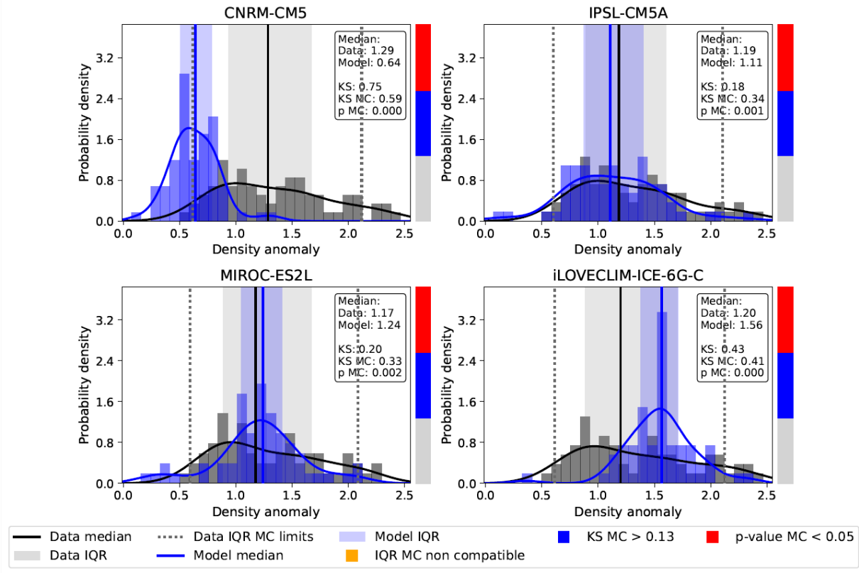
Figure 6: Distribution histograms of surface density anomalies (LGM-PI, kg/m 3 ) for an example of four model simulations. Density reconstructions are shown in black, model simulations in blue. Kernel Density Estimates (KDEs) illustrate the central tendency and overall shape of the distributions. Vertical lines indicate the median of each distribution, and shaded envelopes represent the interquartile ranges (IQRs), providing a measure of data spread that is independent of extreme values. Grey dotted lines indicate the limits of the Monte Carlo propagated reconstruction IQR obtained after accounting for the 95% confidence intervals associated with the density reconstructions. The histograms display the frequency of values, complementing the KDEs and IQRs to give an integrated view of distribution characteristics. Reconstructions uncertainties are explicitly propagated through the Monte Carlo procedure. Colored indicators on the right side of each panel summarize the outcomes of the three comparison metrics. A red flag indicates a Monte Carlo-derived two-sample KS test with p < 0.05 , a blue flag indicates a Monte Carlo-derived KS statistic exceeding the global critical threshold ( KS > 0.13 ), and an orange flag indicates non-overlapping Monte Carlo propagated IQRs between reconstructed and simulated distributions.
