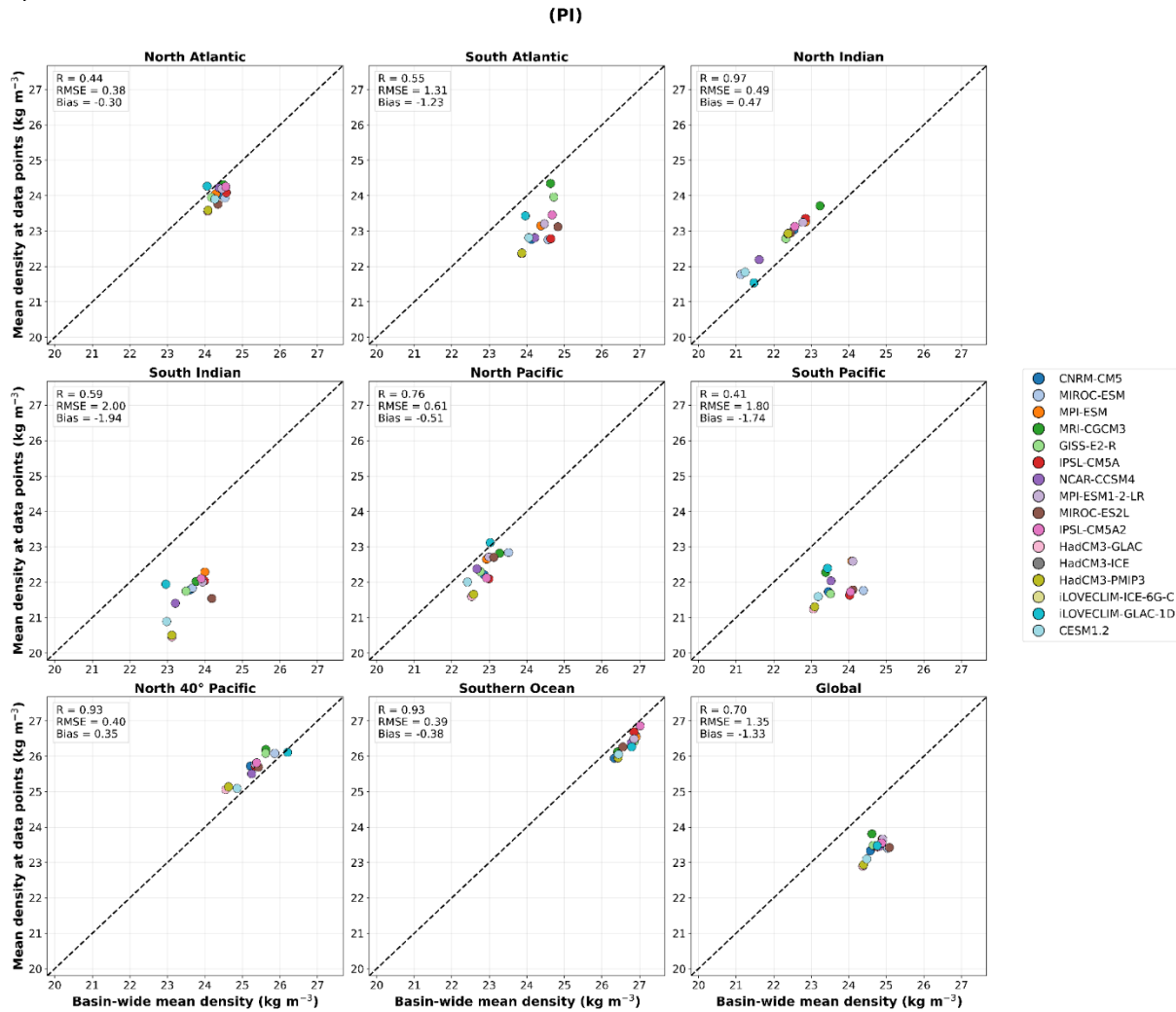
37 Figure S2: Pseudo-proxy test of the spatial representativeness of the proxy network for the LGM (a) and PI (b) ocean surface 38 density. For each ocean basin and for the global ocean, the mean density simulated by each climate model over all grid cells 39 within the basin (x-axis) is compared with the mean density obtained by sampling the same model only at the locations where 40 proxy reconstructions are available (y-axis). Each point represents one model simulation, and the dashed line indicates the 41 1:1 relationship. This pseudo-proxy approach does not involve proxy system modelling. Instead, it evaluates whether the 42 spatial distribution of proxy sites provides an unbiased estimate of the basin-scale density signal. Statistics shown in each 43 panel include the Pearson correlation coefficient (R), bias, and root mean square error (RMSE) between basin-wide model 44 means and model values sampled at proxy locations. A close agreement with the 1:1 line indicates that the proxy network 45 accurately captures the large-scale basin mean, whereas systematic departures reflect spatial sampling biases arising from 46 the uneven distribution of proxy records. The “Global” panel includes all proxy locations from the individual basins shown.
