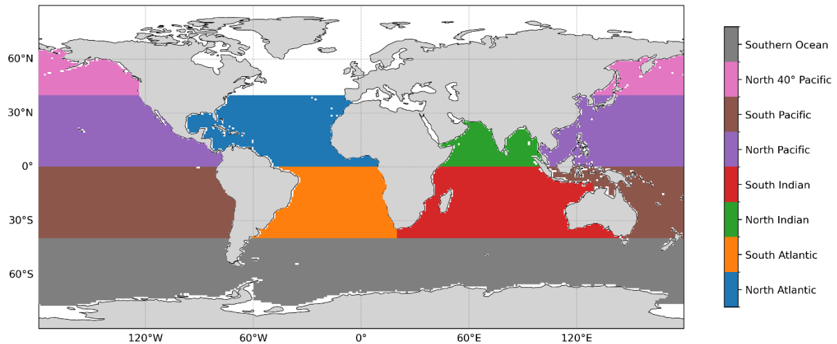
Figure A1: Map of selected basins in this study. The study basins were created from the NOAA WOA23 mask file (which has a 1°×1° grid) (website https://www.ncei.noaa.gov/data/oceans/woa/WOA23/MASKS/basinmask_01.msk ) then some basins were modified, in particular to divide them into North and South. 8 basins were defined and studied: North Indian (latitudinal limit at 0° S), South Indian (latitudinal limit at 40°S), North Atlantic (between 0° and 40° N), South Atlantic (latitudinal limit at 40°S), North Pacific, South Pacific, North Pacific with latitudes > 40°N, and Southern Ocean. North Atlantic is cropped at 40°N following the Caley et al. (2026) density-reconstruction method.
