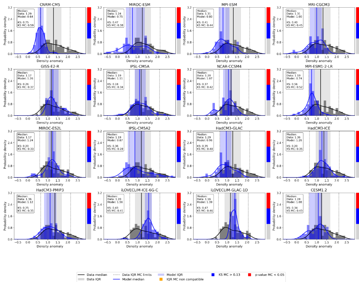
976 Figure C1: Distribution histograms of surface density anomalies (LGM-PI, kg/m 3 ) at the global scale. Density reconstructions 977 are shown in black, model simulations in blue. Kernel Density Estimates (KDEs) illustrate the central tendency and overall 978 shape of the distributions. Vertical lines indicate the median of each distribution, and shaded envelopes represent the 979 interquartile ranges (IQRs), providing a measure of data spread that is independent of extreme values. Grey dotted lines 980 indicate the limits of the Monte Carlo propagated reconstruction IQR obtained after accounting for the 95% confidence 981 intervals associated with the density reconstructions. The histograms display the frequency of values, complementing the 982 KDEs and IQRs to give an integrated view of distribution characteristics. Reconstructions uncertainties are explicitly 983 propagated through the Monte Carlo procedure. Colored indicators on the right side of each panel summarize the outcomes 984 of the three comparison metrics. A red flag indicates a Monte Carlo-derived two-sample KS test with p < 0.05 , a blue flag 985 indicates a Monte Carlo-derived KS statistic exceeding the global critical threshold ( KS > 0.13 ), and an orange flag indicates 986 non-overlapping Monte Carlo propagated IQRs between reconstructed and simulated distributions.
