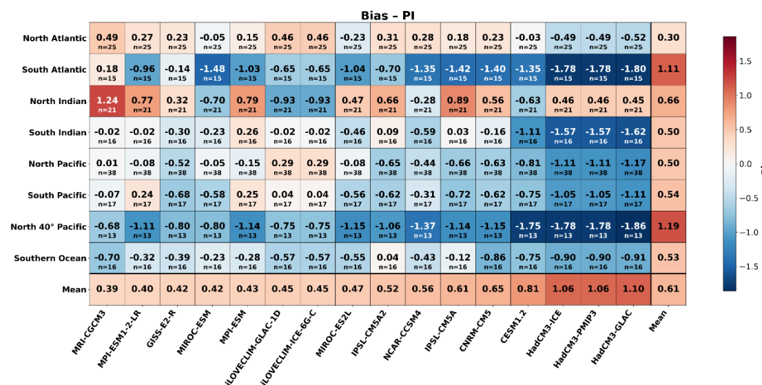
164 Figure S6: Weighted basin-scale mean density bias between simulated and reconstructed seawater density for the eight 165 ocean basins during a) the Last Glacial Maximum (LGM) and b) pre-industrial (PI). Rows correspond to ocean basins and 166 columns to climate model simulations. Individual cells show the mean bias (model – reconstruction) computed from grid 167 points common to all simulations and reconstructions within each basin. The number of valid grid points (n) is indicated 168 below each value. Models are ranked from left to right according to their weighted mean absolute bias, with lower values 169 indicating better agreement with the reconstructions. The final column and row (“Mean”) show weighted averages based 170 on the number of valid grid points in each basin. For these averages, absolute bias values are used to summarize model 171 performance independently of the sign of the error. Positive values indicate simulated densities that are higher than 172 reconstructed densities, whereas negative values indicate underestimation. The colour scale is centred on zero, with blue 173 colours representing negative biases and red colours representing positive biases.
