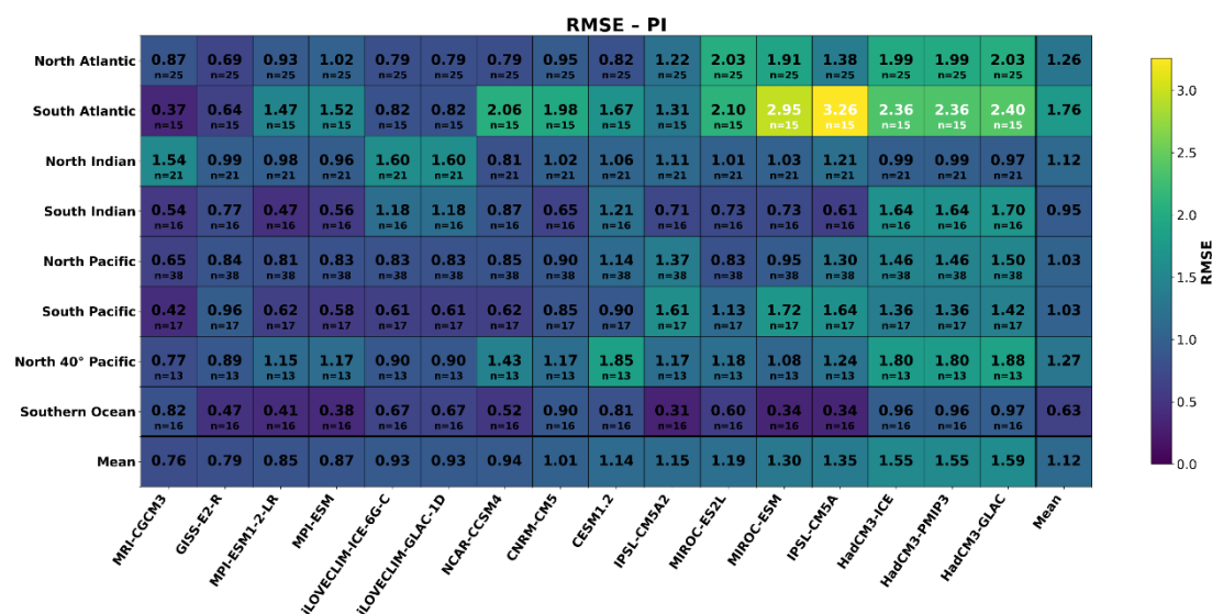
182 Figure S7: Weighted basin-scale root mean square error (RMSE) between simulated and reconstructed seawater density 183 for the eight ocean basins during a) the Last Glacial Maximum (LGM) and b) pre-industrial (PI). Rows correspond to ocean 184 basins and columns to climate model simulations. Individual cells show the RMSE calculated from grid points common to all 185 simulations and reconstructions within each basin. The number of valid grid points (n) is indicated below each value. Models 186 are ranked from left to right according to their weighted mean RMSE, with lower values indicating better agreement with the 187 reconstructions. The final column and row ("Mean") show weighted averages based on the number of valid grid points in 188 each basin. RMSE values are always positive and provide a measure of the overall magnitude of model–data mismatch, 189 combining both systematic and spatially varying errors. Lower RMSE values indicate a closer agreement between simulated 190 and reconstructed density patterns. Colours range from low errors (dark purple) to high errors (yellow).
