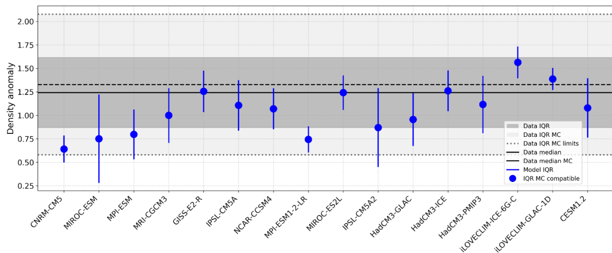
486 Figure 7: The dark grey band indicates the reconstructed IQR without considering uncertainties, while the light grey band and 487 grey dotted lines indicate the Monte Carlo propagated reconstruction IQR after accounting for reconstruction uncertainty.
