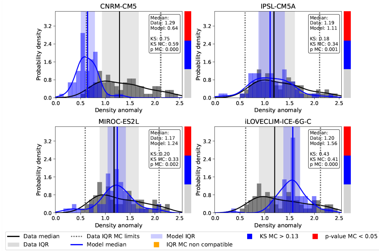
474 Figure 6: Distribution histograms of surface density anomalies (LGM-PI, kg/m 3 ) for an example of four model simulations. 475 Density reconstructions are shown in black, model simulations in blue. Kernel Density Estimates (KDEs) illustrate the central 476 tendency and overall shape of the distributions. Vertical lines indicate the median of each distribution, and shaded envelopes 477 represent the interquartile ranges (IQRs), providing a measure of data spread that is independent of extreme values. Grey 478 dotted lines indicate the limits of the Monte Carlo propagated reconstruction IQR obtained after accounting for the 95% 479 confidence intervals associated with the density reconstructions. The histograms display the frequency of values, 480 complementing the KDEs and IQRs to give an integrated view of distribution characteristics. Reconstructions uncertainties 481 are explicitly propagated through the Monte Carlo procedure. Colored indicators on the right side of each panel 482 summarize the outcomes of the three comparison metrics. A red flag indicates a Monte Carlo-derived two-sample KS test with p < 0.05 , 483 a blue flag indicates a Monte Carlo-derived KS statistic exceeding the global critical threshold ( KS > 0.13 ), and an orange flag 484 indicates non-overlapping Monte Carlo propagated IQRs between reconstructed and simulated distributions.
