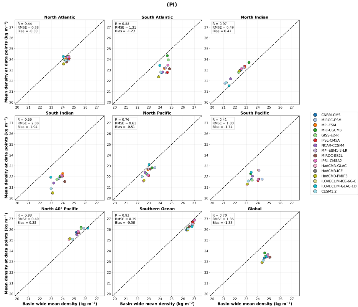
35 Figure S2: Pseudo-proxy test of the spatial representativeness of the proxy network for the LGM (a) and PI (b) ocean surface 36 density. For each ocean basin and for the global ocean, the mean density simulated by each climate model simulations over 37 all grid cells within the basin (x-axis) is compared with the mean density obtained by sampling the same model simulations 38 only at the locations where proxy reconstructions are available (y-axis). Each point represents one model simulation, and the 39 dashed line indicates the 1:1 relationship. This pseudo-proxy approach does not involve proxy system modelling. Instead, it 40 evaluates whether the spatial distribution of proxy sites provides an unbiased estimate of the basin-scale density signal. 41 Statistics shown in each panel include the Pearson correlation coefficient (R), bias, and root mean square error (RMSE) 42 between basin-wide model simulations means and model simulations values sampled at proxy locations. A close agreement 43 with the 1:1 line indicates that the proxy network accurately captures the large-scale basin mean, whereas systematic 44 departures reflect spatial sampling biases arising from the uneven distribution of proxy records. The "Global" panel includes 45 all proxy locations from the individual basins shown.
