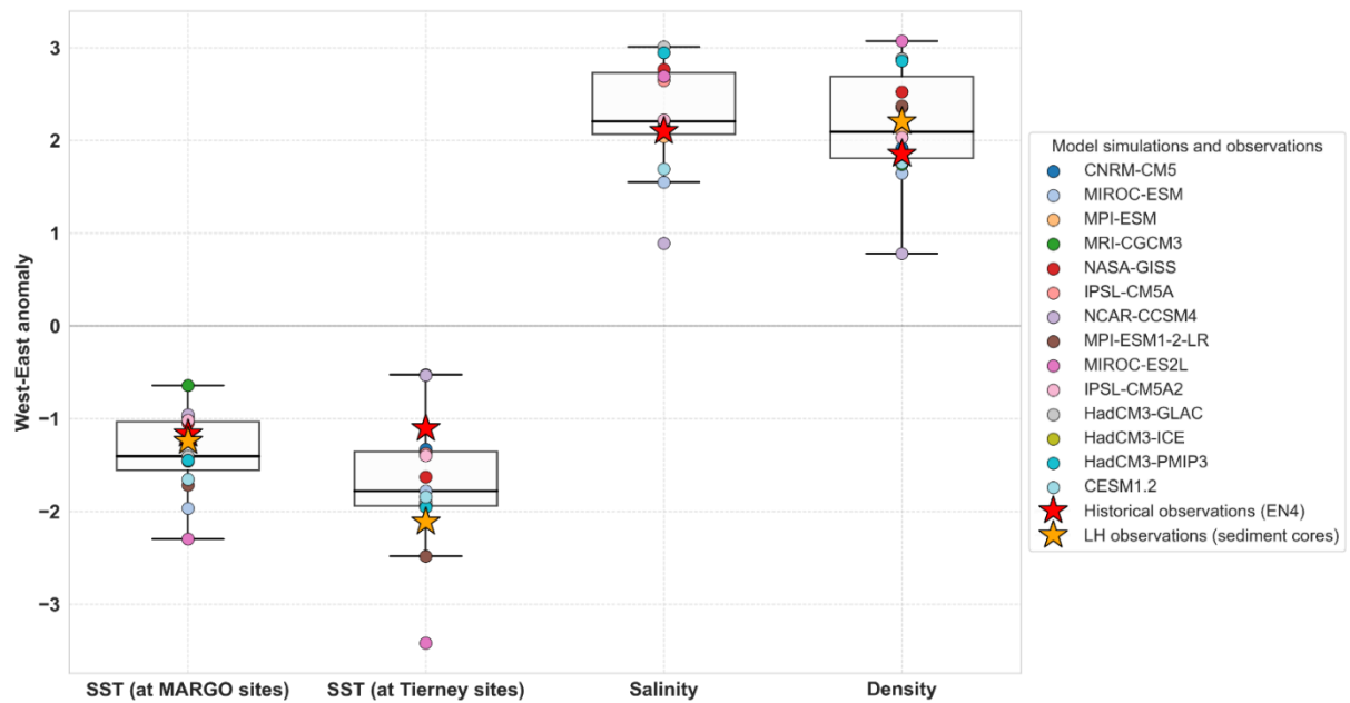
Figure E1: Boxplots showing West-East anomalies (Indian_East – Indian_West) in Sea Surface Temperature (°C), (from the MARGO and Tierney datasets, separately), Sea Surface Salinity (g/kg), and sea surface density (kg/m 3 ) during the pre-industrial period. The boxplots represent the distribution of anomalies from climate model simulations only. Each colored dot corresponds to the anomaly from an individual model simulation. Red stars indicate observed values from the EN4 dataset (Good et al., 2013), averaged over the period 1900–1999 to provide a historical reference. Orange stars indicate reconstructions from databases (PI from WOA18 for MARGO (MARGO project, 2009), LH for Tierney et al. (2020) and LH (Late Holocene) for density (Caley et al.2026)). The "Indian West" box is defined as 50°E-70°E, 12°S-12°N, corresponding to the tropical western Indian Ocean. The "Indian East" box is defined as 90°E-110°E, 10°S-2°N, corresponding to the tropical south-eastern Indian Ocean.
