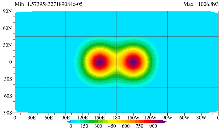
Figure S5. The initial condition of Gaussian hills test on the U60km mesh.
