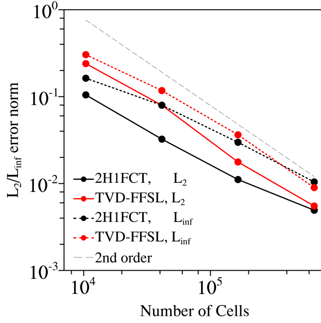
Figure 10. The L_2 and L_{\infty} error norms of the Gaussian hills under the Nair-Case2 deformational flow.
