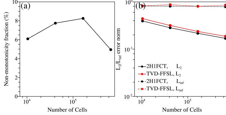
Figure 6. Evaluation of the TVD-FFSL solution for the slotted cylinder under the solid body rotation test. (a) The fraction of cells violating monotonicity in the TVD-FFSL solution, averaged over the first 4 days of the simulation. (b) The L_2 and L_{\infty} error norms of the 2H1FCT and TVD-FFSL solutions at t = T .
