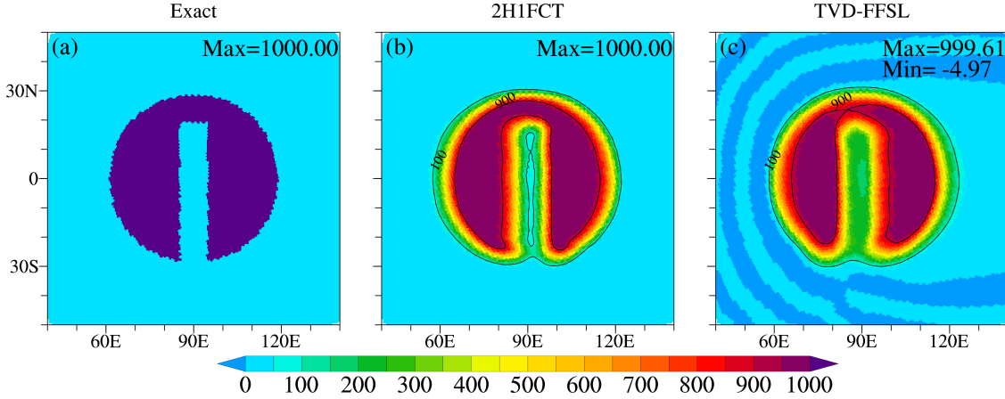
Figure S4. Slotted cylinder under the solid body rotation test on the U120km mesh at t = T . (a) Exact solution. (b) Result of the original 2H1FCT scheme in iAMAS. (c) Result of the TVD-FFSL hybrid scheme.
