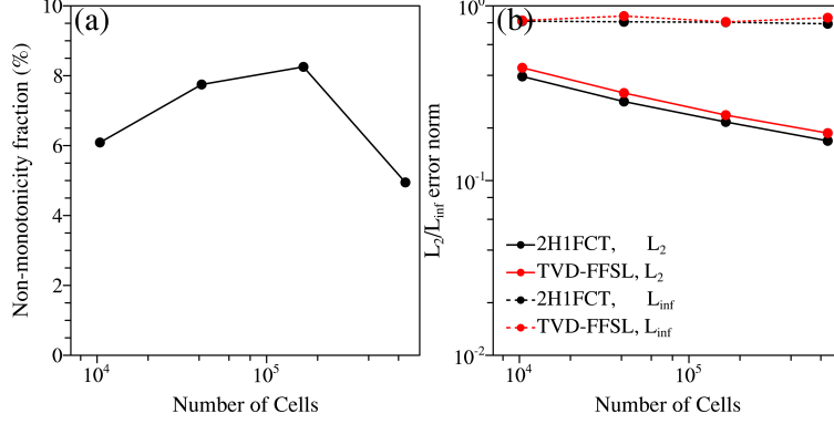
Figure 6. Evaluation of the TVD-FFSL solution for the slotted cylinder under the solid body rotation test. (a) The fraction of cells violating monotonicity in the TVD-FFSL solution, averaged over the first 4 days of the simulation. (b) The L_2 and L_{\infty} error norms of the 2H1FCT and TVD-FFSL solutions at t = T .
