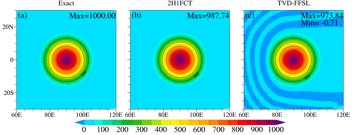
Figure 3. Cosine bell under the solid body rotation test on the U60km mesh at t = T . (a) Exact solution. (b) Result of the original 2H1FCT scheme in iAMAS. (c) Result of the TVD-FFSL hybrid scheme.
