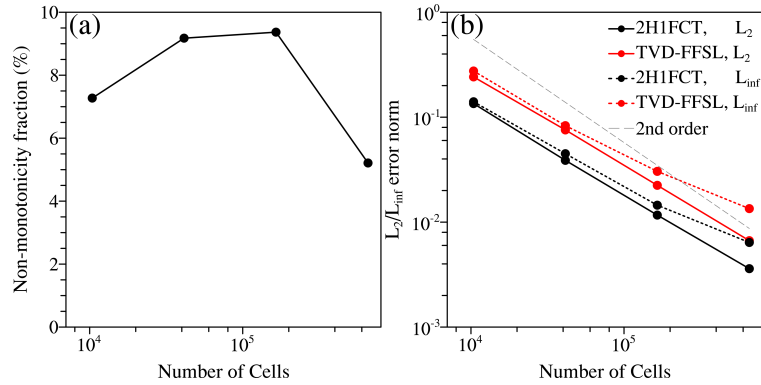
Figure 4. (a) The fraction of cells violating monotonicity in the TVD-FFSL solution, averaged over the first 4 days of the simulation. (b) The L_2 and L_{inf} error norms of the cosine bell under the solid body rotation test.
