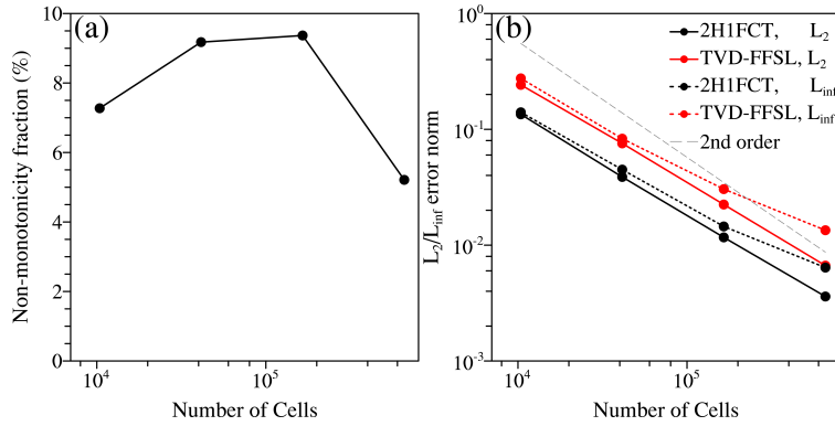
Figure 4. (a) The fraction of cells violating monotonicity in the TVD-FFSL solution, averaged over the first 4 days of the simulation. (b) The L_2 and L_{inf} error norms of the cosine bell under the solid body rotation test.
