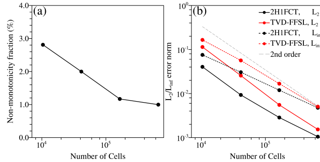
Figure 8. Evaluation of the TVD-FFSL solution for the cosine bell under deformational flow. (a) The fraction of cells violating monotonicity in the TVD-FFSL solution, averaged over the first 4 days of the simulation. (b) The L_2 and L_{\infty} error norms of the 2H1FCT and TVD-FFSL solutions at t = \frac{T}{2} .
