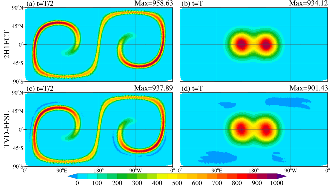
Figure S6. Gaussian hills under the Nair-Case2 deformational flow on the U120km mesh. (a-b) Results of 2H1FCT at t = \frac{T}{2}, T . (c-d) Results of TVD-FFSL at t = \frac{T}{2}, T .
