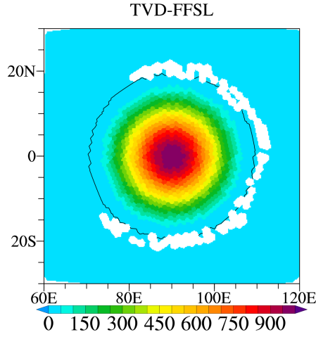
Figure S3. Initial distribution of the cosine bell (shaded) on the U120km mesh. Cells violating monotonicity in the solution after the first integration step are masked out (white). The black contour denotes the tracer value of 0.1.
