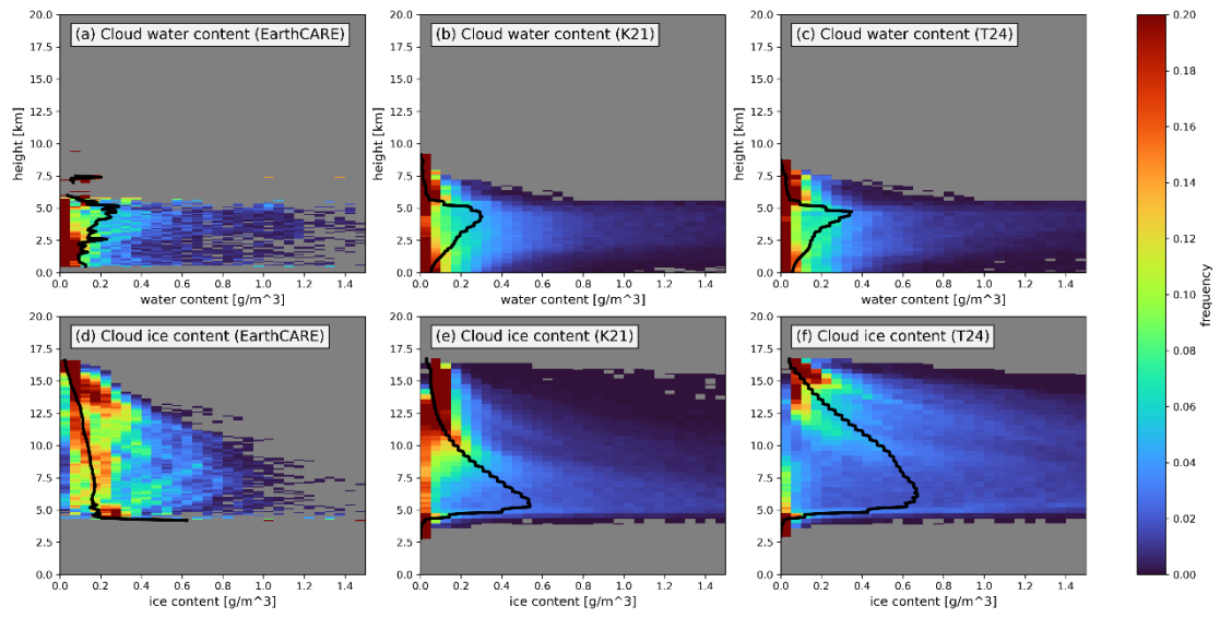
Figure S3. Same as Fig. 11, but all data within a 300 km radius are used to perform statistics for K21 and T24
