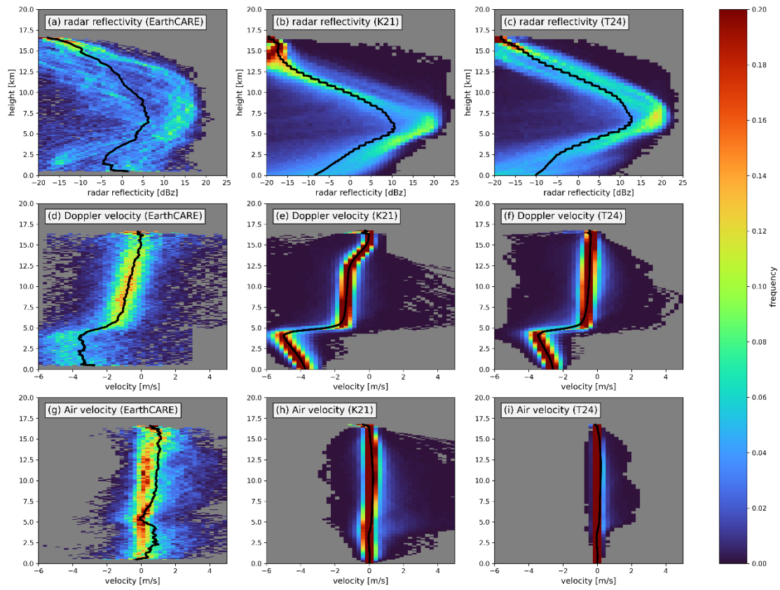
Figure S2. Same as Fig. 10, but all data within a 300 km radius are used to perform statistics for K21 and T24
