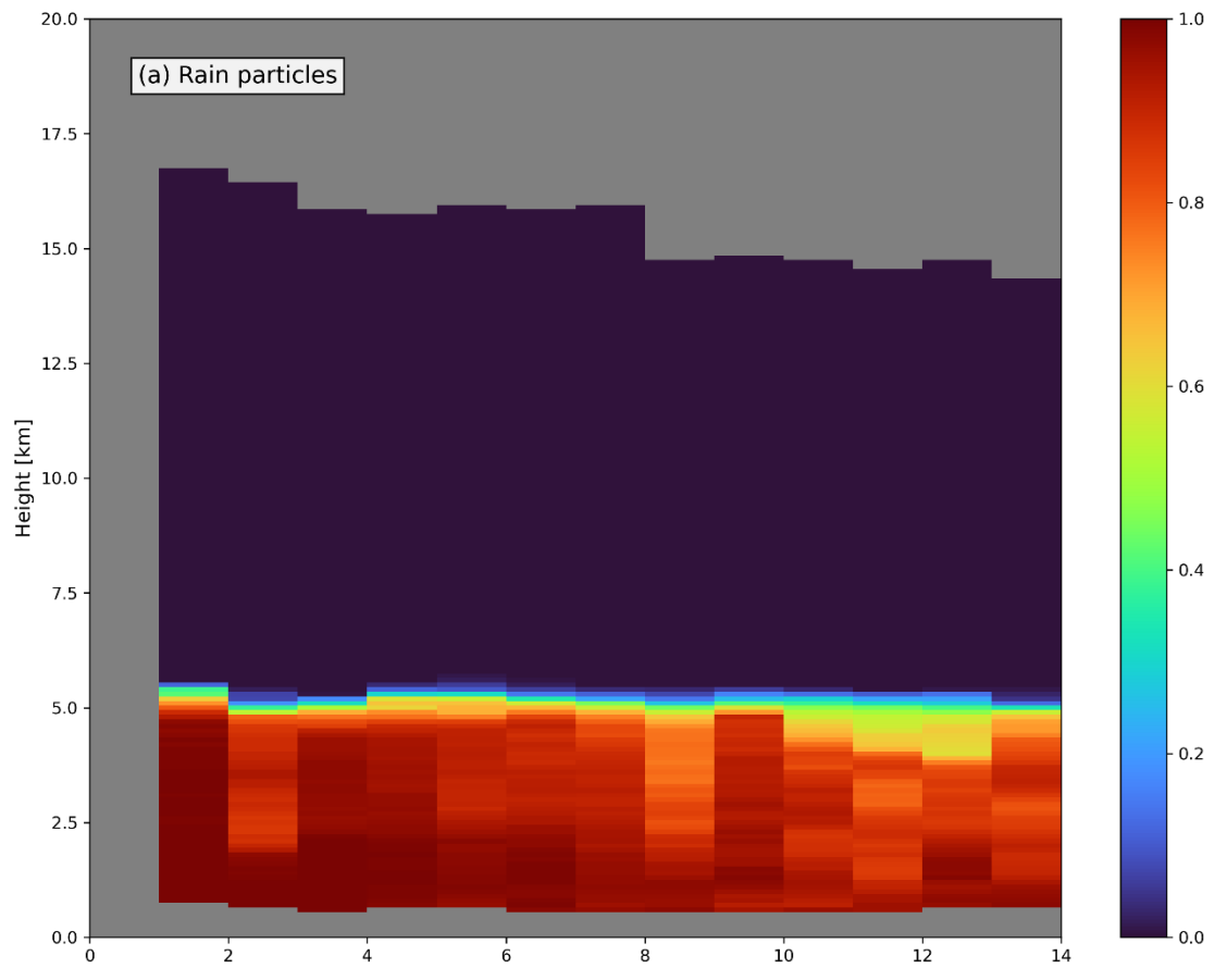
Figure S1. RMW-height frequency diagram of rain particles.
