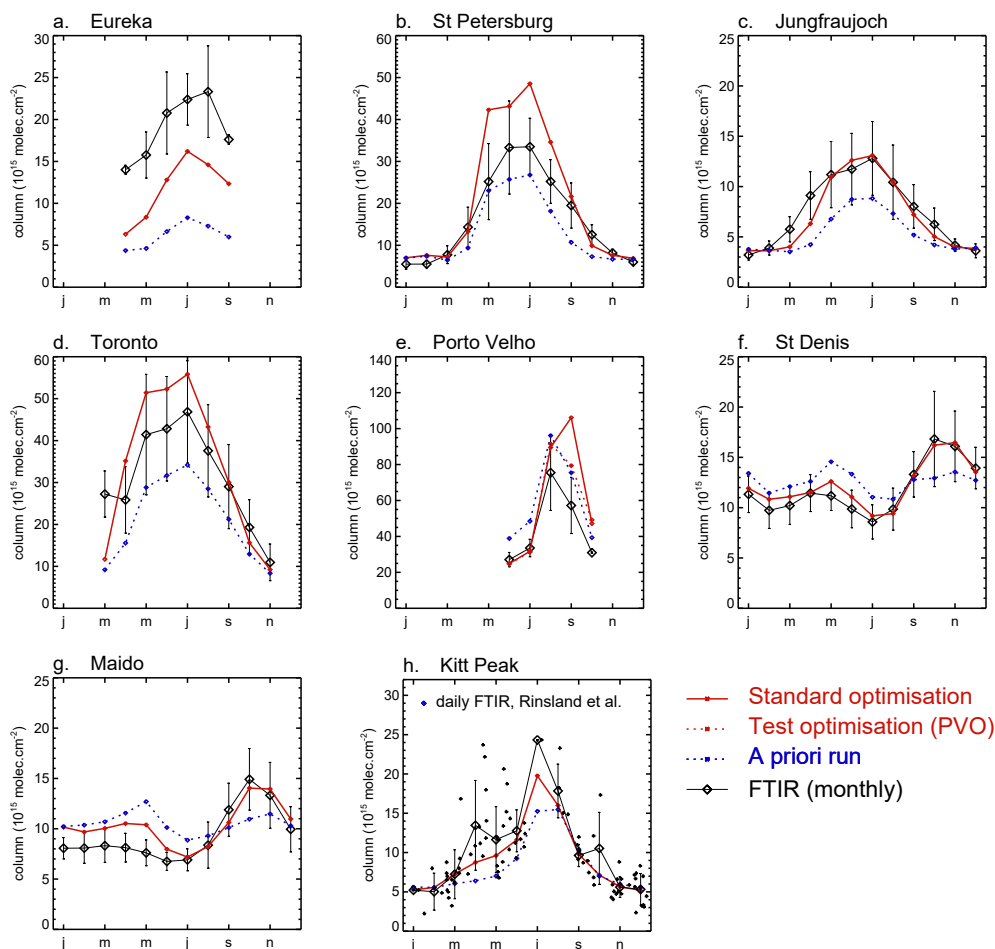
Figure 15. Monthly \text{CH}_3\text{OH} FTIR columns ( 10^{15} \text{ molec. cm}^{-2} ) averaged over 2008–2019 (black lines and diamonds) and corresponding averages from the a priori simulation (dotted blue) and optimised model (red) at (a) Eureka, (b) St Petersburg, (c) Jungfraujoch, (d) Toronto, (e) Porto Velho, (f) St Denis, and (g), Maïdo. The FTIR averaging kernels and sampling times are accounted for in the calculation of the model columns. The dotted red line in panel (e) denotes model columns from a test optimisation in which IASI data between 13 and 30 September 2019 were excluded. Panel (h) displays the average seasonal cycle of FTIR columns (2.09–14 km above sea level) recorded at Kitt Peak between 1985 and 2003 (Rinsland et al., 2009), compared with the 2008–2019 climatological average from the model. The daily FTIR averages (Fig. 5 of Rinsland et al., 2009) are also shown. The error bars denote the standard deviations of the monthly data.
