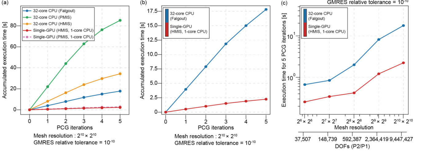
Figure 2. Execution time analysis of the SolCx benchmark in GPU and CPU environments. (a) Accumulated execution times on the GPU and 32-core CPU under different AMG preconditioner coarsening schemes (Falgout, PMIS, and HMIS). (b) Accumulated execution time on the single-GPU (HMIS) and 32-core CPU (Falgout). (c) Execution time for five preconditioned conjugate-gradient (PCG) iterations with increasing mesh resolution on the single-GPU (HMIS) and 32-core CPU (Falgout).
