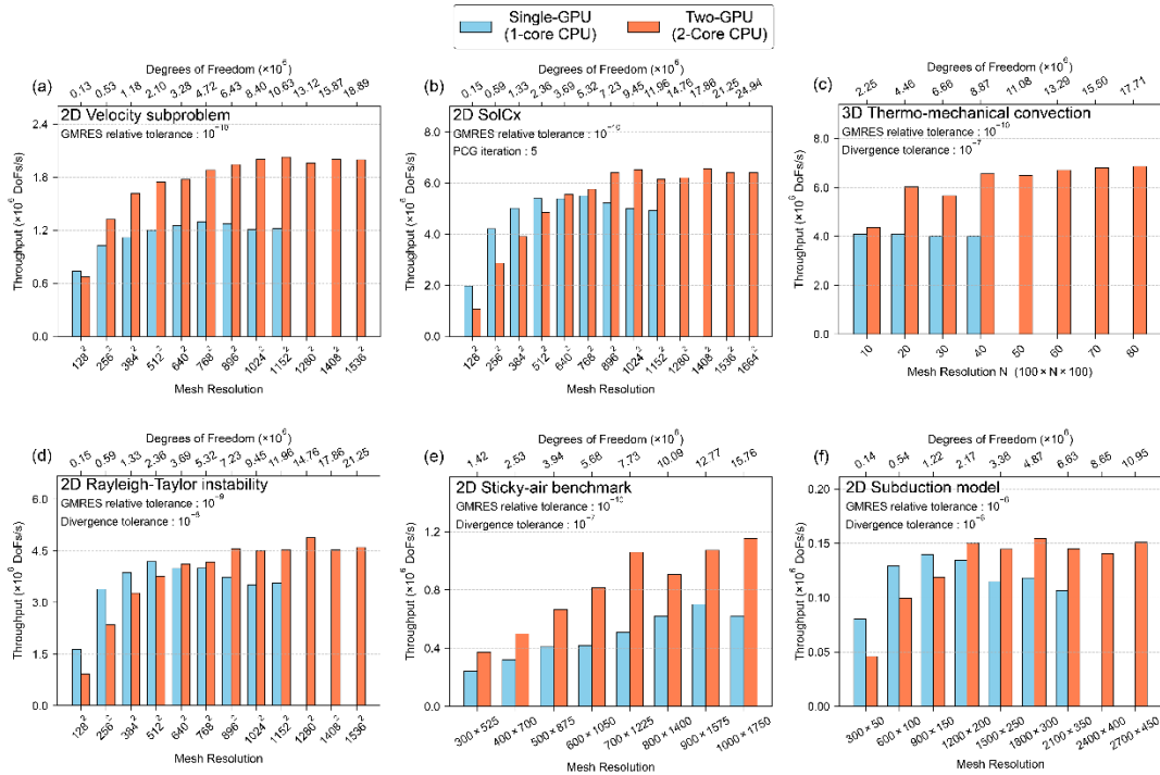
Figure 1412. Performance comparison between single-GPU with (1-core CPU) and two-GPU (2-core CPU) configurations in this study. (a)–(f) Comparison of execution time throughput for the velocity subproblem, SolCx, 3D thermo-mechanical convection, 2D/3D Rayleigh-Taylor instability, sticky-air benchmark, and subduction model, respectively. Horizontal axes represent mesh resolution and degrees of freedom; vertical axes represent execution time . Black arrows indicate crossover points where the two-GPU configuration begins to outperform the single-GPU setup as problem size increases. throughput (DOFs/s).
