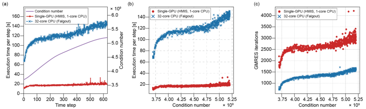
Figure 13.11. Analysis of GPU performance and matrix condition number for subduction modelling. (a) Evolution of the condition number and corresponding changes in execution time for single-GPU (HMIS) with 1-core CPU and 32-core CPU (Falgout) over elapsed time. (b) Correlation between the matrix condition number and execution time per step for the subduction model. (c) Correlation between the matrix condition number and inner GMRES iterations per step for the subduction model. (d) Wall time for 30 time steps under four processor configurations: two GPU with 16-core CPU, single GPU with 16-core CPU, single GPU with 1-core CPU, and 32-core CPU (CPU only).
