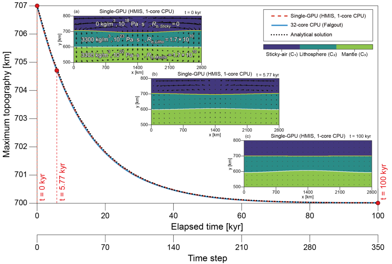
Figure 108. Evolution of maximum topography in the sticky-air benchmark. The solid blue dashed red line denotes the single-GPU (HMIS) with 1-core CPU, the dashed red solid blue line denotes the 32-core CPU computation, and the dotted black line denotes the analytical solution. Panels (a), (b), and (c) correspond to Temporal evolution of the compositional fields field at t=0 t=0 , 5.77, and 100 kyr, respectively, obtained from the single-GPU (HMIS) with, 1-core CPU. The temporal evolution of maximum topography indicates close agreement between the GPU and CPU computations and with the analytical solution.
