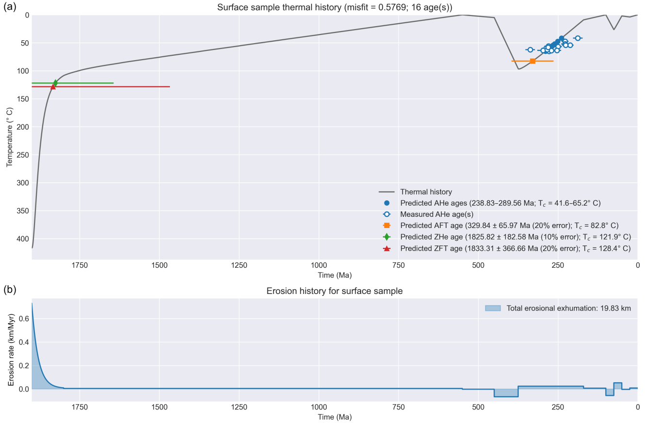
Figure 7. Thermal history, predicted thermochronometer ages, and exhumation history for Slave Craton, Canada. (a) The cooling history (dark gray line) shows initial rapid cooling followed by protracted slow cooling and several reheating and cooling events. Burial and re-heating from 450–375 Ma heats the tracking particle to temperatures sufficient to reset the apatite (U-Th)/He and fission-track thermochronometers (blue and orange symbols). Measured apatite (U-Th)/He ages (blue symbols with white fill) are quite similar to the predicted ages for this example, as reflected by the low model misfit ( <1 ). Note that the misfit calculated here uses Equation 4, the default for forward models in T_c 1D. Measured age data from Ault et al. (2009). (b) Burial and exhumation history corresponding to the thermal history in (a).
