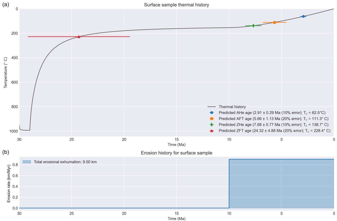
Figure 5. Thermal history, predicted thermochronometer ages, and exhumation history for the pluton emplacement example. (a) The cooling history (dark gray line) shows rapid cooling after pluton activity ceases followed by a period of slow cooling prior to moderate cooling during exhumation from 10–0 Ma. Predicted thermochronometer ages (colored markers) generally correspond to the late stage of exhumation, except the older ZFT age that records post-magmatic cooling. (b) The exhumation history shows no activity from 30–10 Ma followed by exhumation at a constant rate of 0.9 mm/yr from 10–0 Ma.
