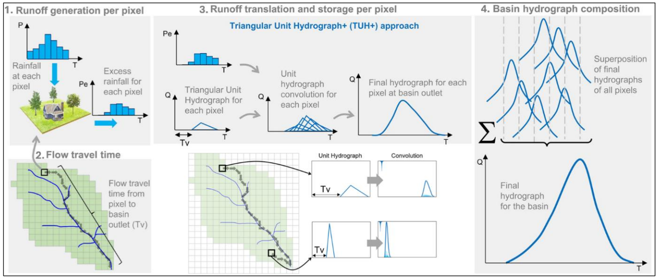
165 Figure 3. Schematic illustration of the Hidropixel model (based on Lima et al., 2024).
