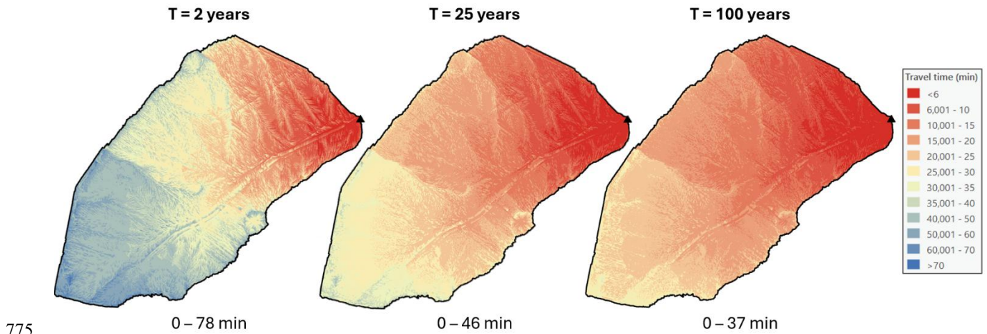
Figure 11. Spatial distribution of runoff travel times across the catchment under varying design storm magnitudes (2-year, 25-year, and 100-year return periods) adjusted according to Meyersohn's formula.
