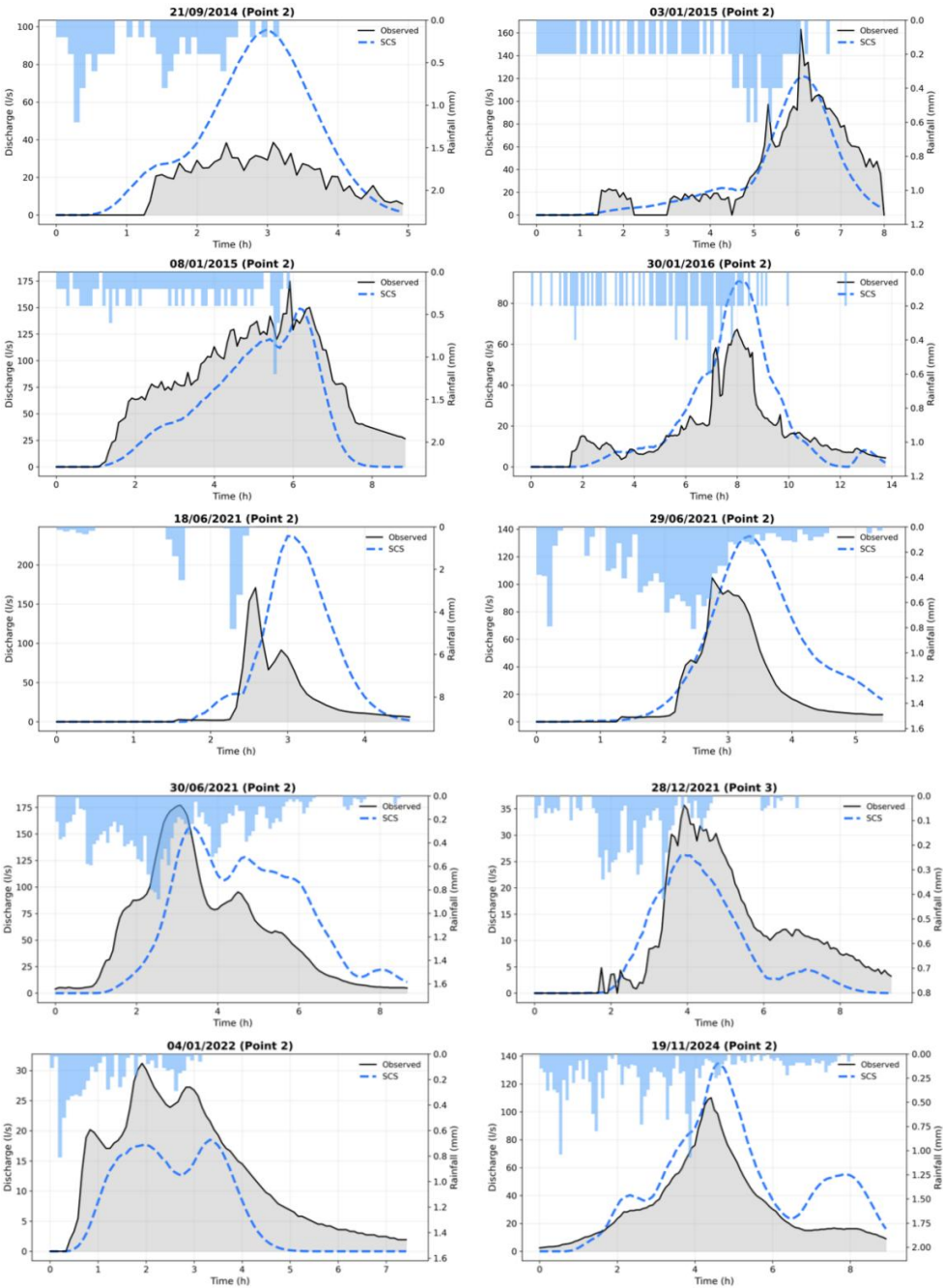
910 Figure E1. Comparison of observed and simulated hydrographs for a selection of distinct rainfall-runoff events recorded between 2014 and 2024.
