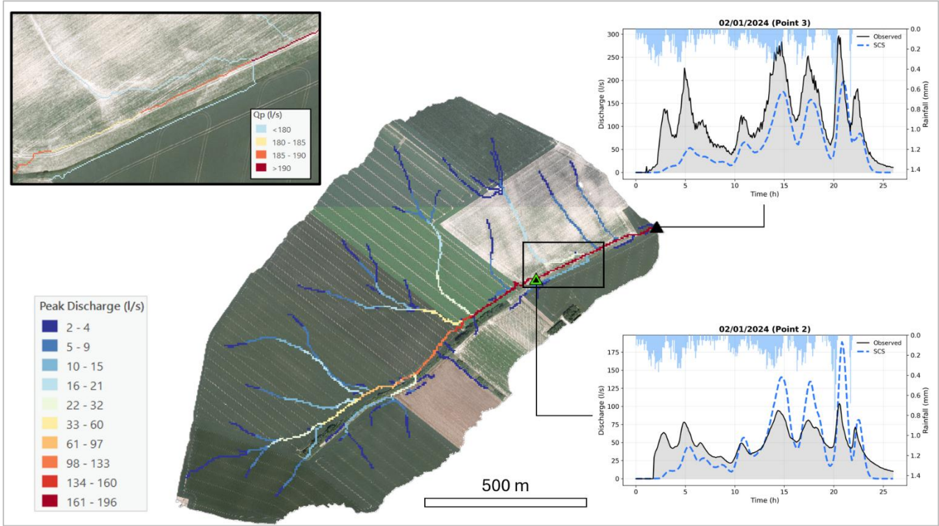
735 Figure 10. Spatial distribution of simulated Q_p using the SCS velocity method along the concentrated flow paths of the catchment during the 02/01/2024 rainfall event (duration: 18 h, total depth: 28 mm). The right panels display the corresponding hydrographs at the upstream (Point 2) and downstream (Point 3) monitoring stations, comparing observed discharge with the model outputs using both the SCS and SWRRB routing configurations. The zoomed area highlights the spatial variability of Q_p . Maps data: © Service public de Wallonie, 2018.
