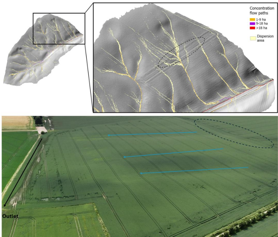
935 Figure F3. Top: spatial dispersion and mapped location of simulated flow paths. Bottom: aerial view of the northern hillslope of the Chastre catchment following the 29 May 2026 storm, highlighting the three main concentrated flow axes (blue) converging into the primary thalweg (black); flow paths within the dotted area exhibit a diffuse and mobile pattern.
