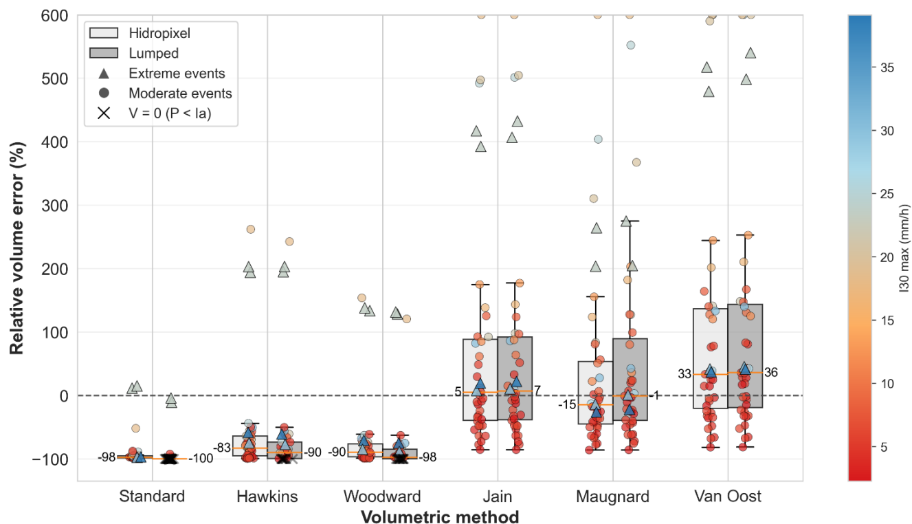
Figure D1. Comparative boxplots of signed relative volume error (%) for runoff events (n = 39) at the Chastre watershed using the Hidropixel model (light grey) and a lumped model approach (grey). Marker shapes distinguish event categories (circles for normal events, triangles for extreme events), while the colour gradient indicates the I30 max (the maximum intensity of rainfall recorded over a period of 30 minutes), and the black crosses highlight zero-runoff simulations ( P < I_a ). Numeric median values are displayed.
