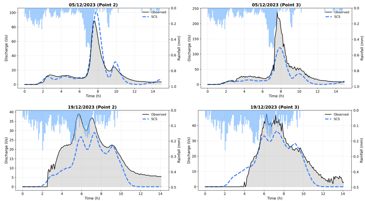
Figure D2-Figure E2. Simultaneous hydrograph restitution at the upstream (Point 2) and downstream (Point 3) monitoring stations for two rainfall events.
