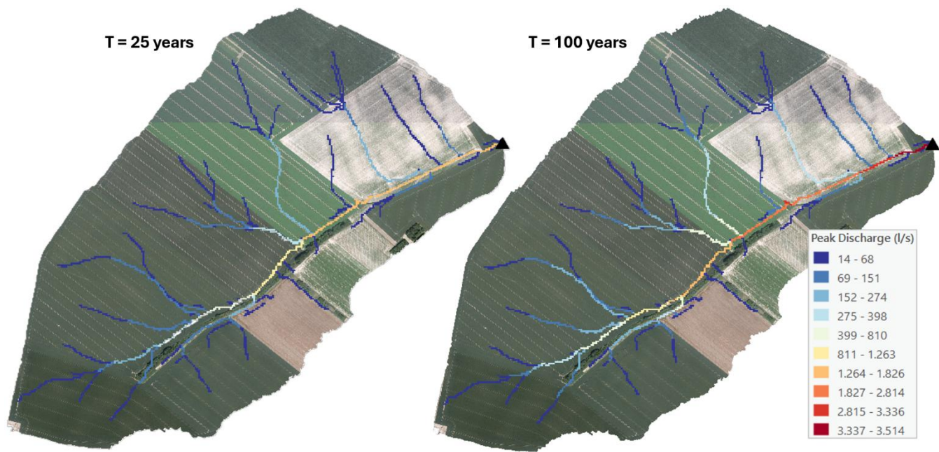
Figure 12. Spatial distribution of simulated peak flows Q_p along concentrated flow paths for the 25-year and 100-year design storms. Maps data: © Service public de Wallonie, 2018.
