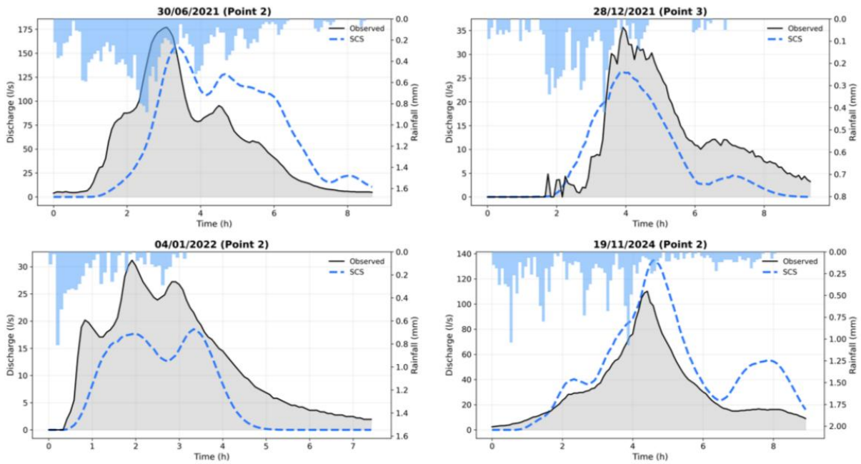
Figure D1-Figure E1. Comparison of observed and simulated hydrographs for a selection of distinct rainfall-runoff events recorded between 2014 and 2024.
