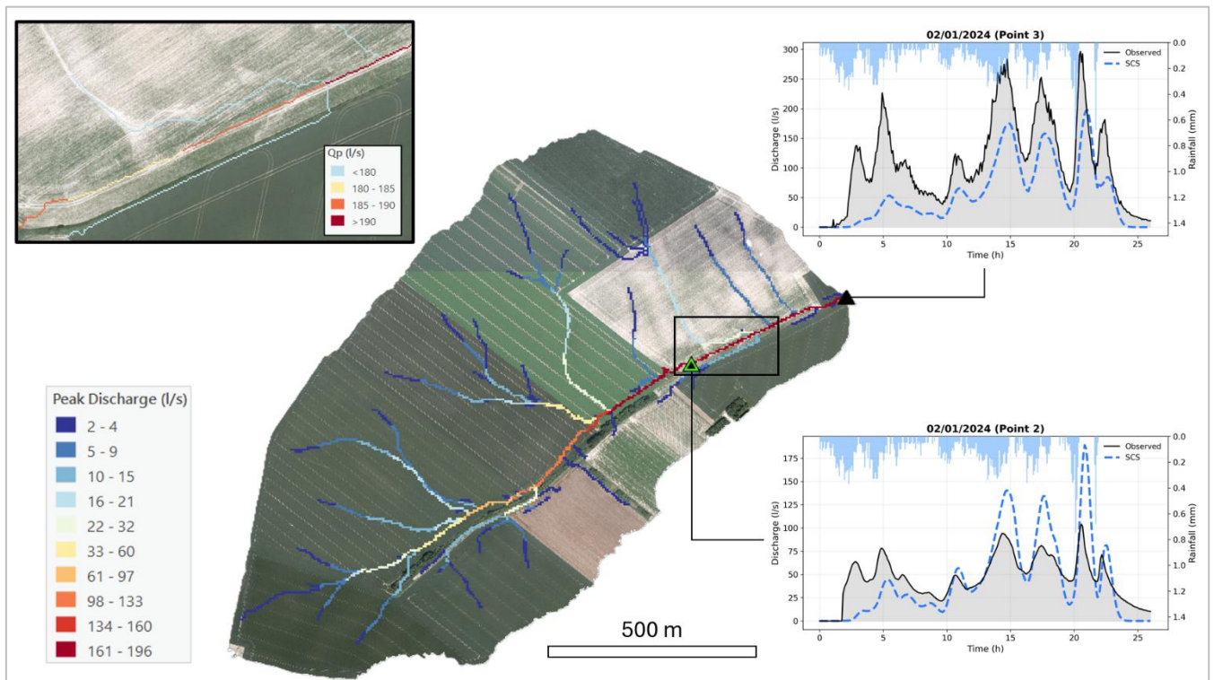
Figure 10. Spatial distribution of simulated peak-flow Q_p using the SCS velocity method along the concentrated flow paths of the catchment during the 02/01/2024 rainfall event (duration: 18 h, total depth: 28 mm). The right panels display the corresponding hydrographs at the upstream (Point 2) and downstream (Point 3) monitoring stations, comparing observed discharge with the model outputs using both the SCS and SWRRB routing configurations. The zoomed area highlights the spatial variability of Q_p . Maps data: © Service public de Wallonie, 2018.
