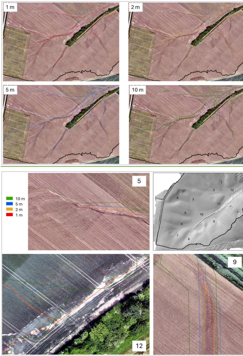
Figure F4. Simulated concentrated flow networks extracted at four spatial resolutions (1, 2, 5, and 10 m) based on the 2021–2022 DEM, with the location of 12 ephemeral gullies observed after the 29 May 2026 storm, mapped on the post-event DEM (captured 30 May 2026).
