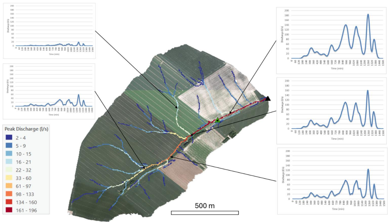
Figure F1. Spatio-temporal simulation of the 02/01/2024 runoff event using the Hidropixel SCS model. The central map displays peak discharges ( l\ s^{-1} ) along flow concentration paths, while the surrounding panels show simulated hydrographs at specific locations. The black triangle denotes the main outlet, and the green triangle indicates an upstream gauging station. Maps data: © Service public de Wallonie, 2018.
