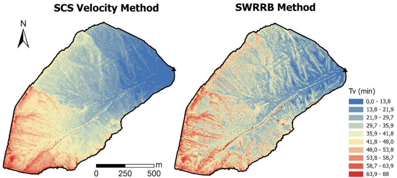
640 Figure 7. Spatial patterns of flow travel time ( T_v ) to the outlet calculated using the SCS velocity method (left) and the SWRRB method (right) for the year 2021 in the 111 ha basin (Point 3).
