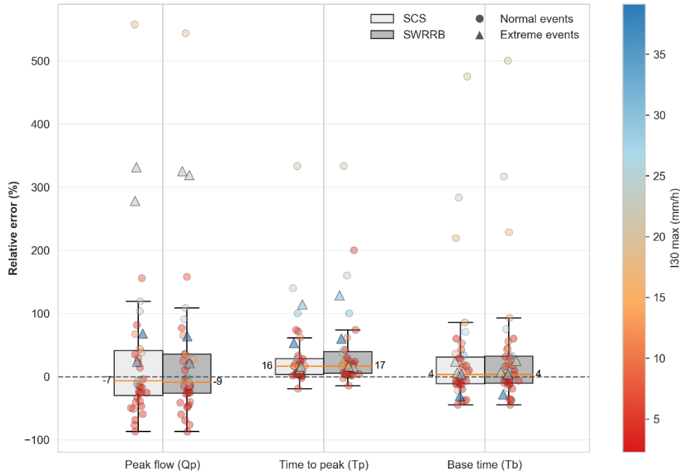
Figure 9. Relative errors (%) of hydrological flood indicators for events (based on Jain's method to estimate runoff volume). The boxes compare Hidropixel SCS and SWRRB for peak flowpeak discharge ( Q_p ), peak timetime to peak ( T_p ), and base time ( T_b ). Marker shapes distinguish event categories (circles for normal events, triangles for extreme events), while the colour gradient indicates the maximum 30-minute rainfall intensity. Median values are indicated on each boxplot.
