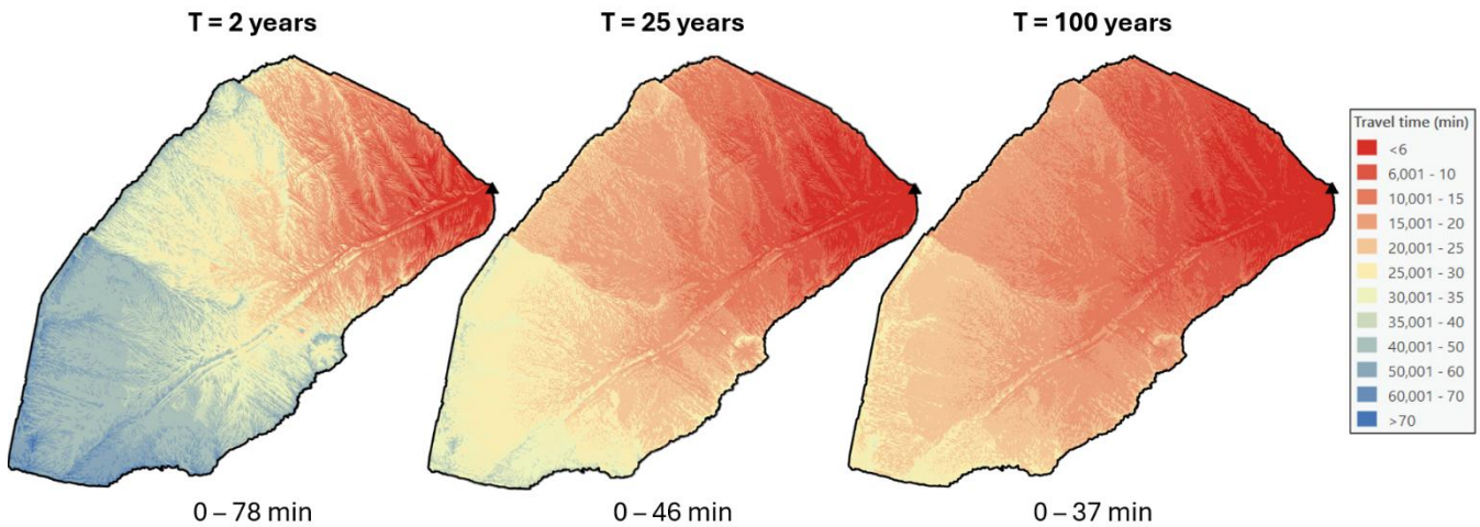
Figure 11. Spatial distribution of runoff travel times across the catchment under varying design storm magnitudes (2-year, 25-year, and 100-year return periods) adjusted according to Meyersohn's formula.
