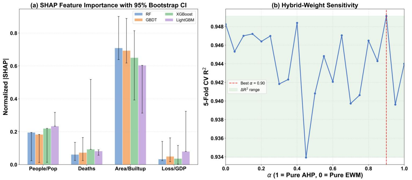
Figure 4: Recommended presentation: (a) normalized out-of-fold SHAP contributions with bootstrap intervals; (b) hybrid-weight sensitivity across \alpha
