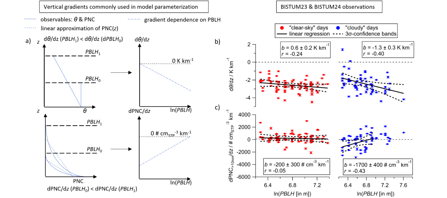
Figure 2: (a) Schematic description of the dependency of atmospheric stability (reflected by \theta(z) , with the altitude z ) and a pollutant with source at ground level ( PNC(z) ) on altitude for the well-mixed planetary boundary layer with a height PBLH_i as commonly used in model parameterizations (a, left). Deriving the dependence of d\theta/dz and dPNC/dz from PBLH results in a linear-logarithmic dependency of respective gradients on the boundary layer height (a, right). Experimental data of gradients of the potential temperature \theta (b) and the particle number concentration PNC_{>10 \text{ nm}} (c) in the lowermost 500 m in a mixed PBL from both campaigns are plotted versus associated logarithms of respective planetary boundary layer heights (PBLH, in m). Linear regression with the slope b and its 3\sigma -confidence bands are depicted in solid and dotted lines.
