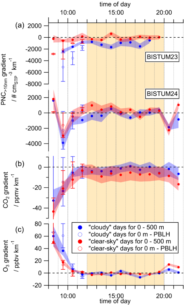
Figure 4: Average hourly-resolved gradients of PNC >10 nm (a), CO 2 (b) and O 3 (c) in the lowermost 500 m above ground show a diurnal variation for “clear-sky” (red) and “cloudy” days (blue). Open markers represent gradients and ratios calculated for measurements solely within the PBLH, when PBLH was lower than 500 m. The yellow shading represents hours with the PBLH being higher than 500 m. Propagated uncertainty bars (1σ) are presented as shaded areas.
