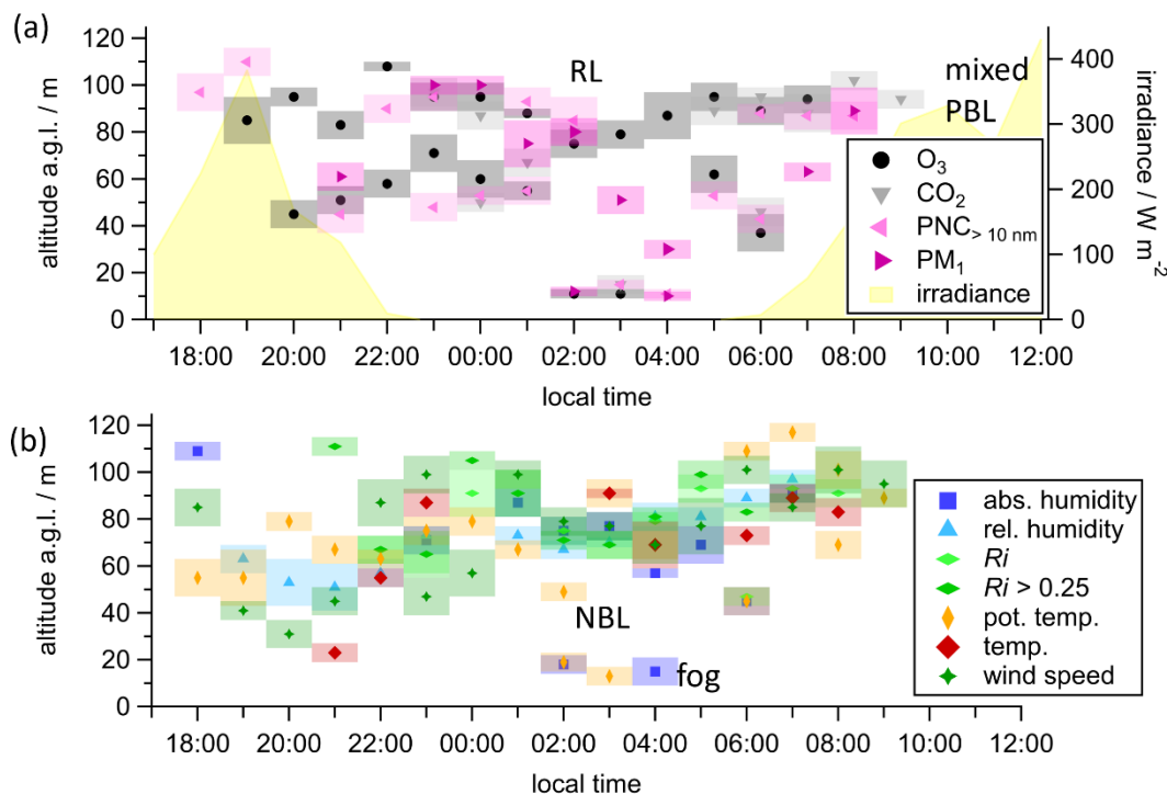
Figure 1: Estimated boundary layer heights (solid markers, with uncertainty ranges depicted as shaded areas) during the night of June 20 to 21, 2024. The boundary layer heights were derived from strongest gradient changes of the respective trace matter variables (a) and meteorological variables (b) and when the criterion Ri > 0.25 was fulfilled. The yellow shaded area in (a) represents the measured irradiance, which was reduced by cloudiness in the afternoon and the late morning.
