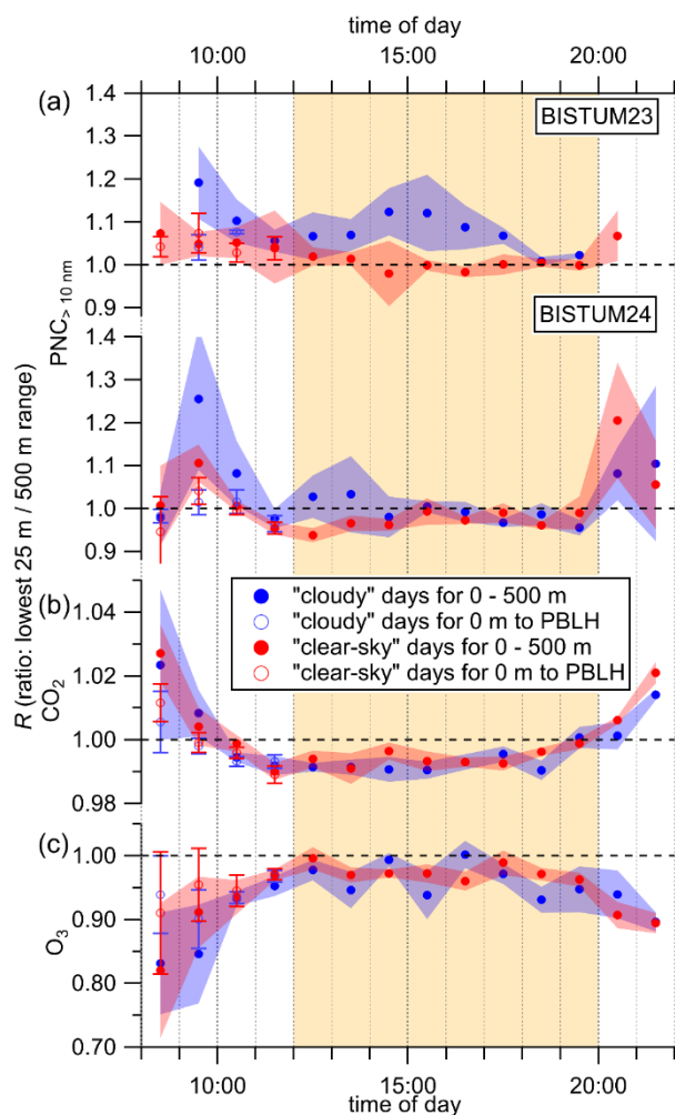
Figure 5: A diurnal variation the representativity R of \text{PNC}_{>10 \text{ nm}} (a), \text{CO}_2 (b) and \text{O}_3 (c) of ground-based measurements for the 500 m-column above. Open markers represent ratios calculated for measurements solely within the PBLH, when PBLH was lower than 500 m. The yellow shading represents hours with the PBLH being higher than 500 m. Propagated uncertainty for data points derived from the whole 500 m and from ground to the PBLH are represented as shaded areas and error bars as 1\sigma -uncertainties, respectively.
