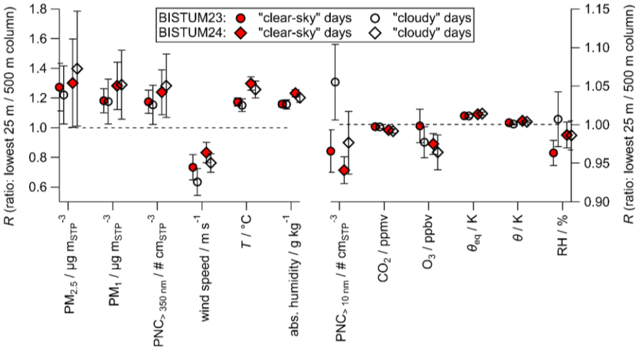
Figure 7: Representativity R (ratio of lowest 25 m/500 m column averages) of ground-based measurements with regard to the lowermost 500 m in a mixed PBL for meteorological and trace matter variables for two campaigns (circles and diamonds) for “clear-sky” and “cloudy” days (red and white filled markers, respectively). The x-axis is split to enhance visibility of variables with better representativity (note the different scaling of the y-axes). Error bars represent the overall uncertainty, mainly due to day-to-day variability.
