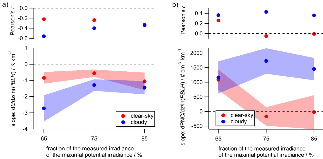
Figure 3: Influence of the irradiance threshold as a criterion to separate “clear-sky” (red) and “cloudy” days (blue) on the dependency of d\theta/dz and dPNC_{>10 \text{ nm}}/dz on the PBLH (in m). Pearson’s correlation coefficient r and slopes of the respective gradients versus the logarithm of the PBLH are depicted with 1 \sigma -confidence bands. The classification criteria are the ratios of the measured irradiance in respect to the maximal potential irradiance.
