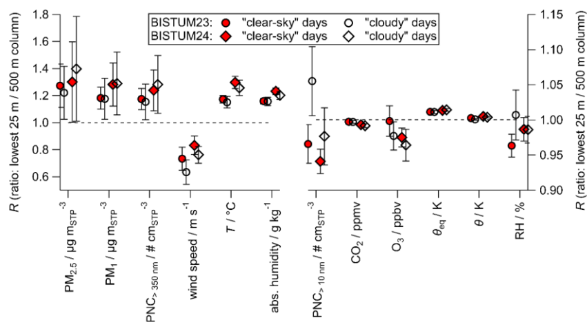
Figure 67: Representativity R (ratio of lowest 25 m/500 m column averages) of ground-based measurements with regard to the lowermost 500 m in a mixed PBL for meteorological and trace matter variables for two campaigns (circles and diamonds) for “clear-sky” and “cloudy” days (red and white filled markers, respectively). The x-axis is split to enhance visibility of variables with better representativity (note the different scaling of the y-axes). Error bars represent the overall uncertainty, mainly due to day-to-day variability.
