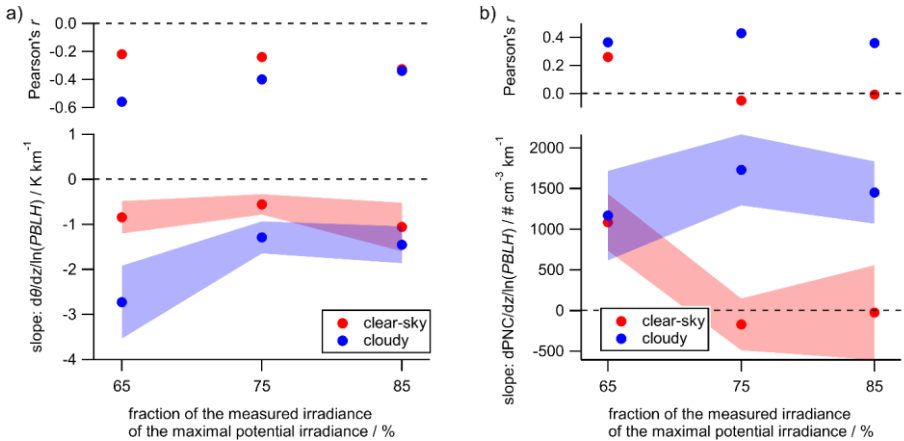
Figure 3: Influence of the irradiance threshold as a criterion to separate “clear-sky” (red) and “cloudy” days (blue) on the dependency of d\theta/dz and dPNC_{>10\text{ nm}}/dz on the PBLH (in m). Pearson’s correlation coefficient r and slopes of the respective gradients versus the logarithm of the PBLH are depicted with 1\sigma -confidence bands. The classification criteria are the ratios of the measured irradiance in respect to the maximal potential irradiance.
